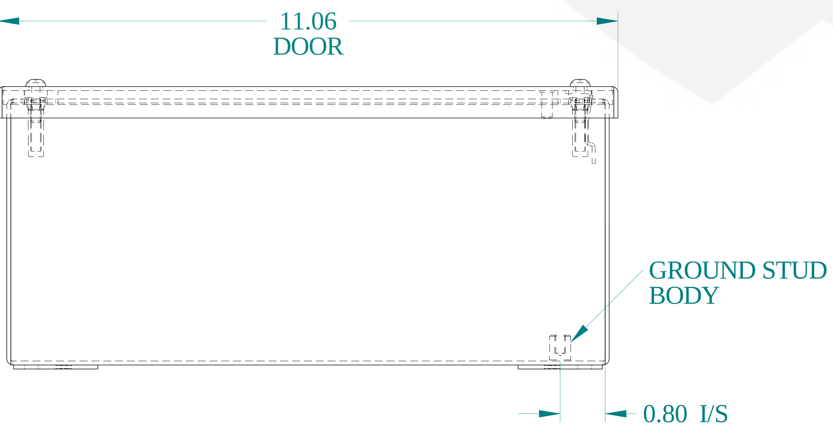
BOTTOM VIEW
