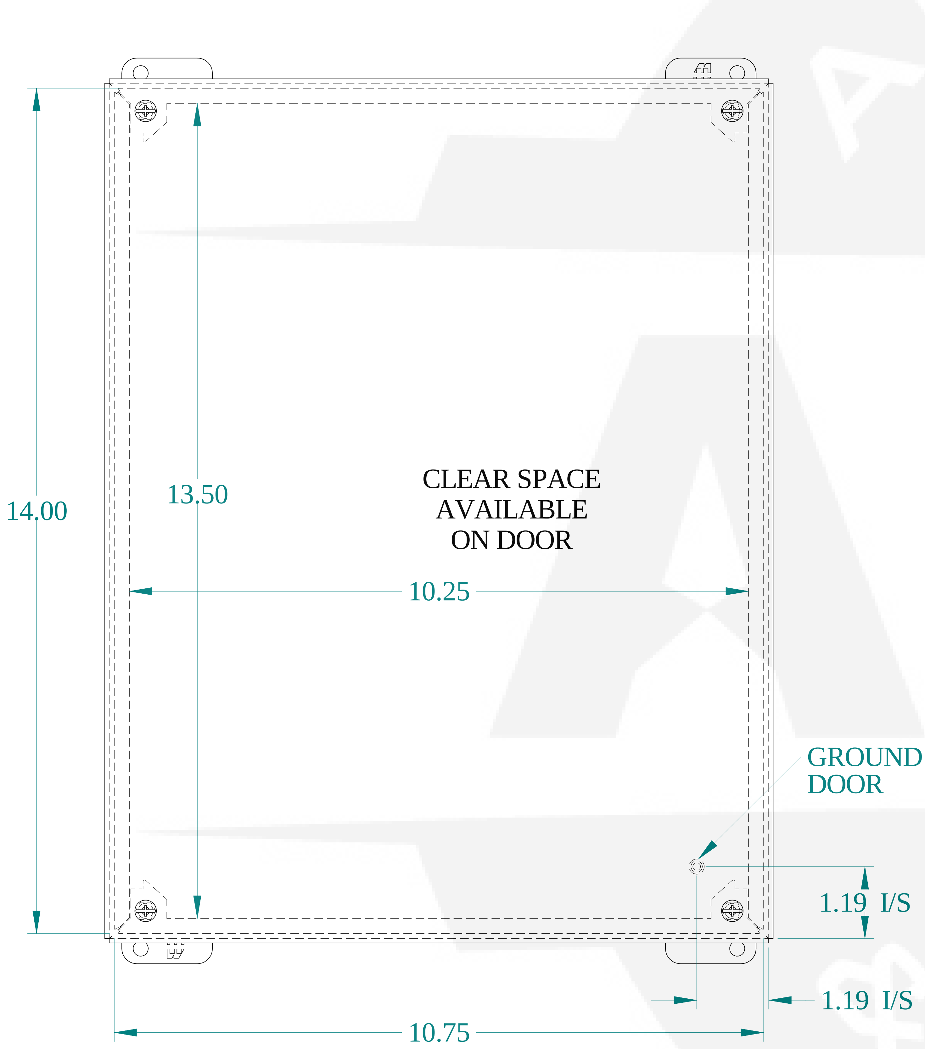
FRONT VIEW
