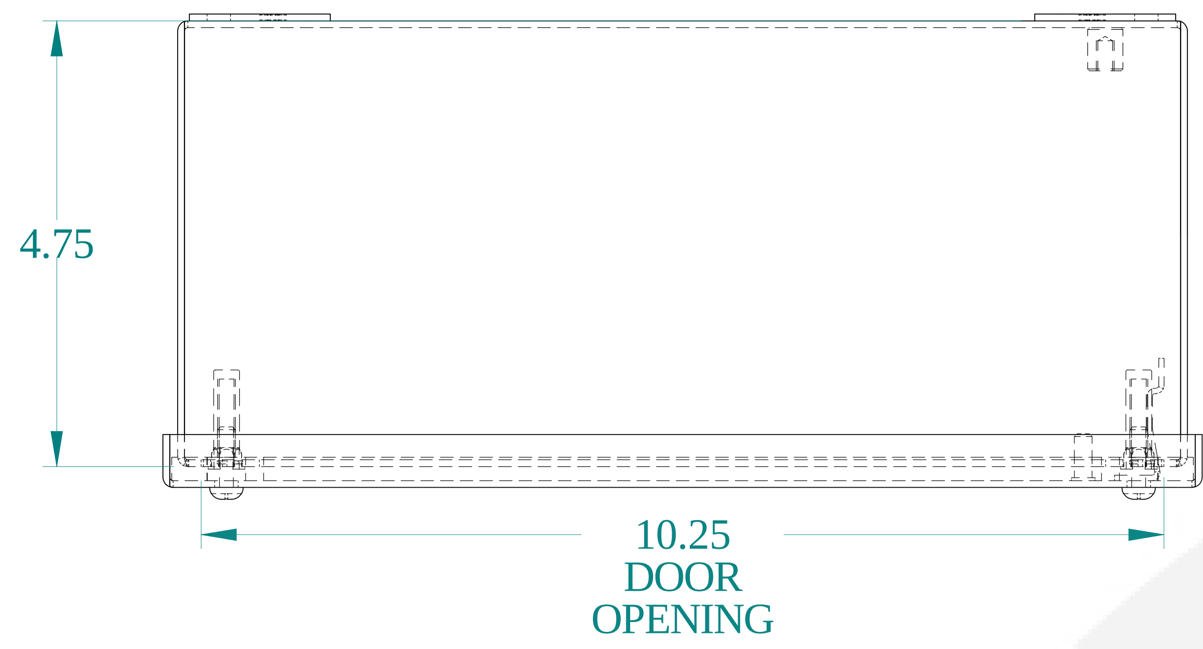
TOP VIEW
