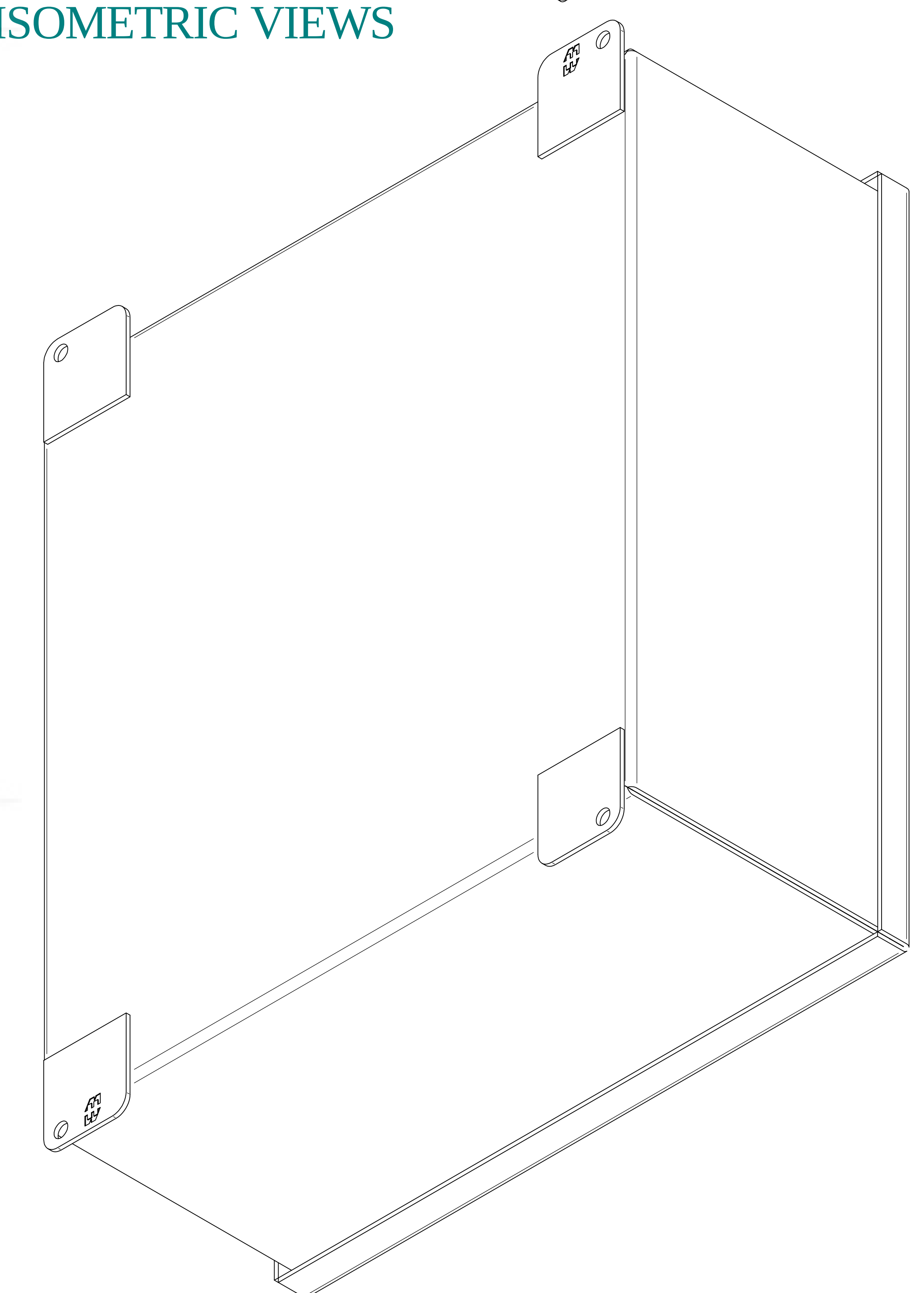
ISOMETRIC VIEWS
