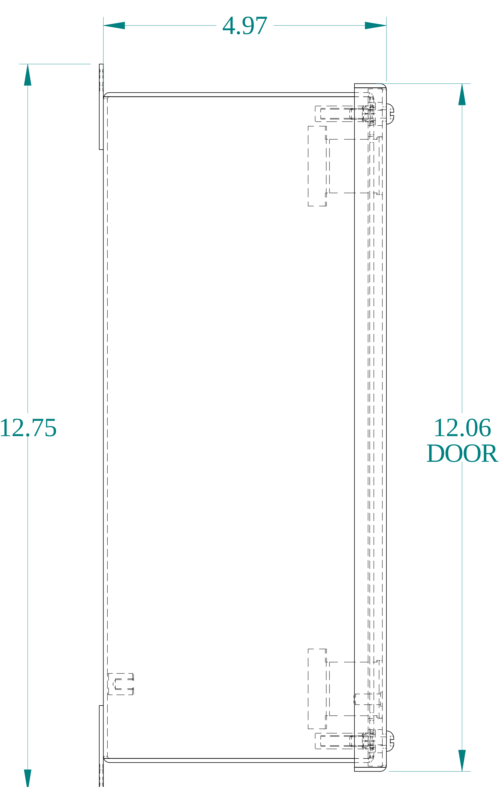
SIDE VIEW
