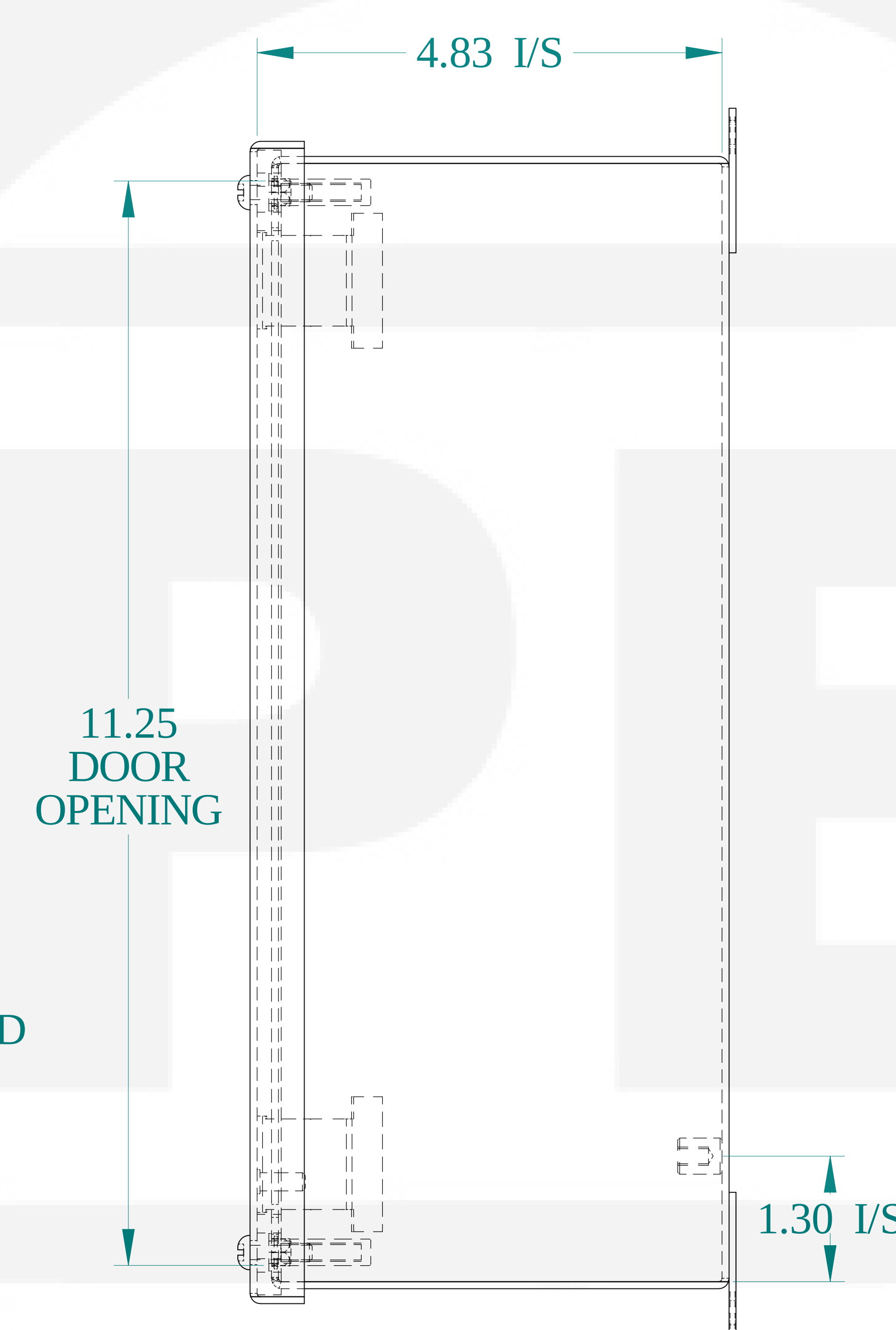
SIDE VIEW
