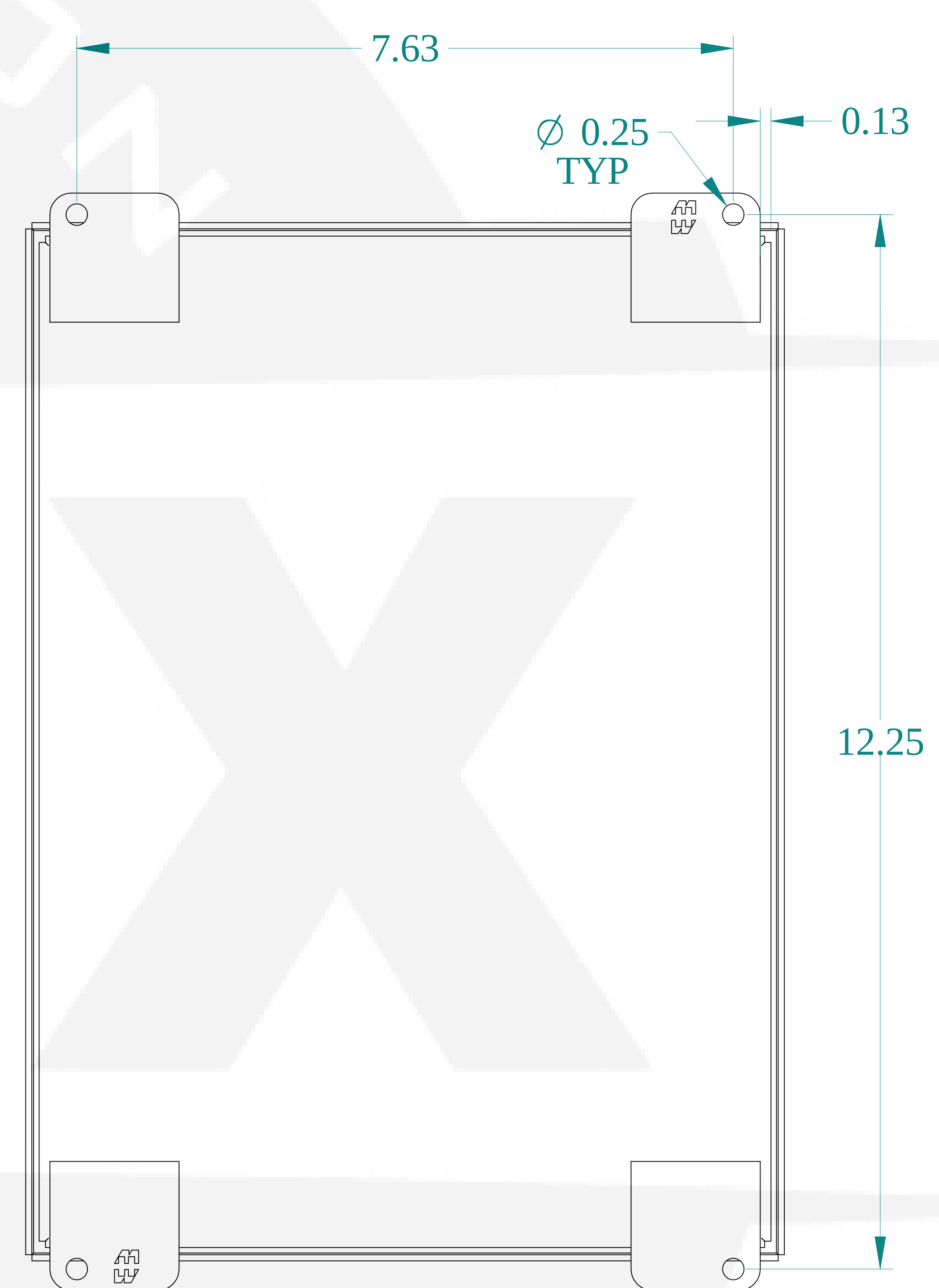
BACK VIEW
