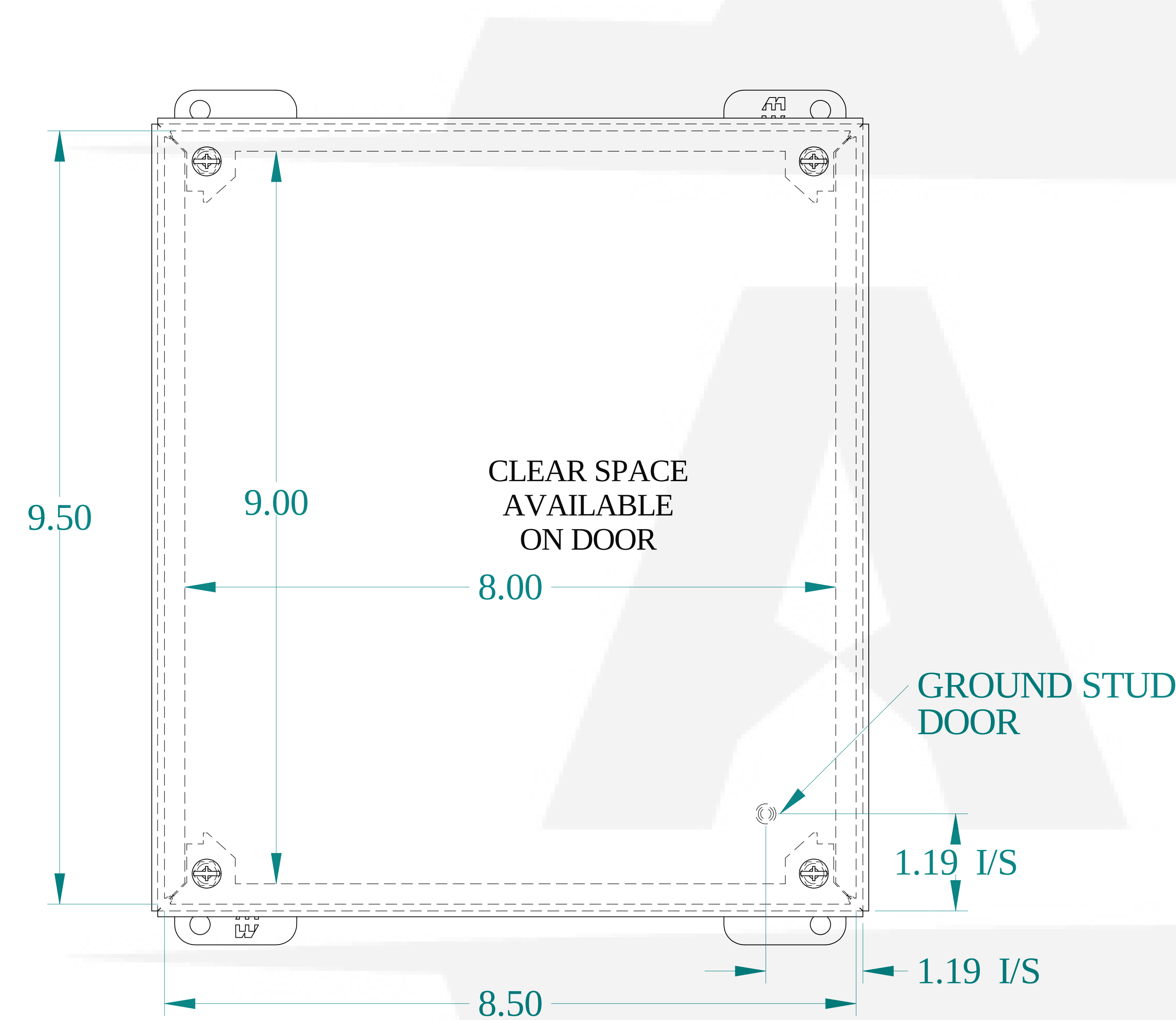
FRONT VIEW
