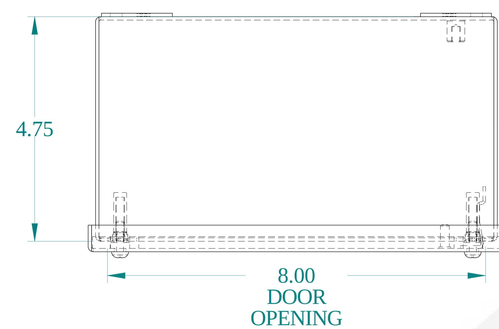
TOP VIEW
