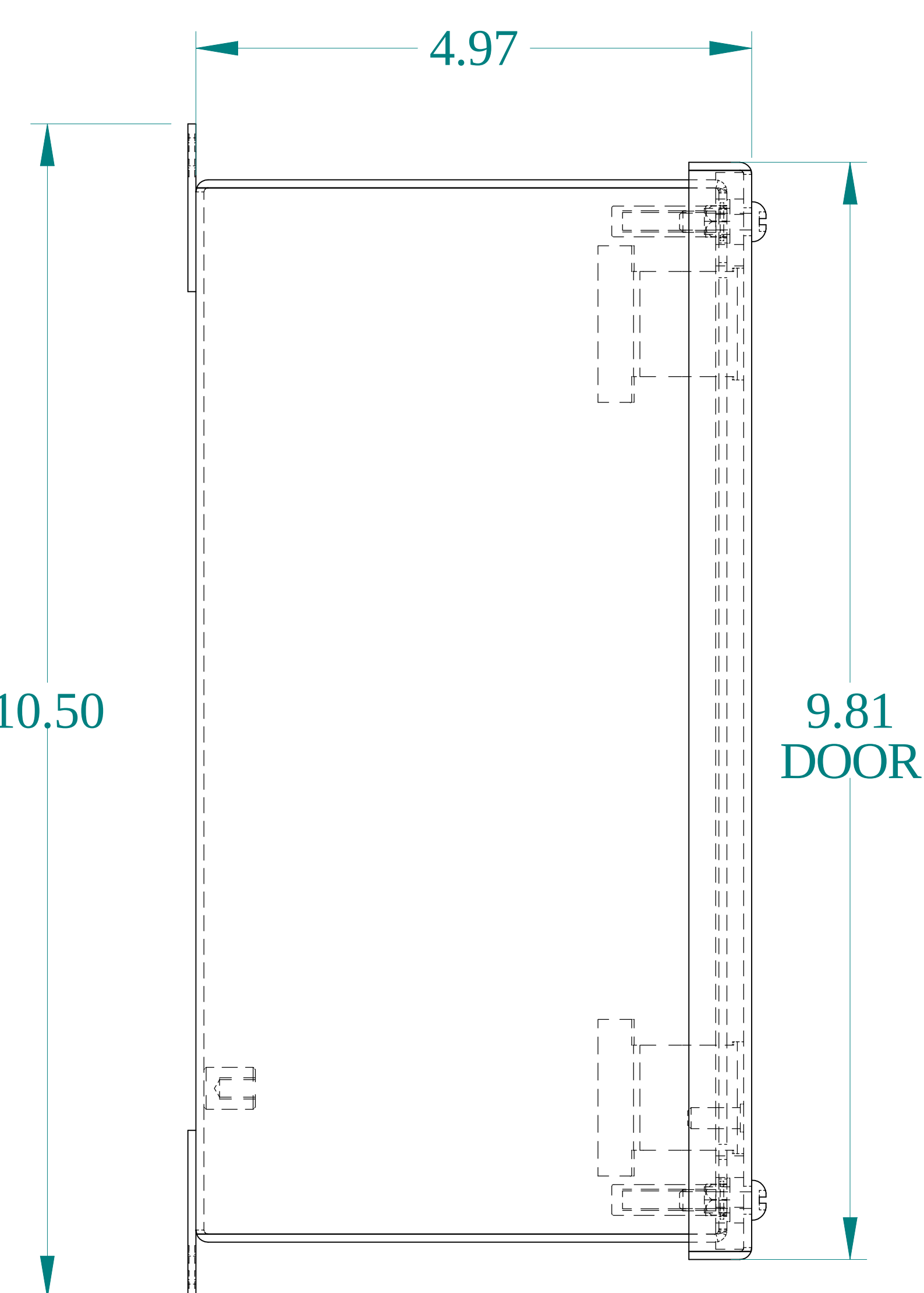
SIDE VIEW
