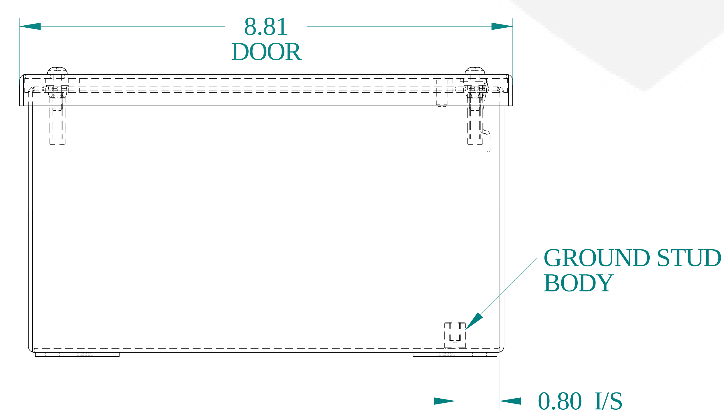
BOTTOM VIEW
