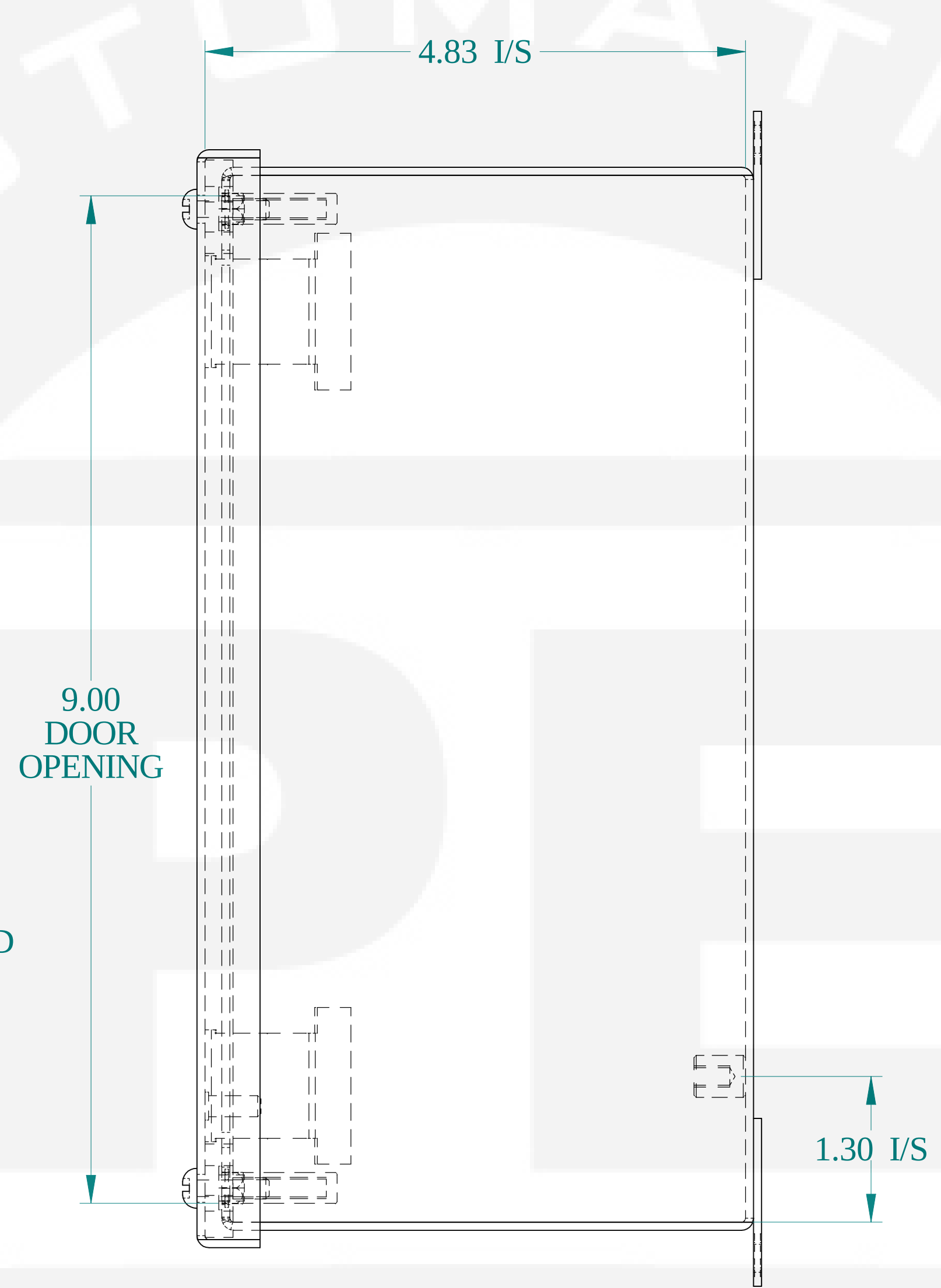
SIDE VIEW
