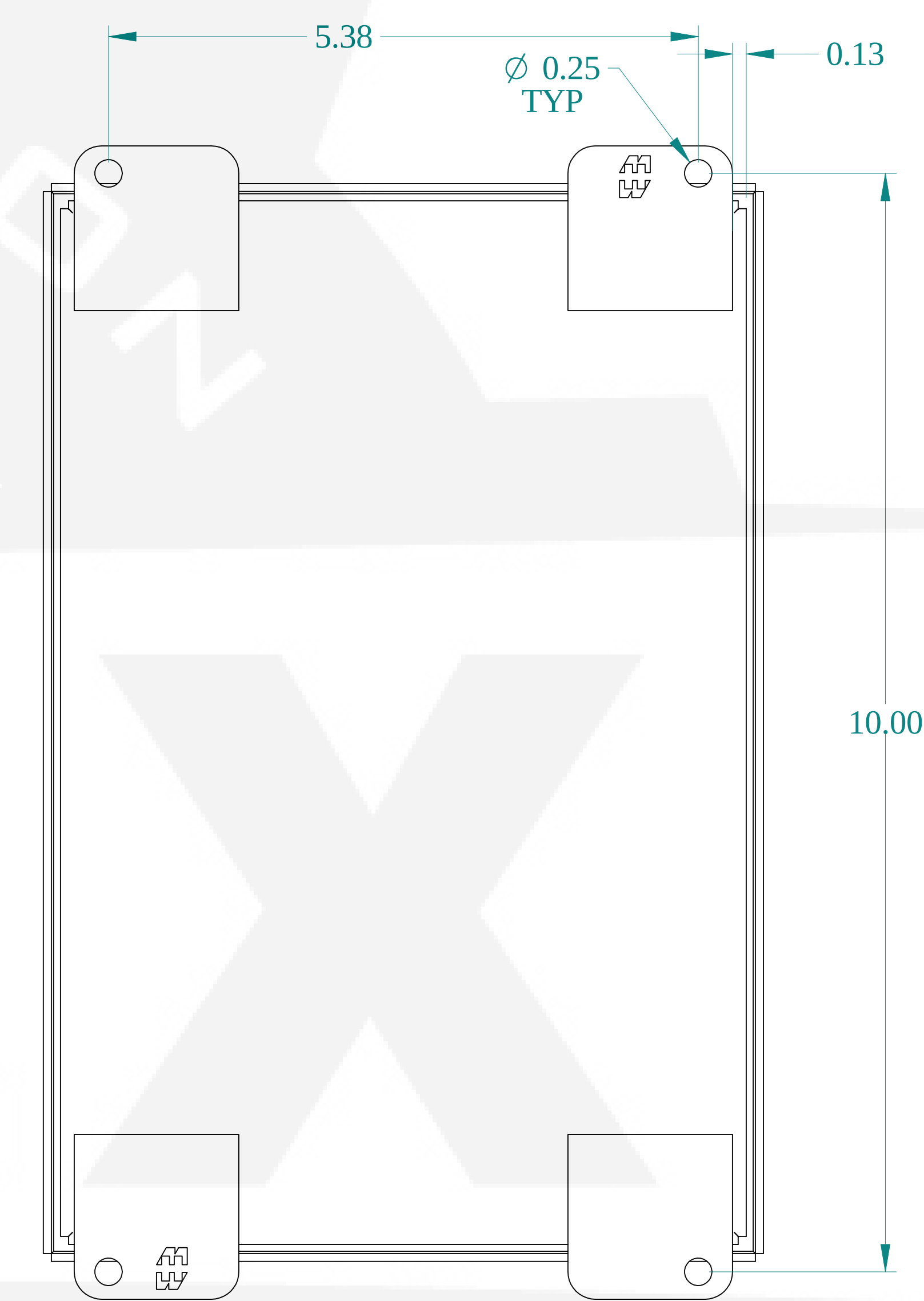
BACK VIEW
