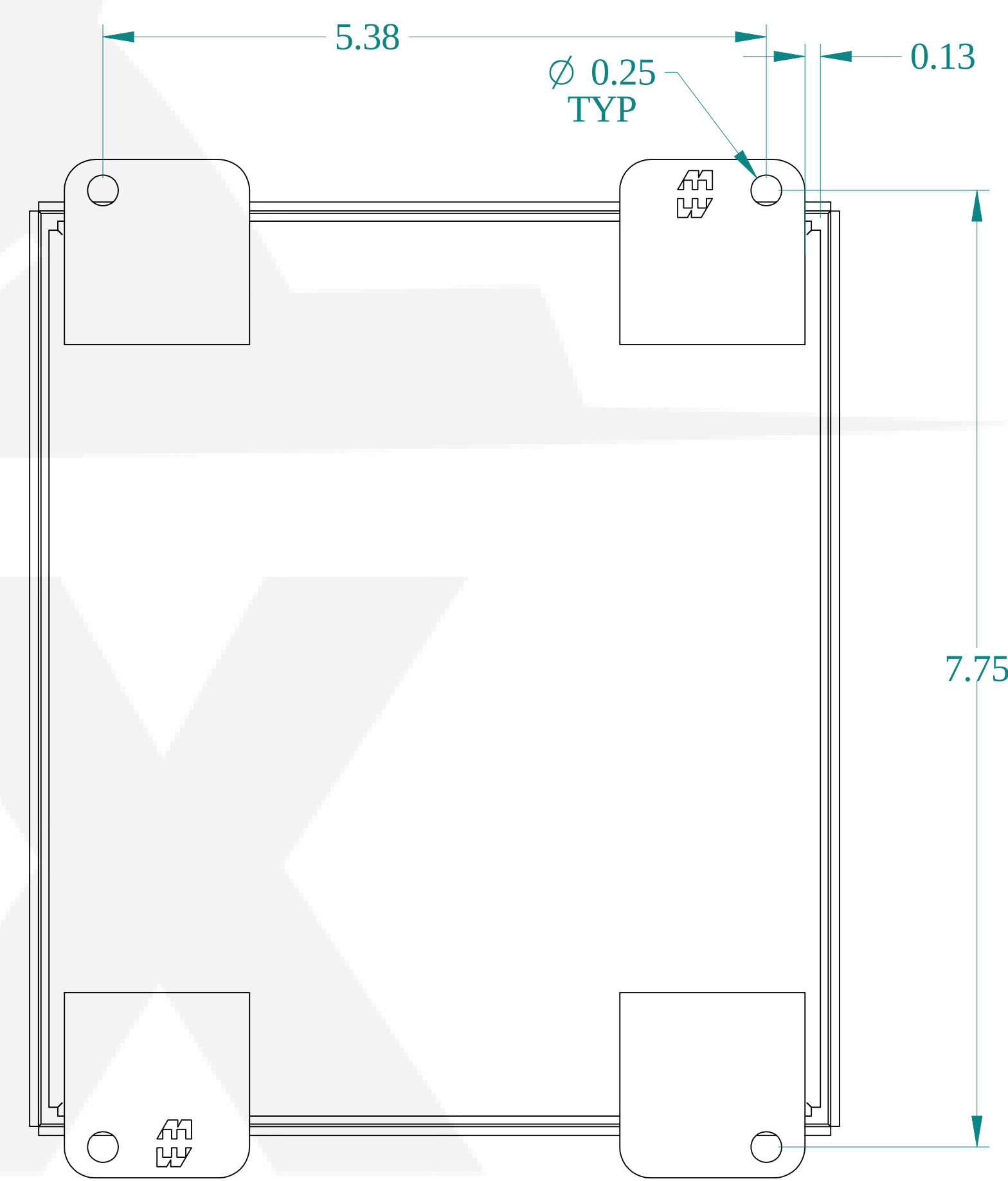
BACK VIEW
