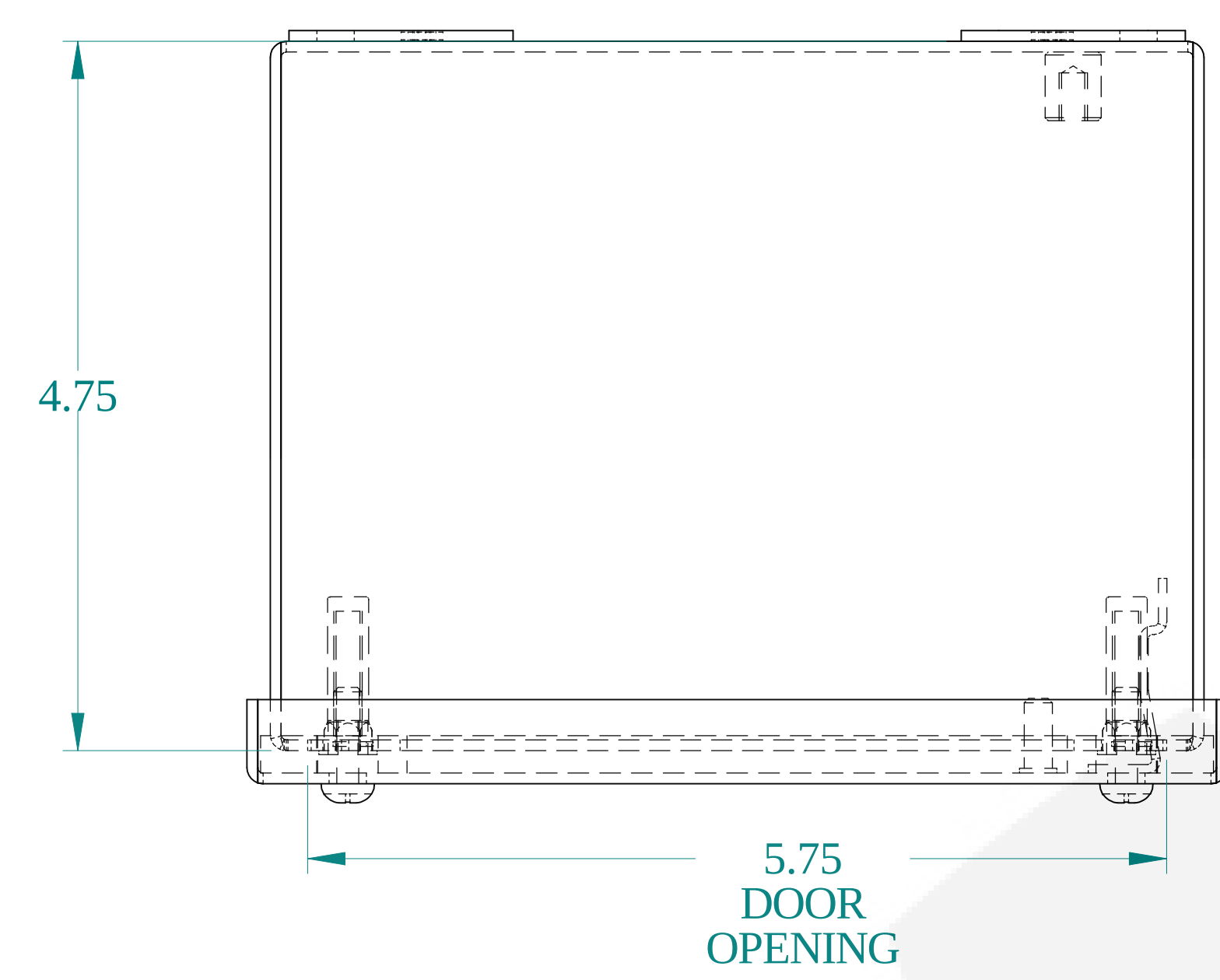
TOP VIEW
