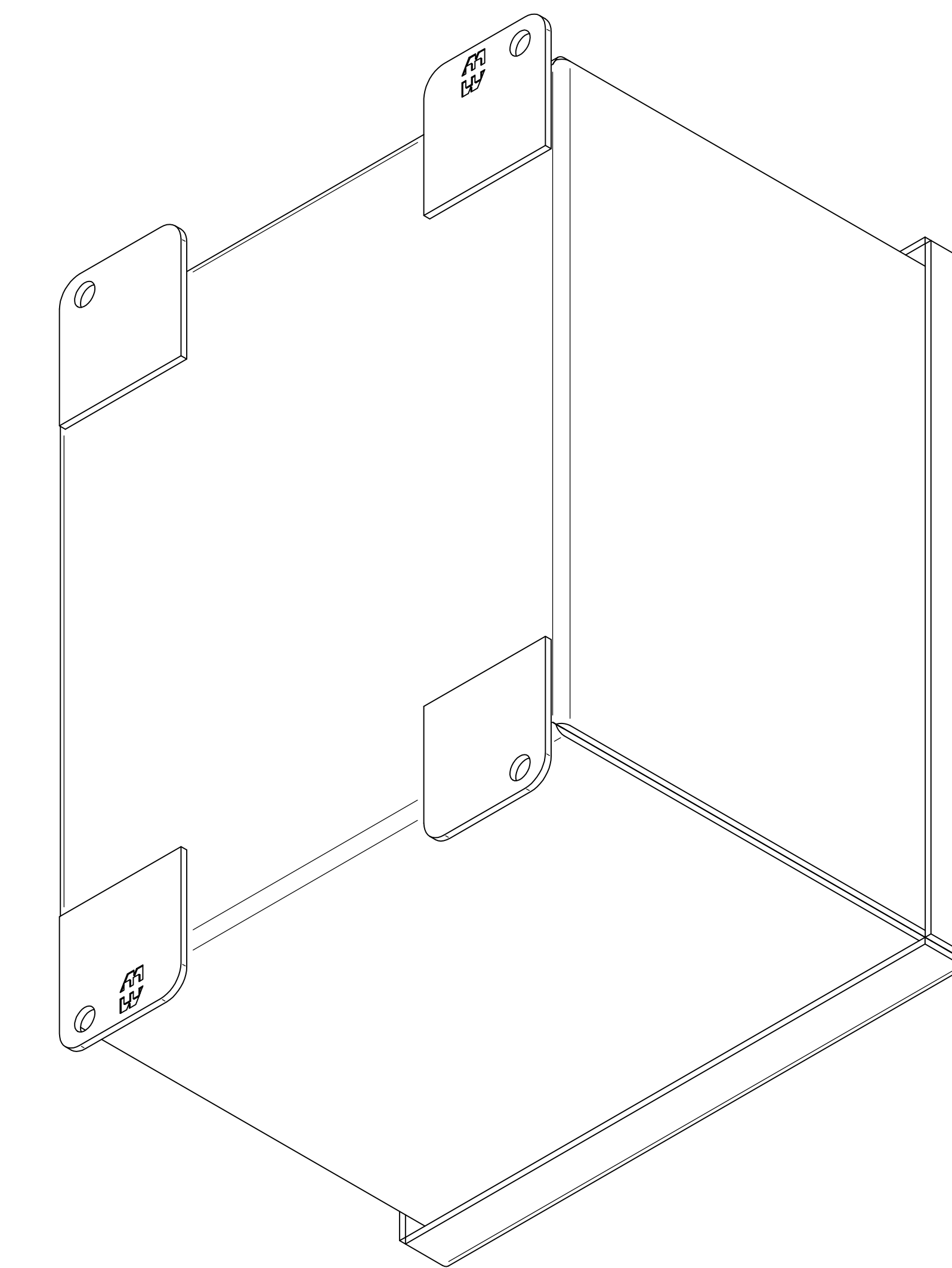
ISOMETRIC VIEWS
