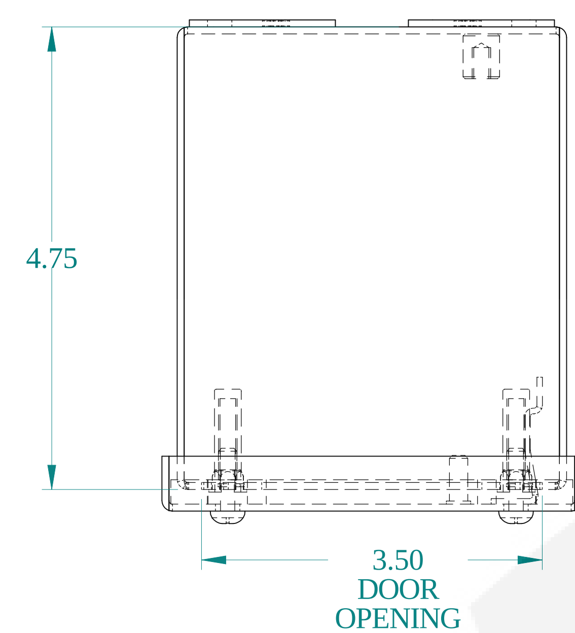
TOP VIEW
