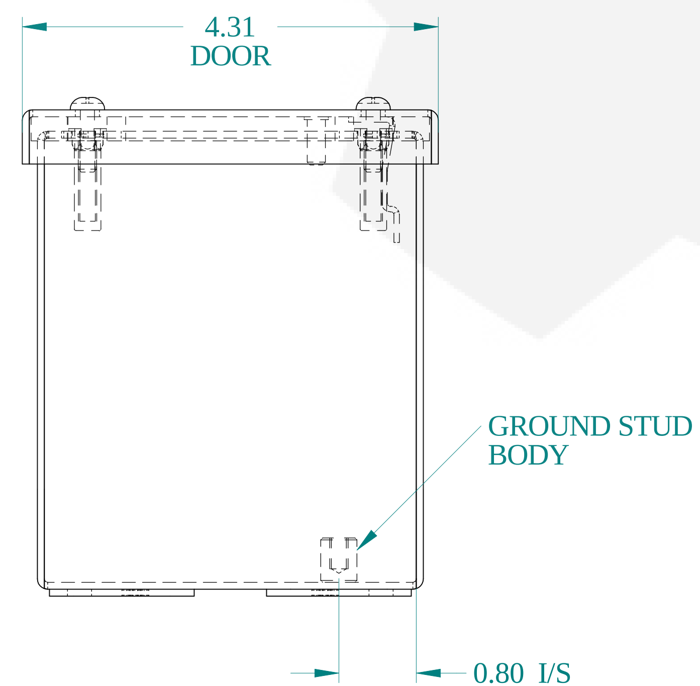
BOTTOM VIEW
