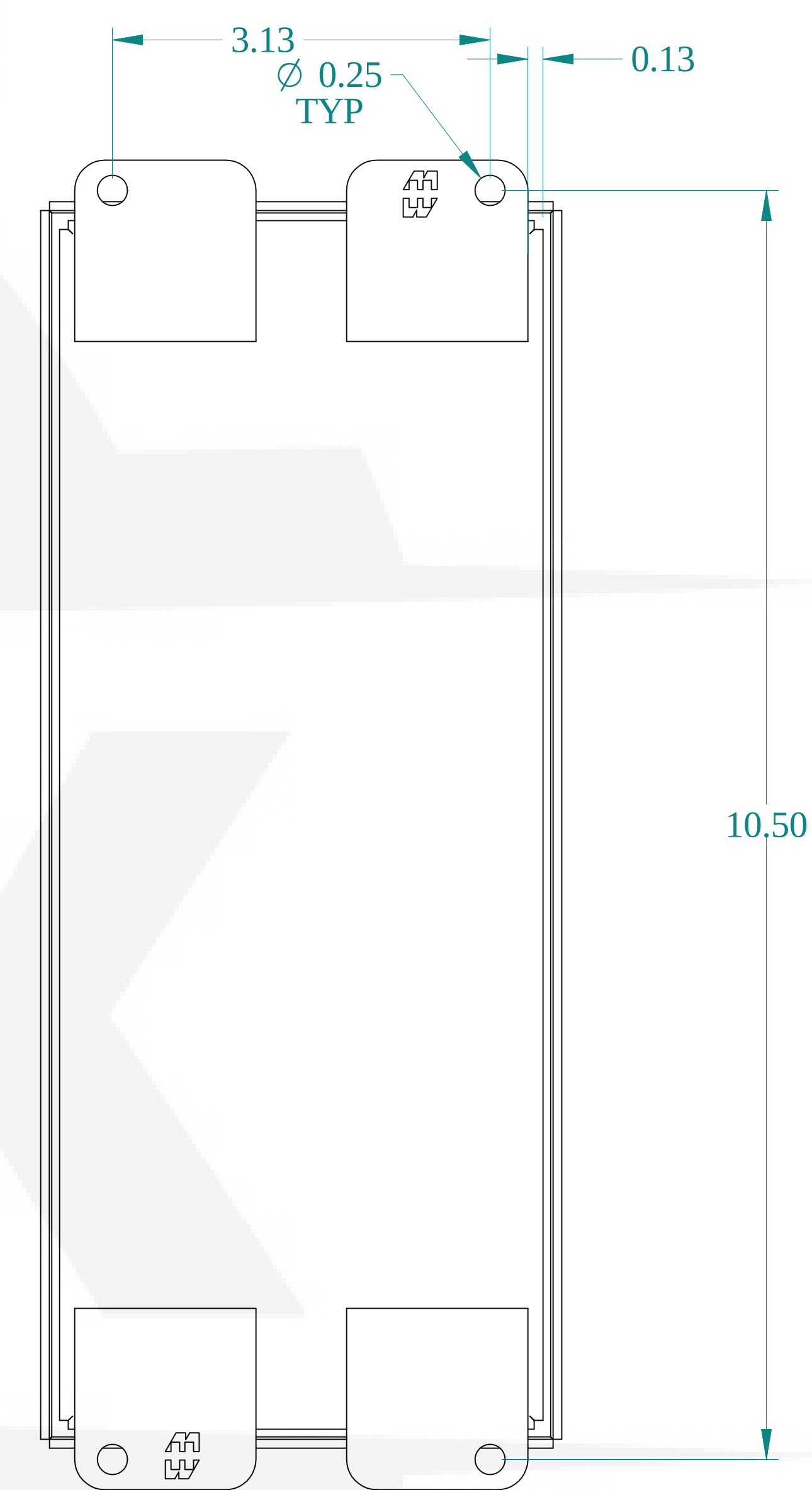
BACK VIEW
