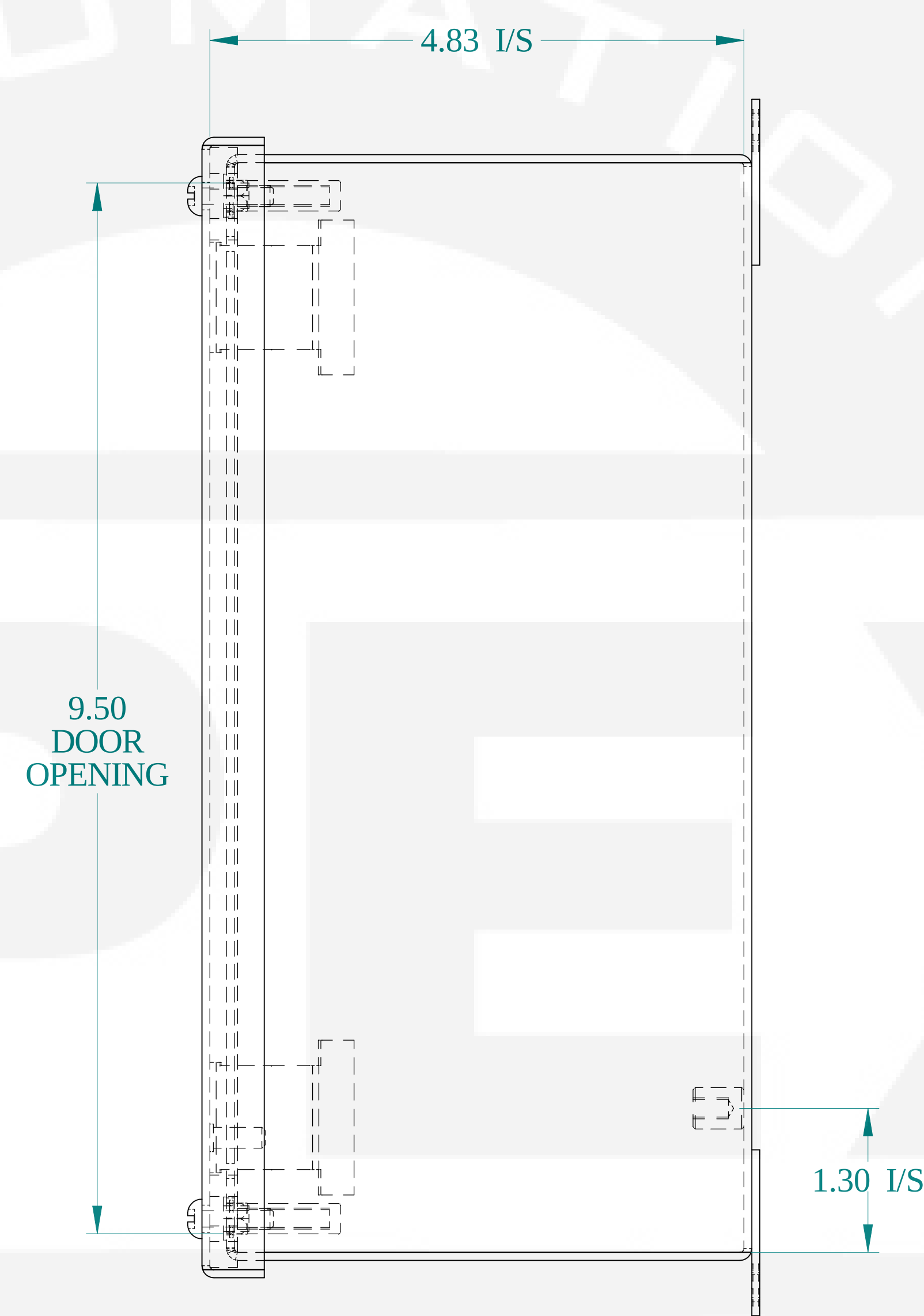
SIDE VIEW
