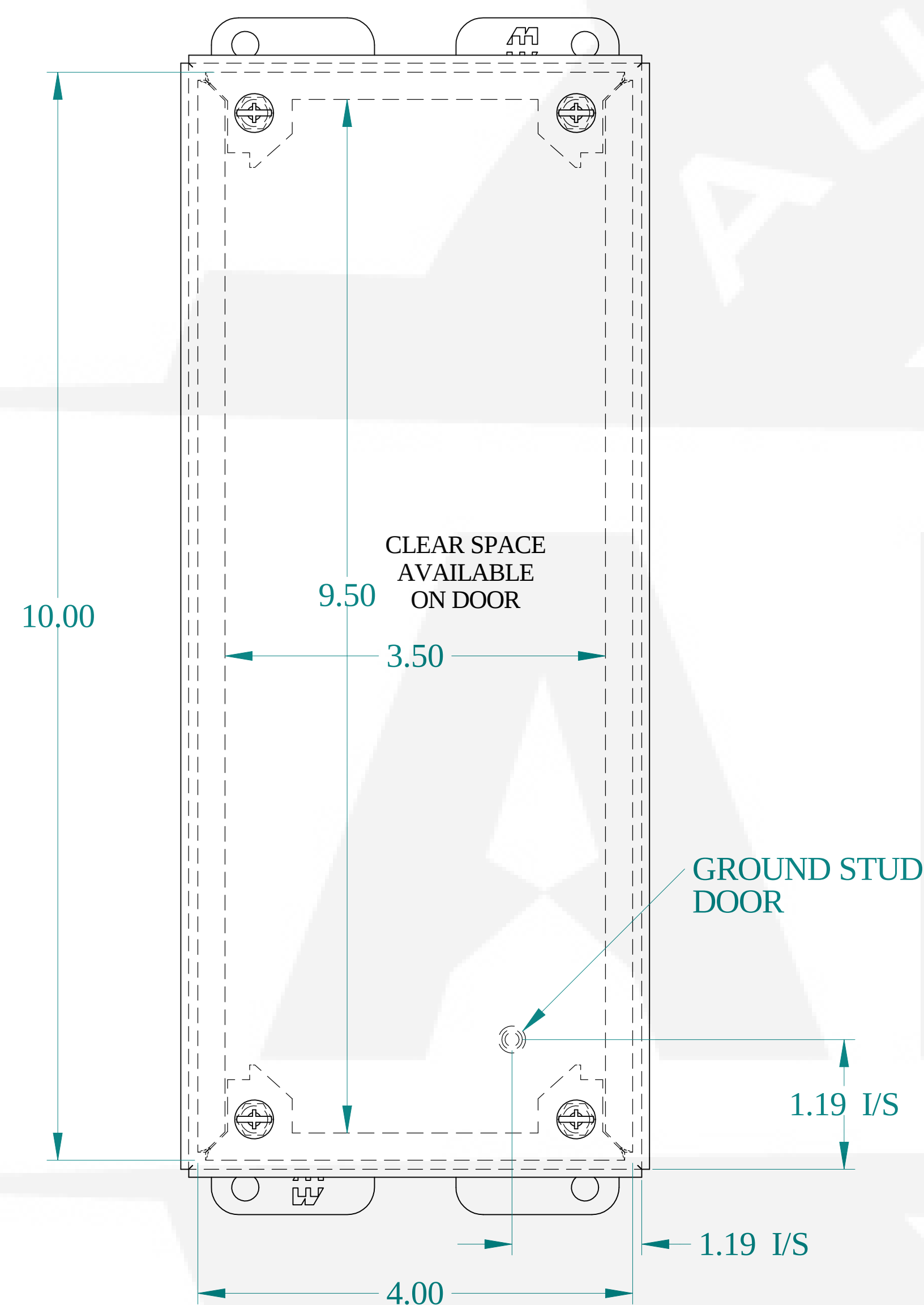
FRONT VIEW
