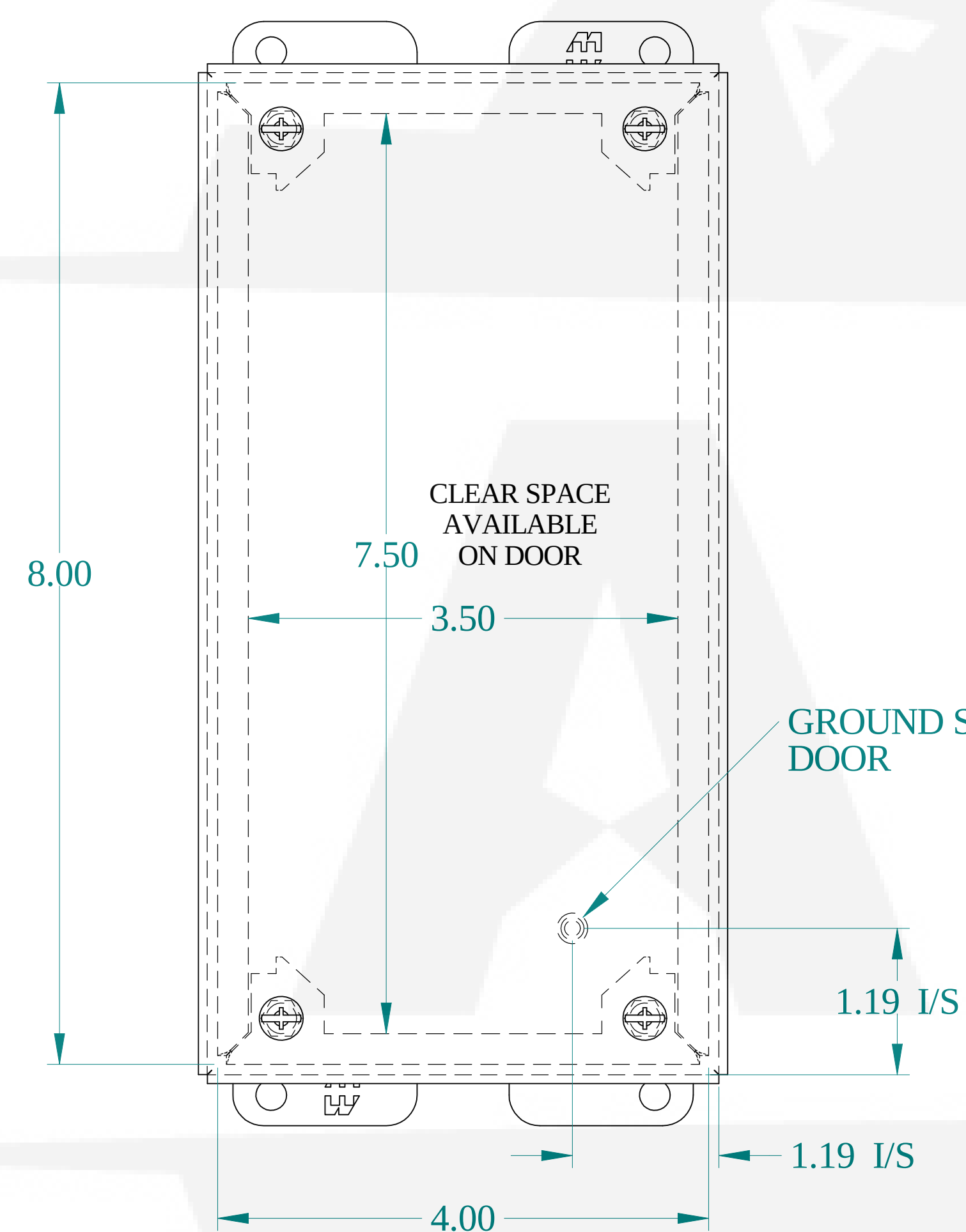
FRONT VIEW
