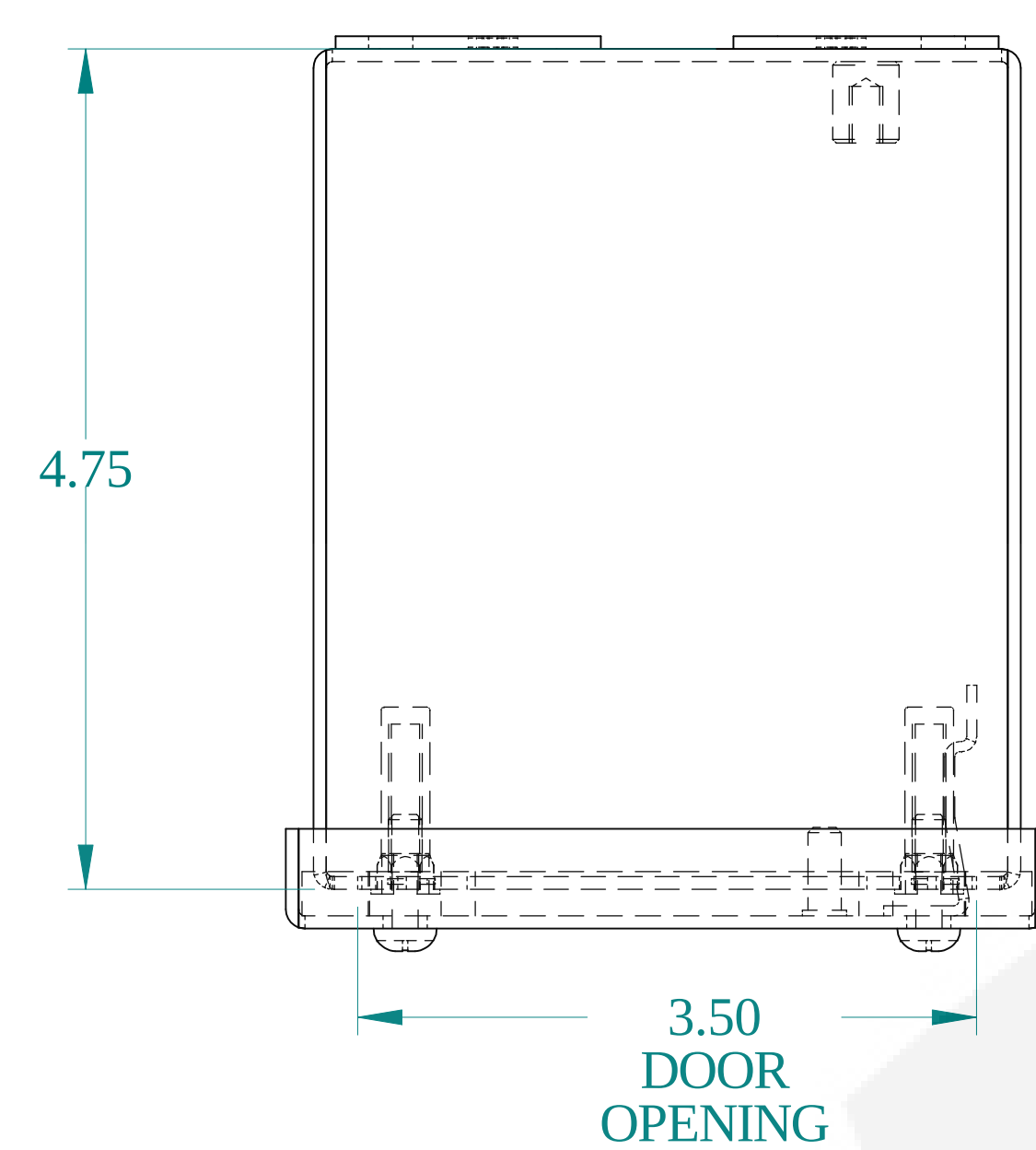
TOP VIEW
