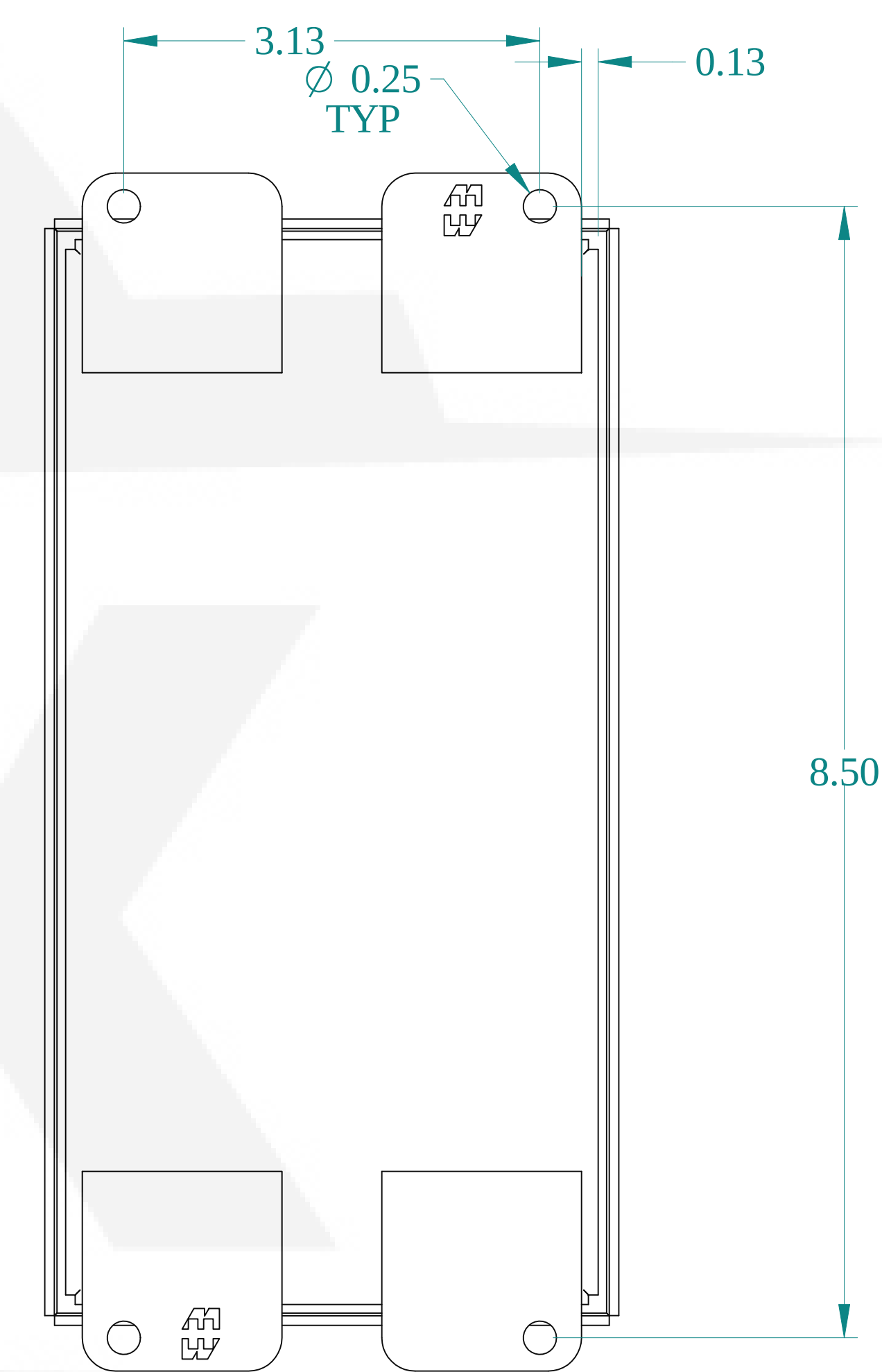
BACK VIEW
