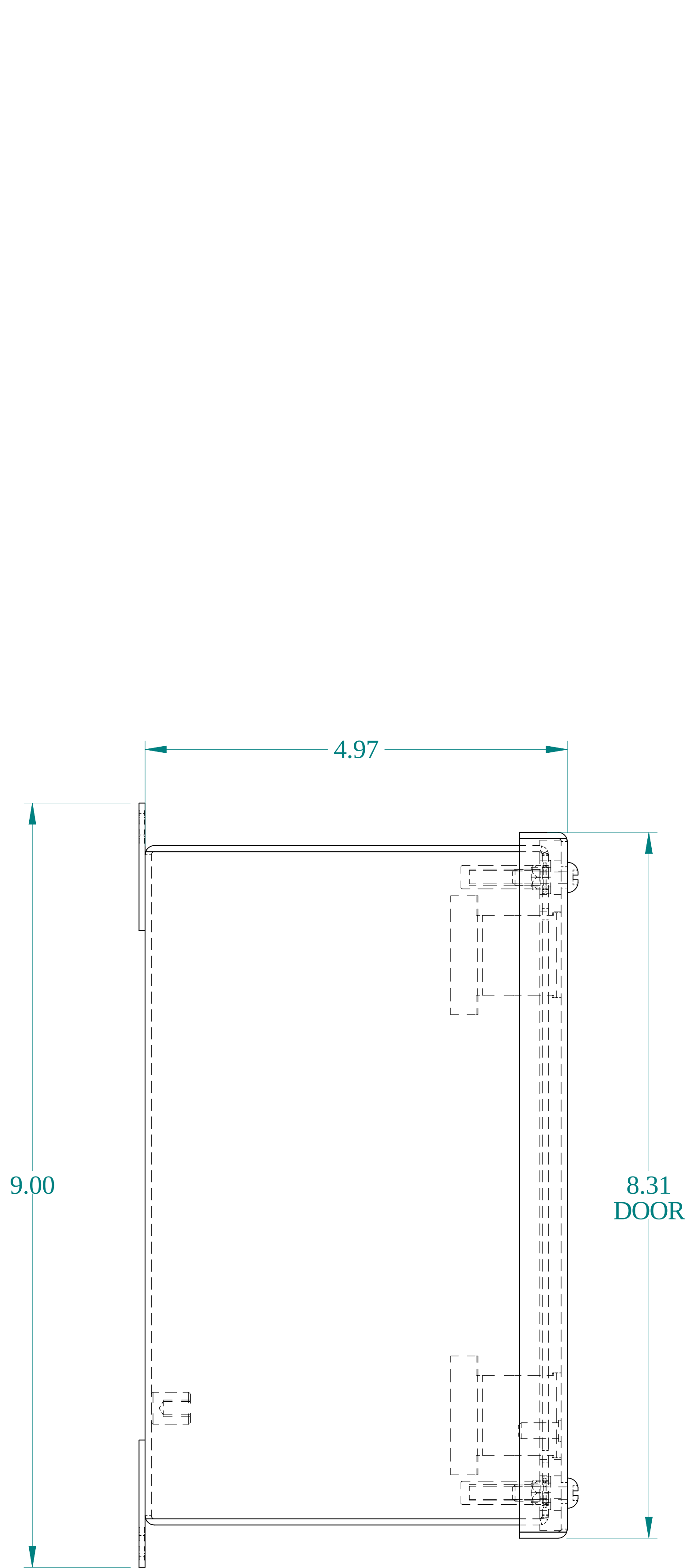
SIDE VIEW
