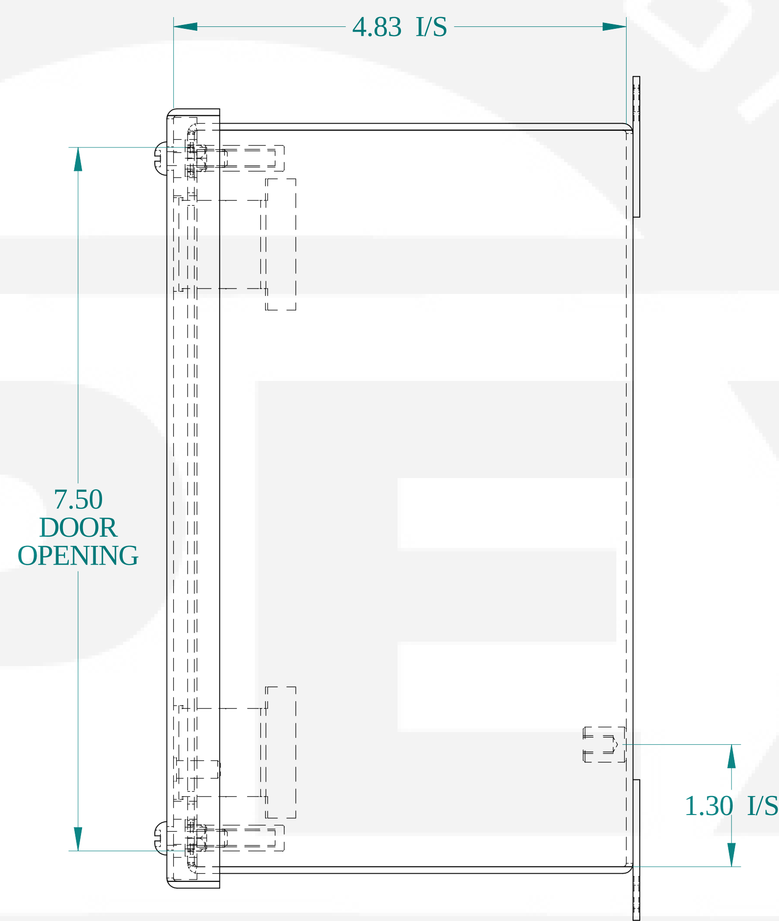
SIDE VIEW
