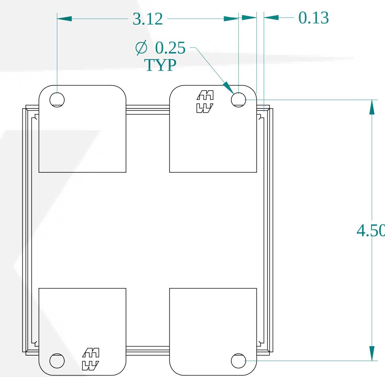
BACK VIEW
