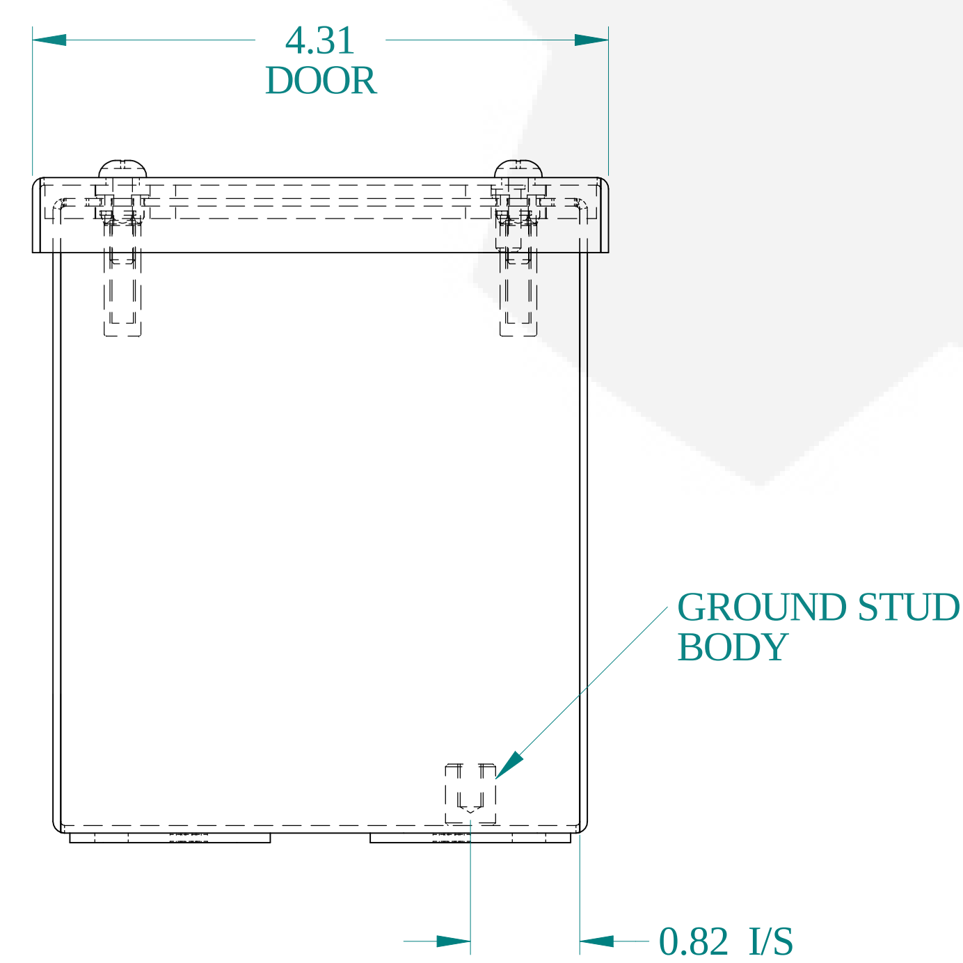
BOTTOM VIEW
