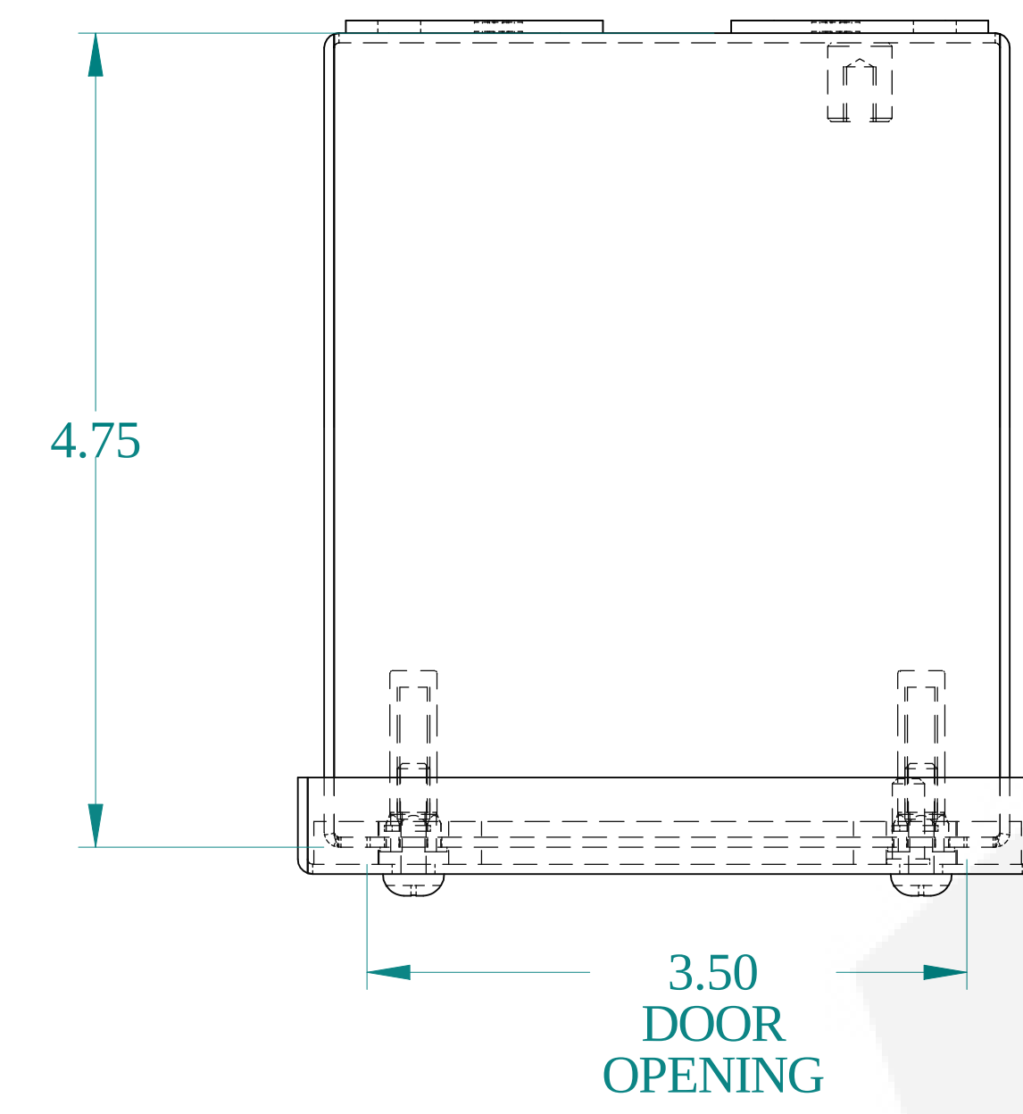
TOP VIEW
