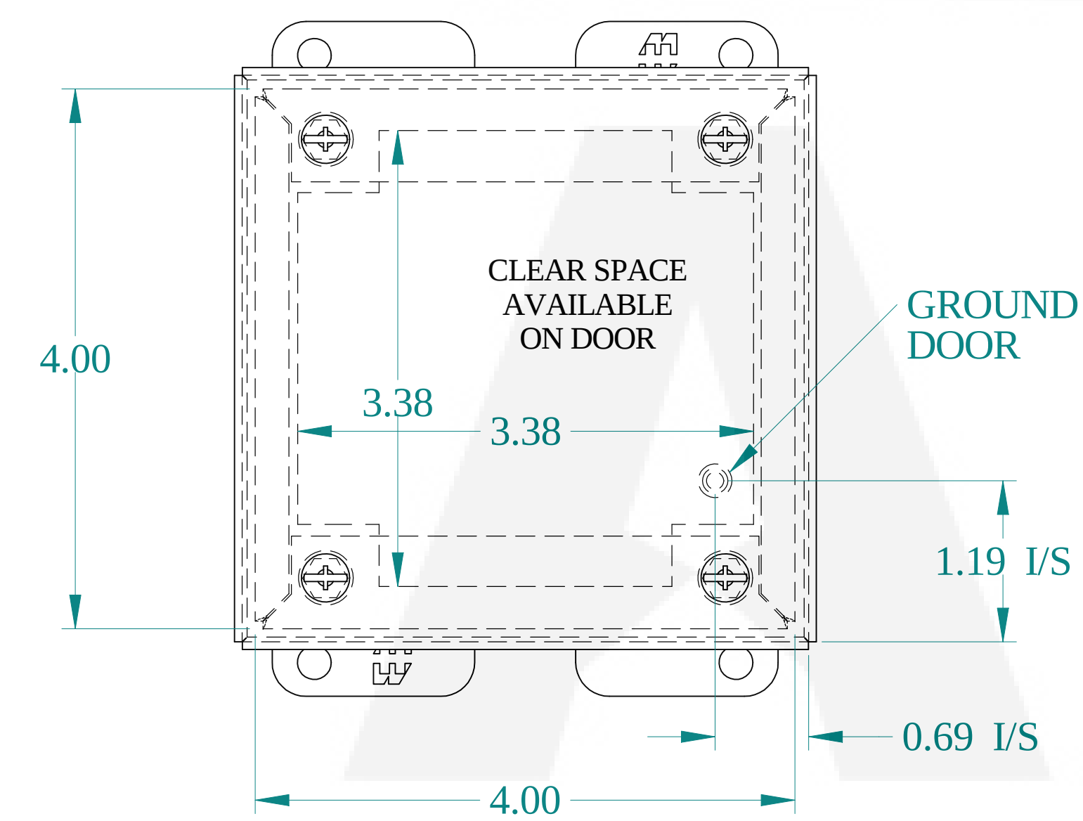
FRONT VIEW
