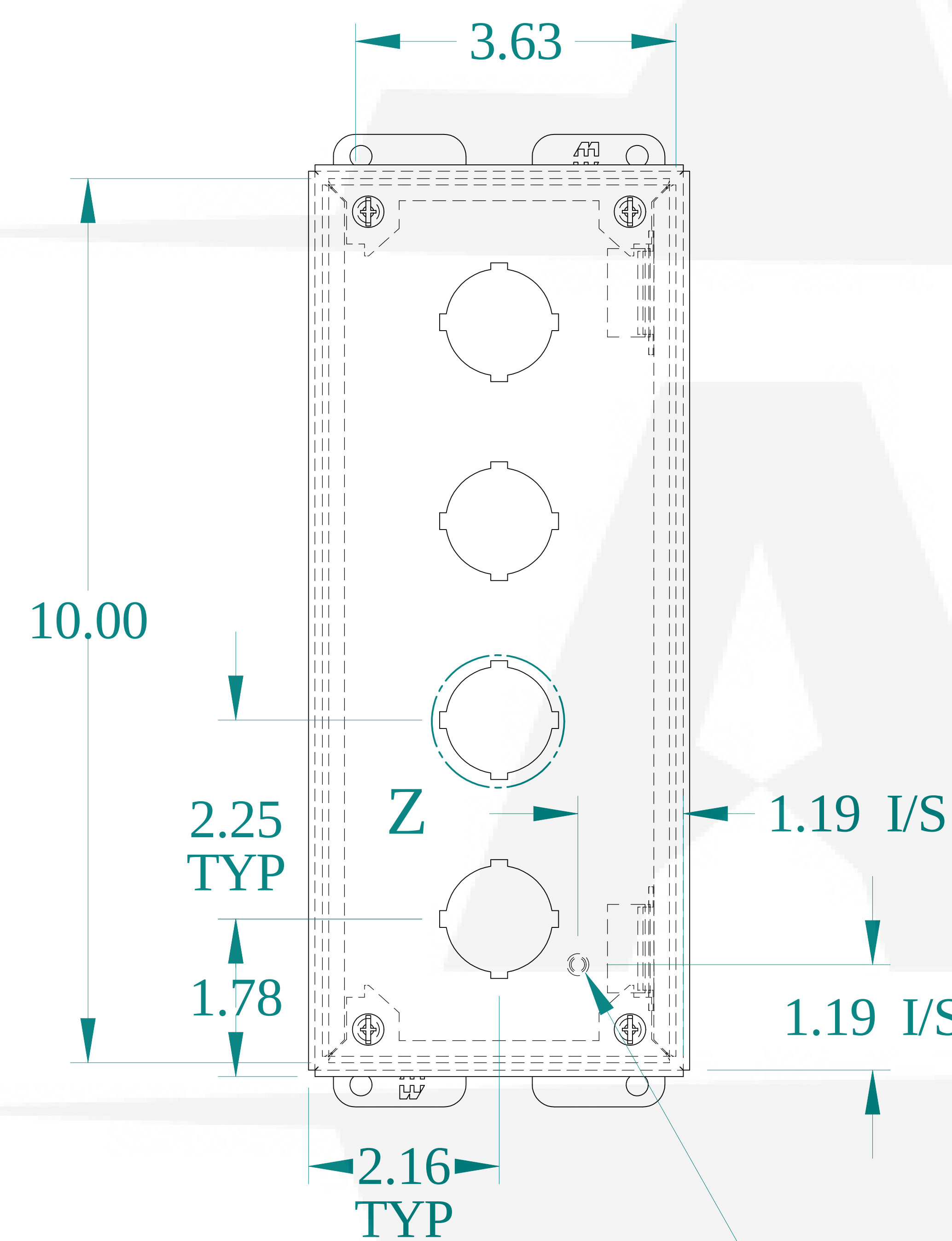
FRONT VIEW
