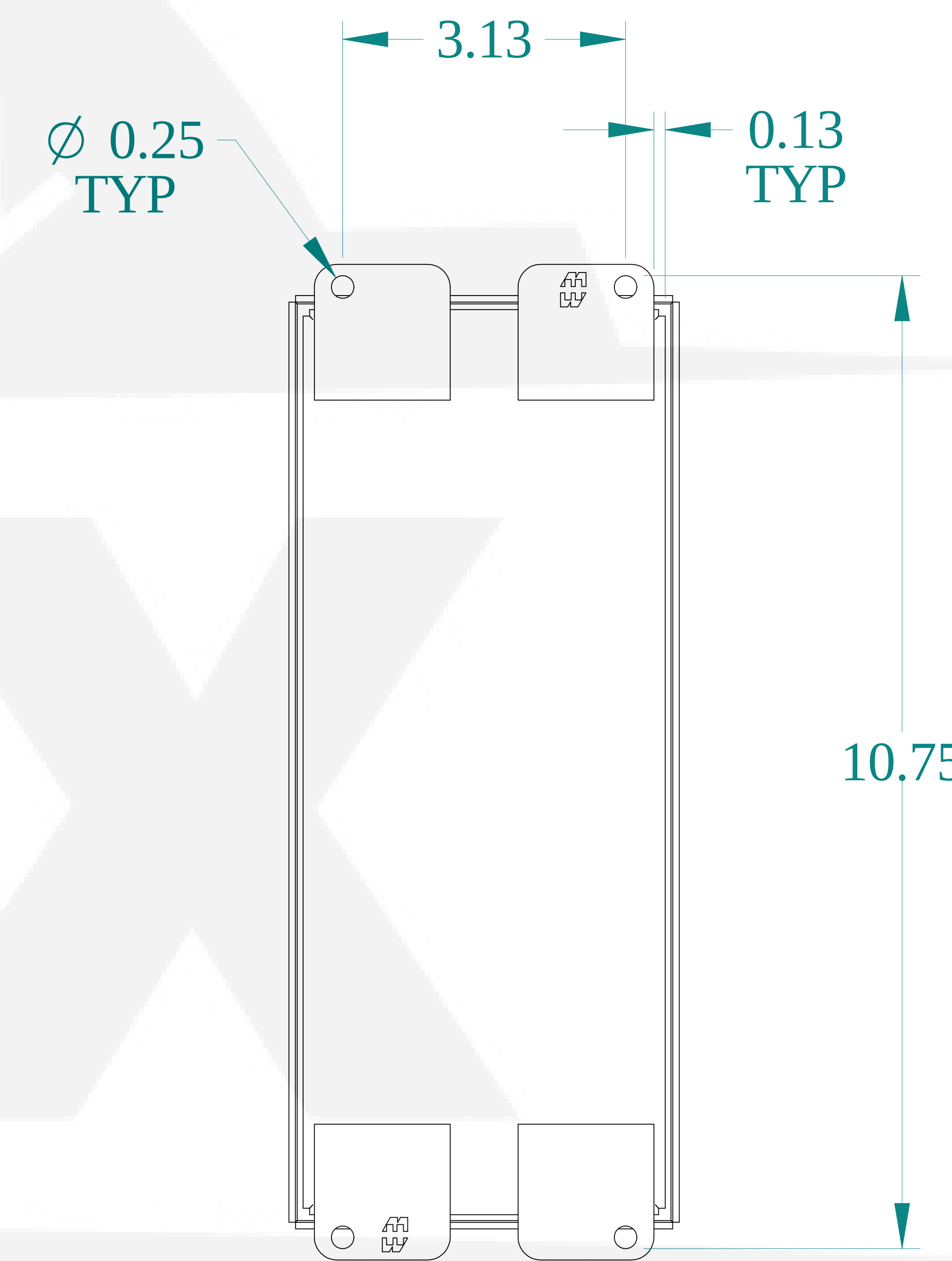
BACK VIEW
