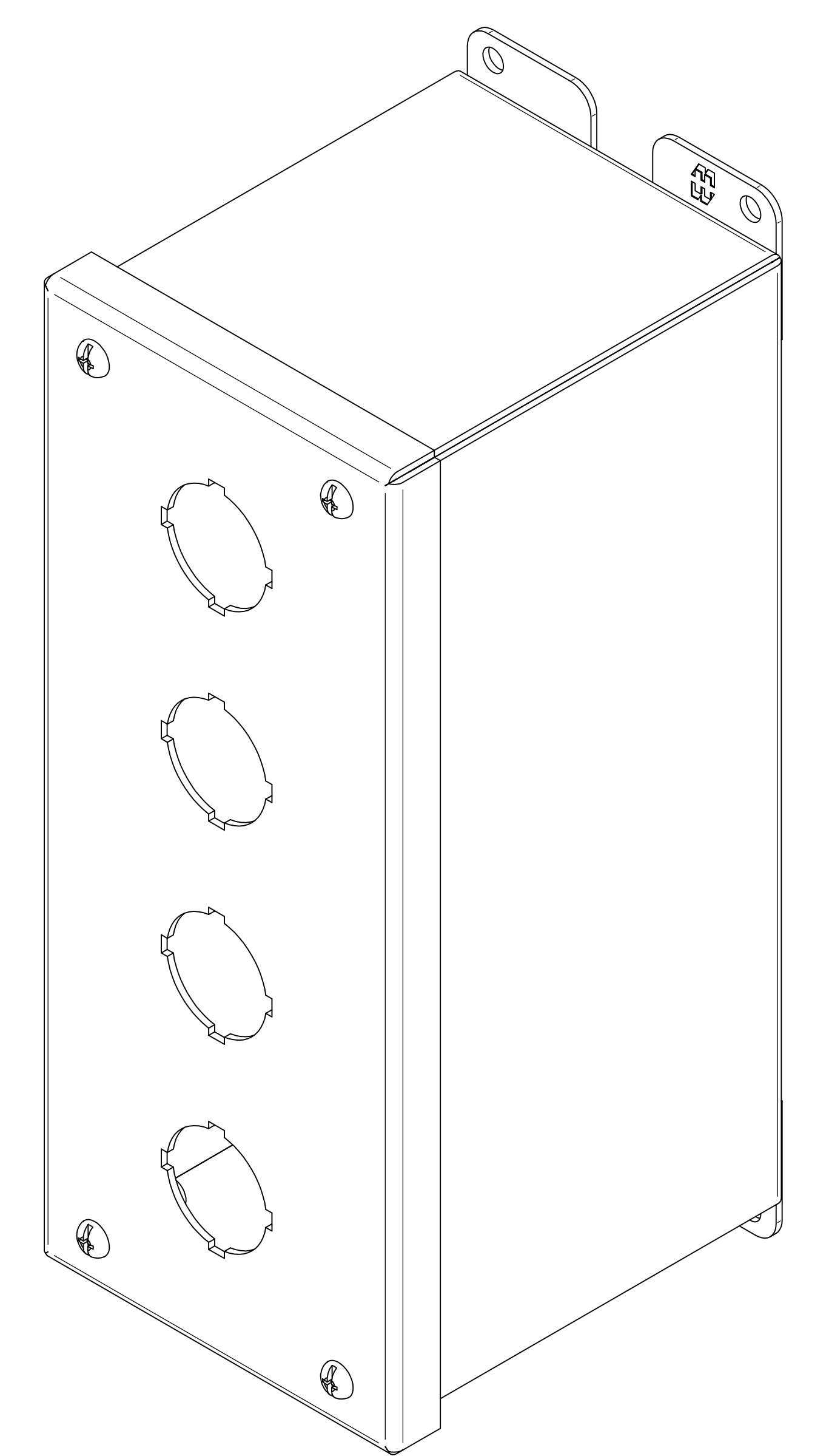
ISOMETRIC VIEWS
