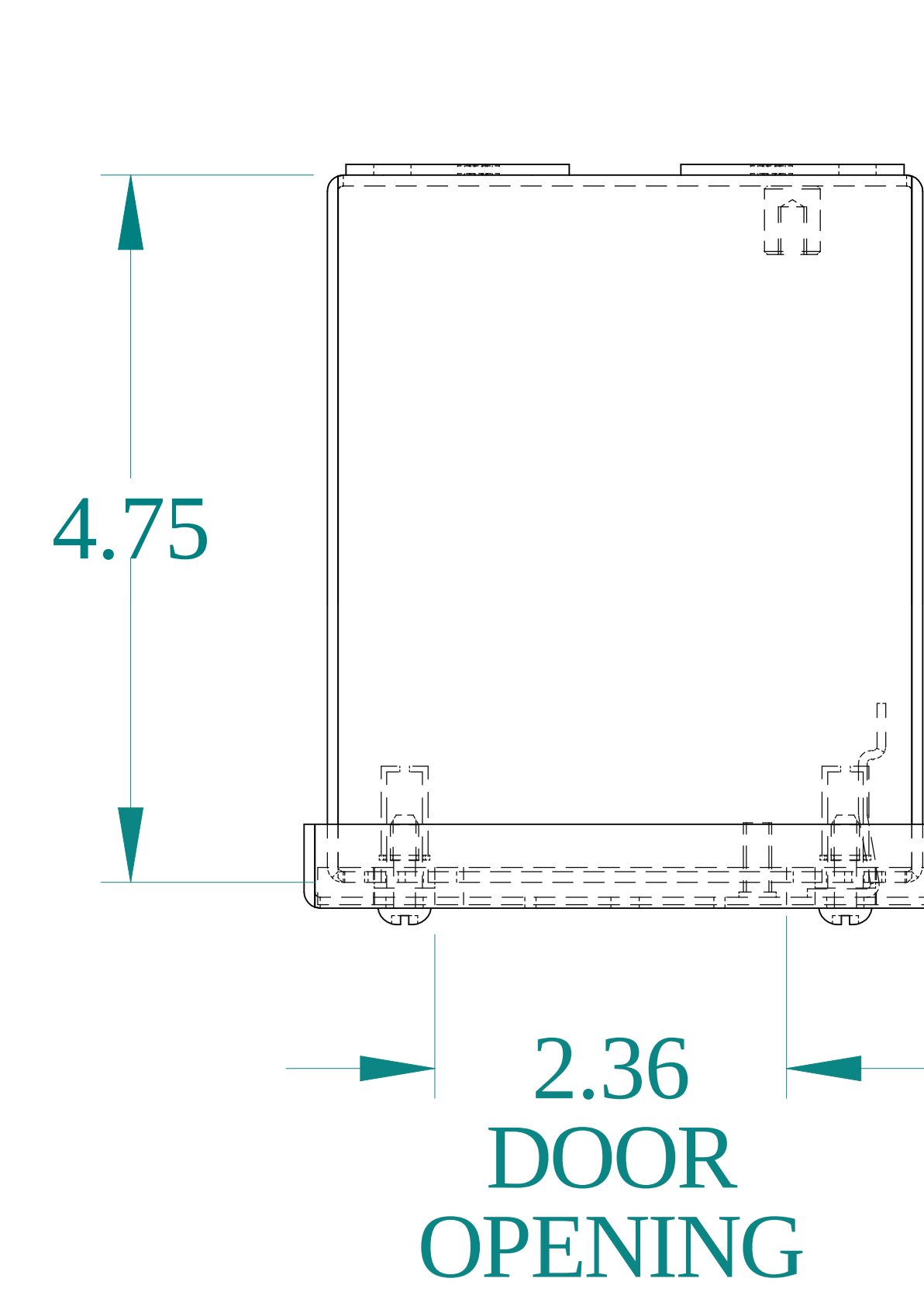
TOP VIEW
