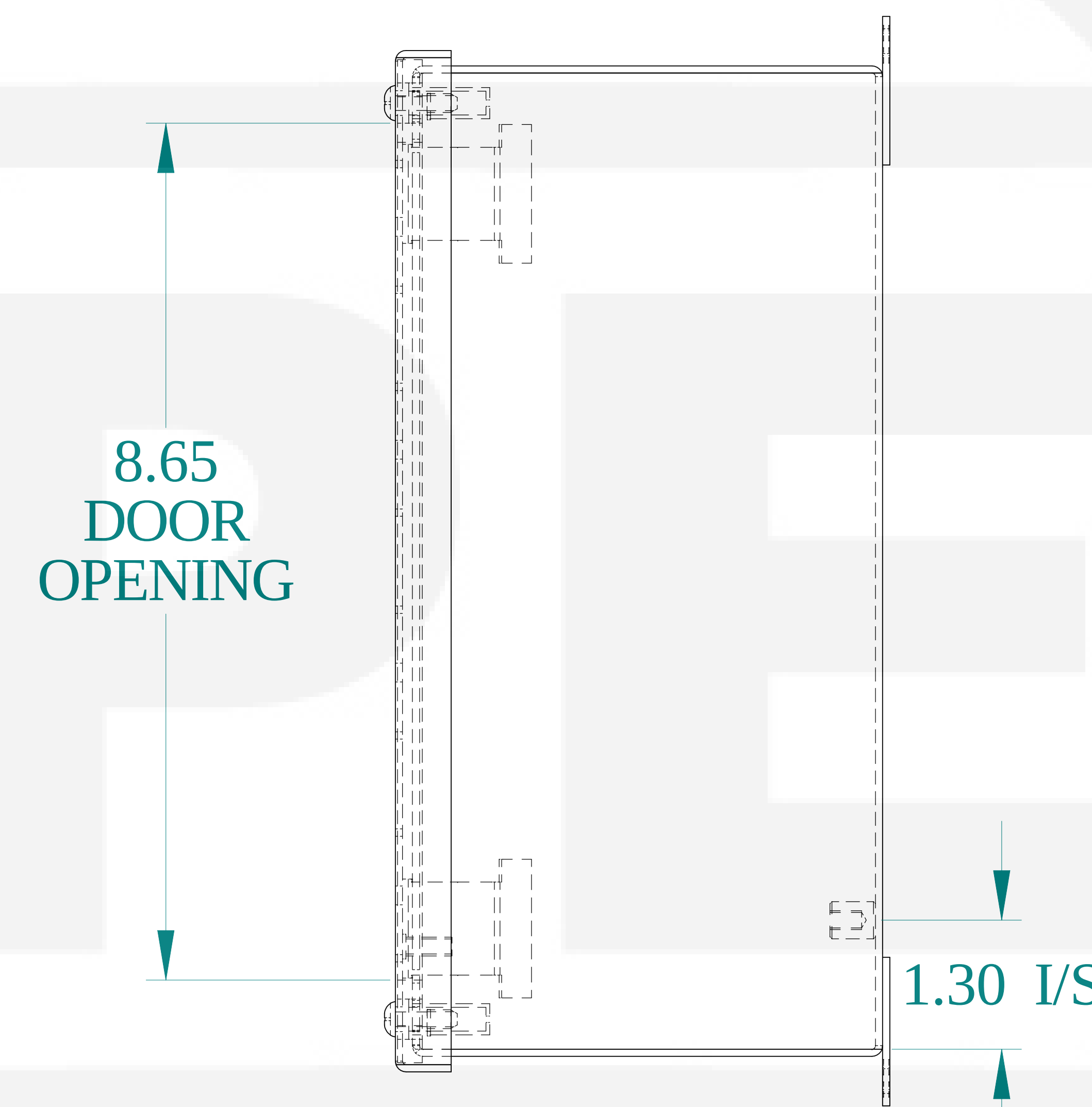
SIDE VIEW
