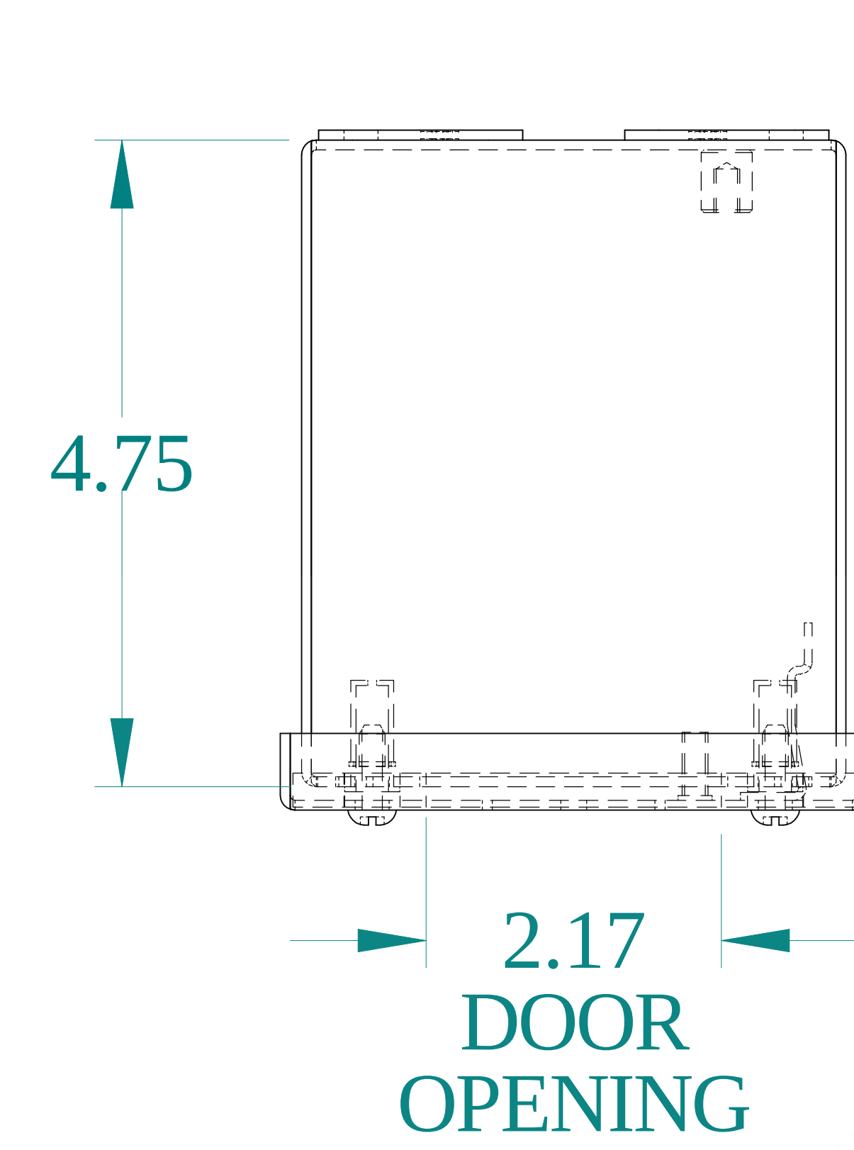
TOP VIEW
