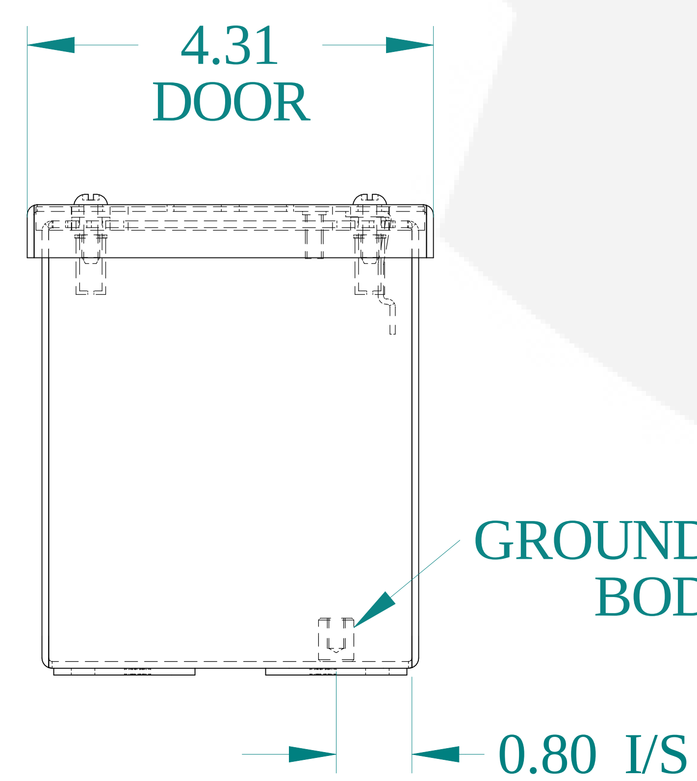
BOTTOM VIEW
