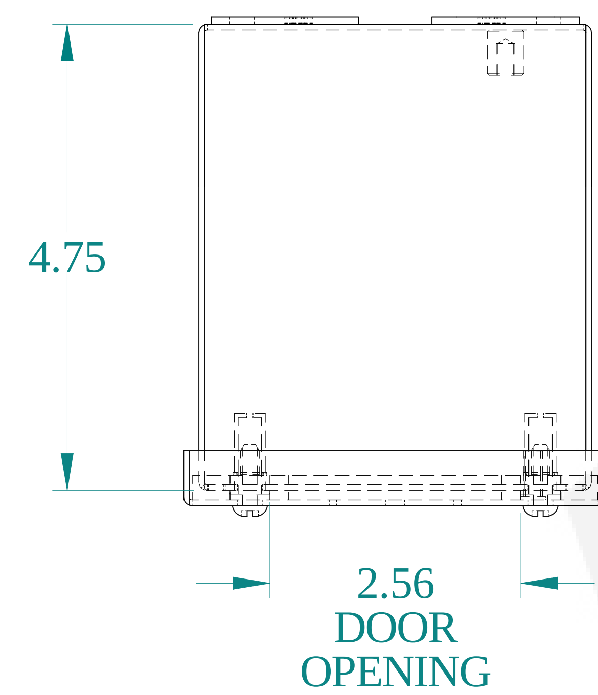
TOP VIEW
