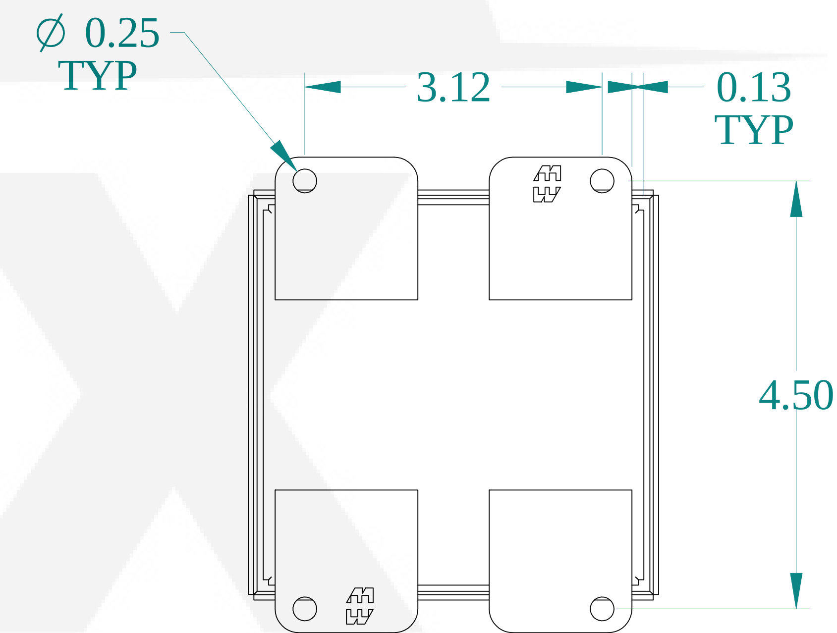
BACK VIEW
