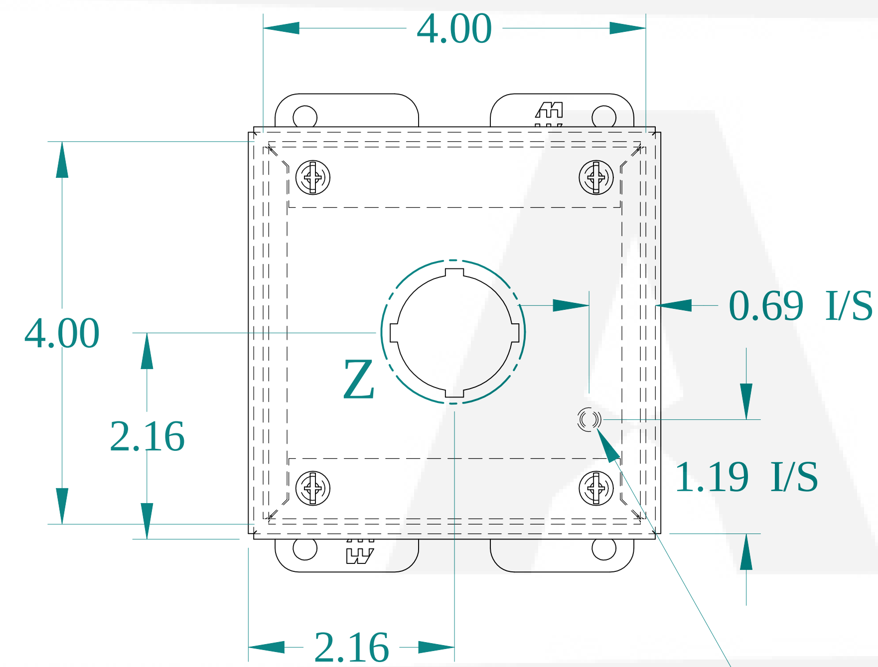
FRONT VIEW
