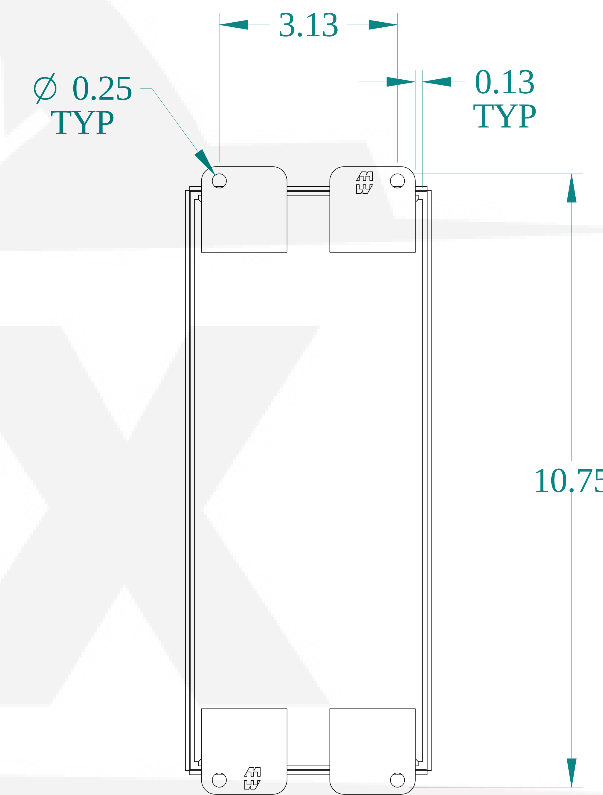
BACK VIEW
