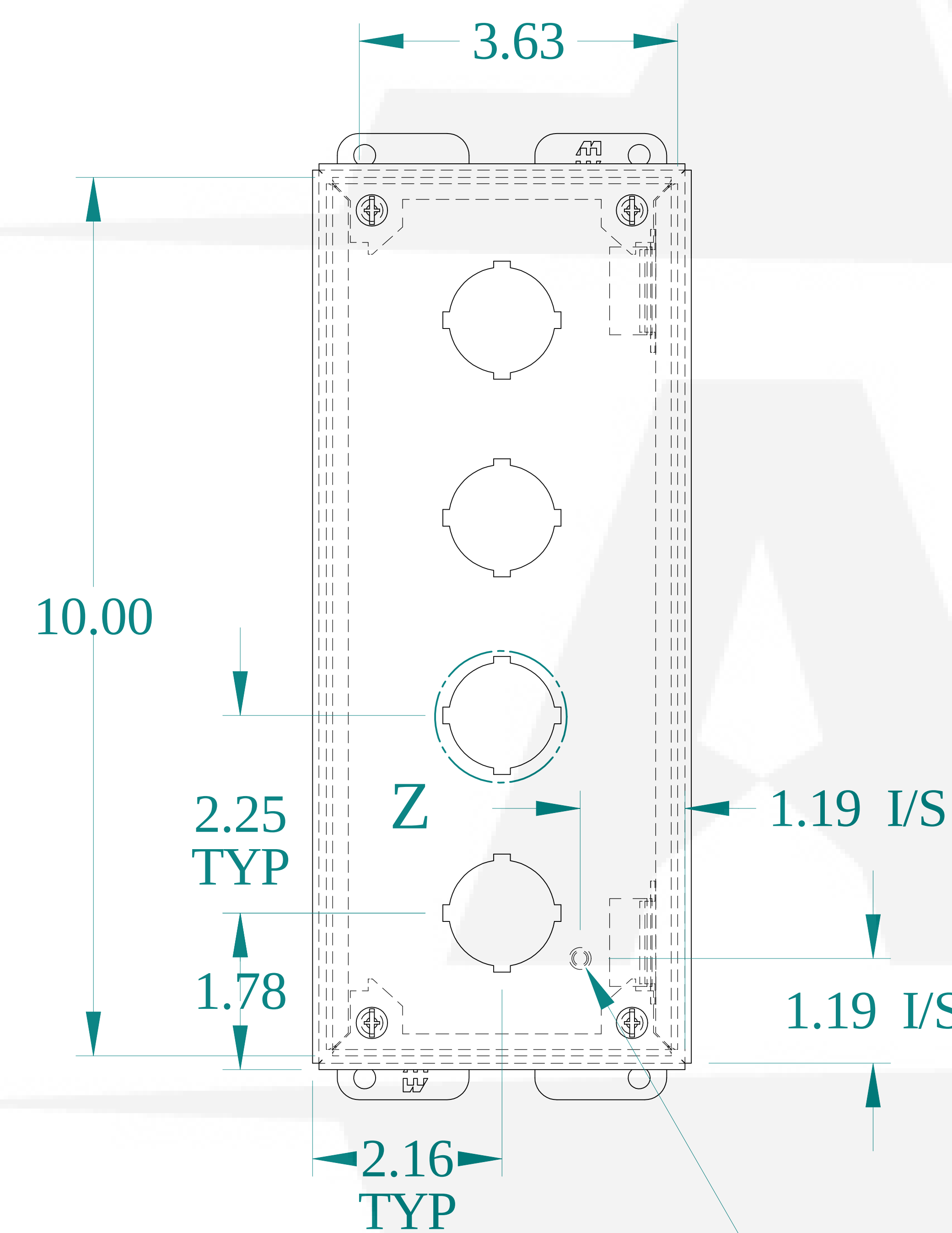
FRONT VIEW
