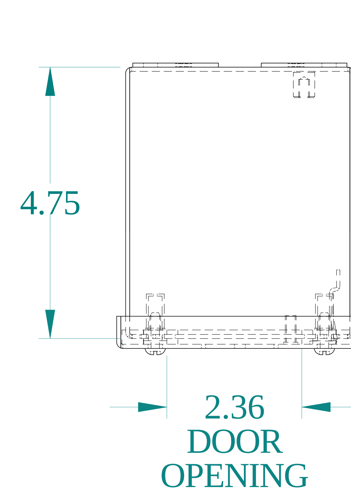
TOP VIEW
