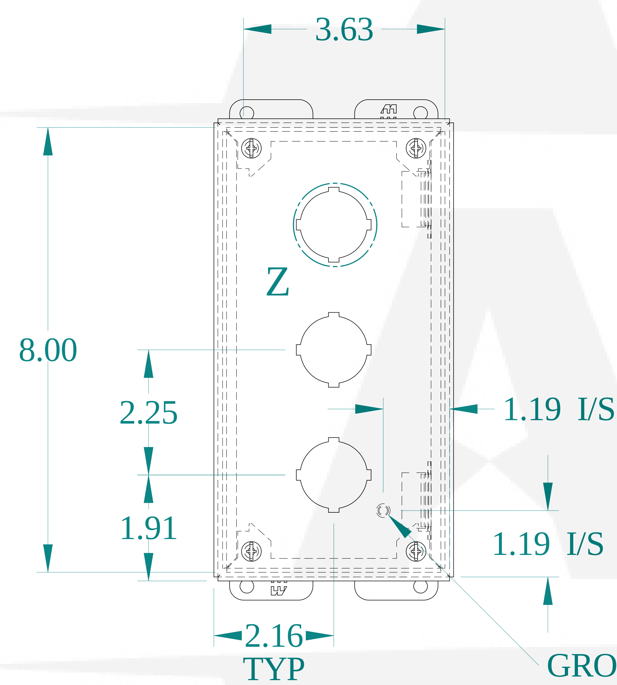
FRONT VIEW
