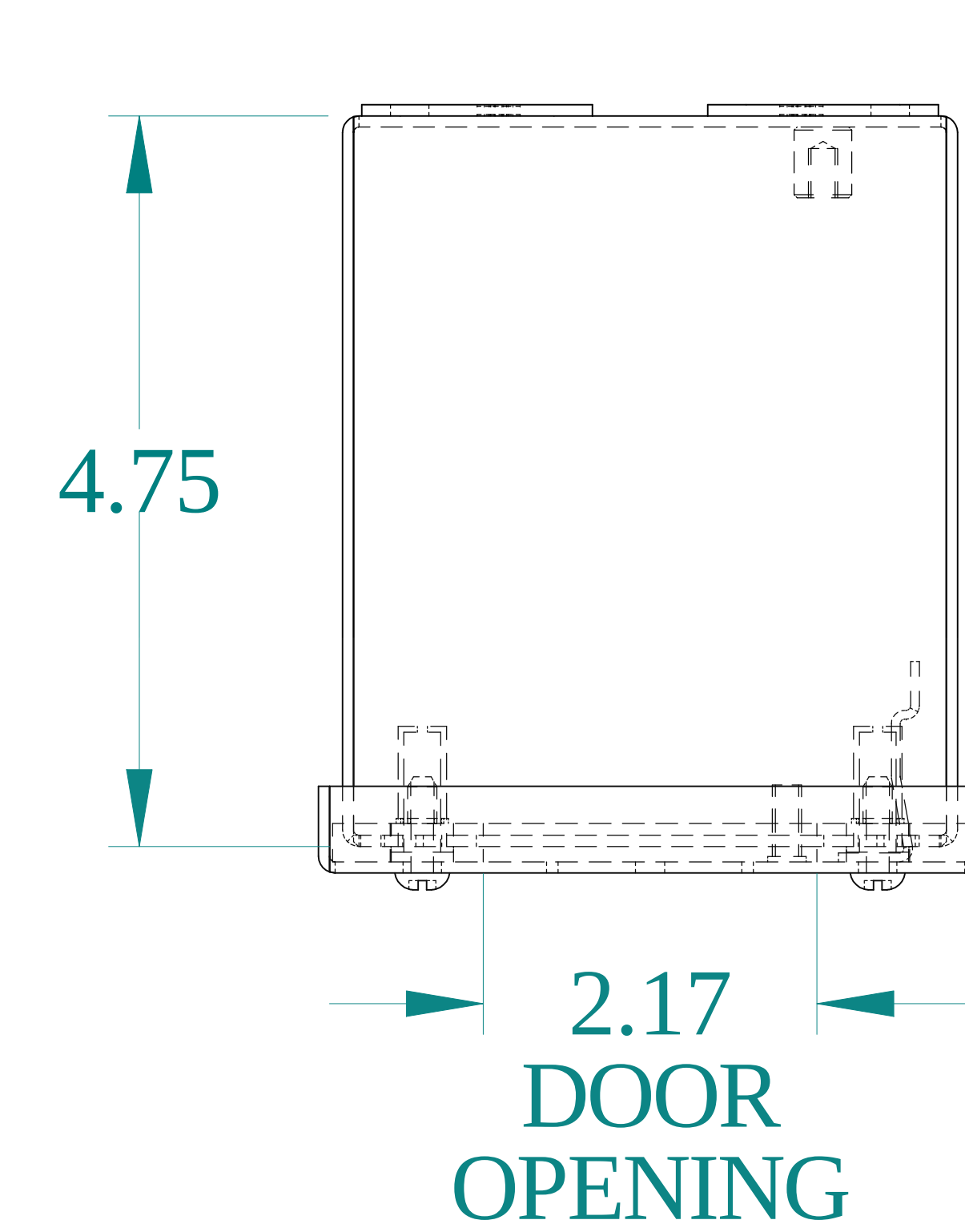
TOP VIEW
