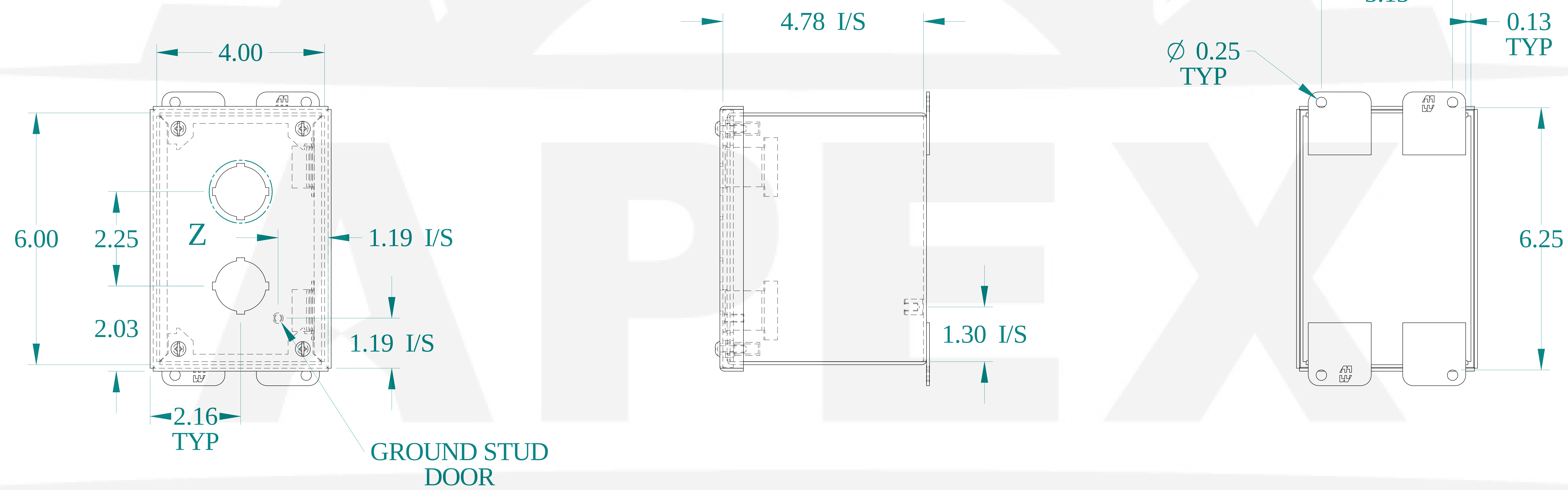
BACK VIEW
