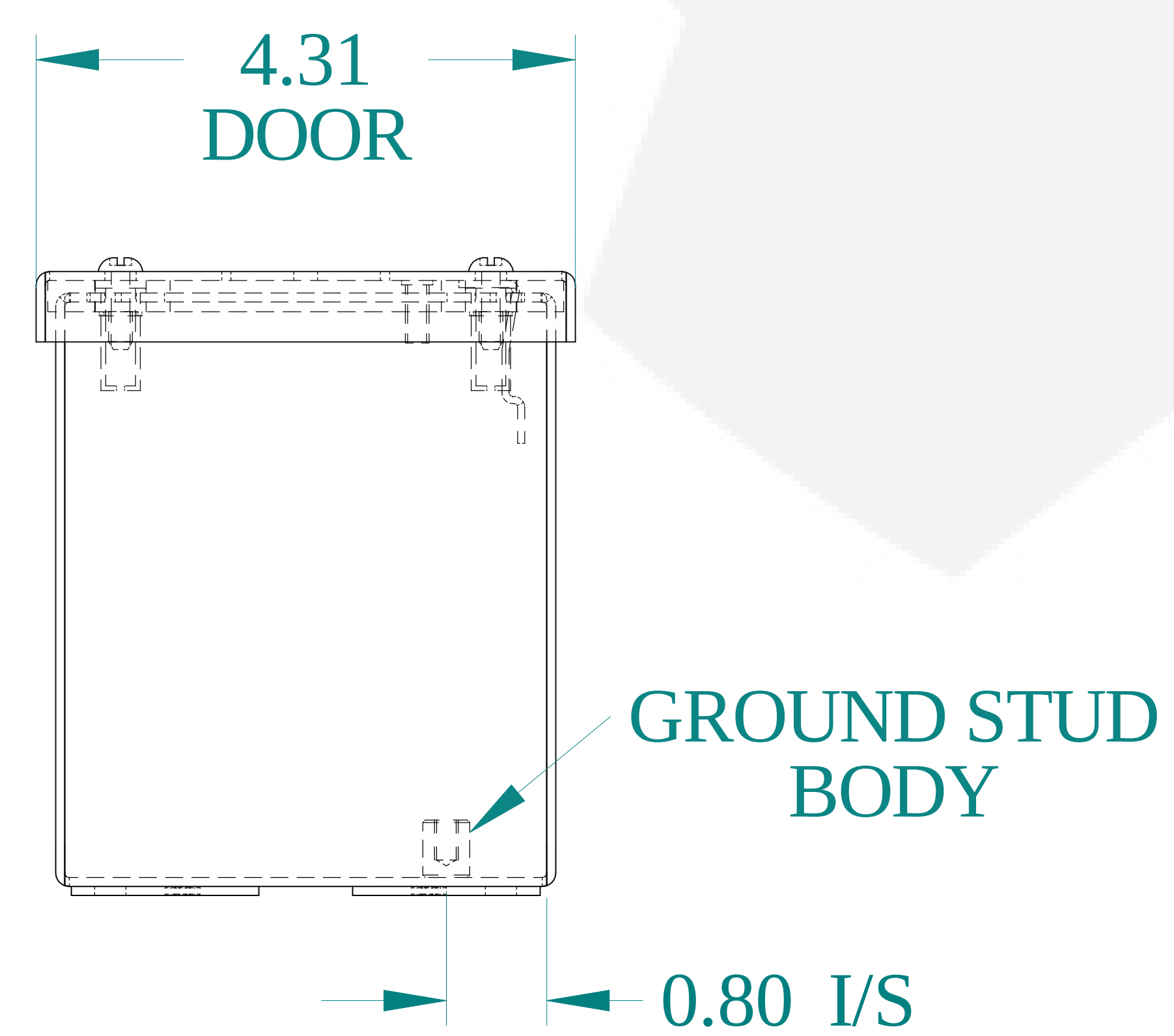
BOTTOM VIEW
