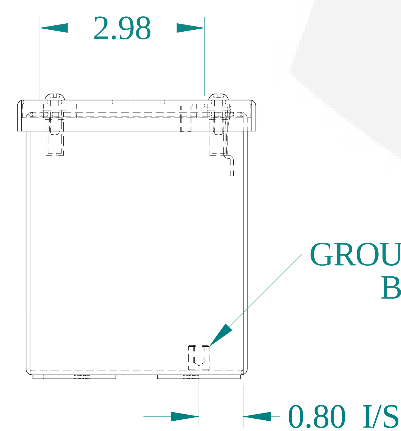
BOTTOM VIEW
