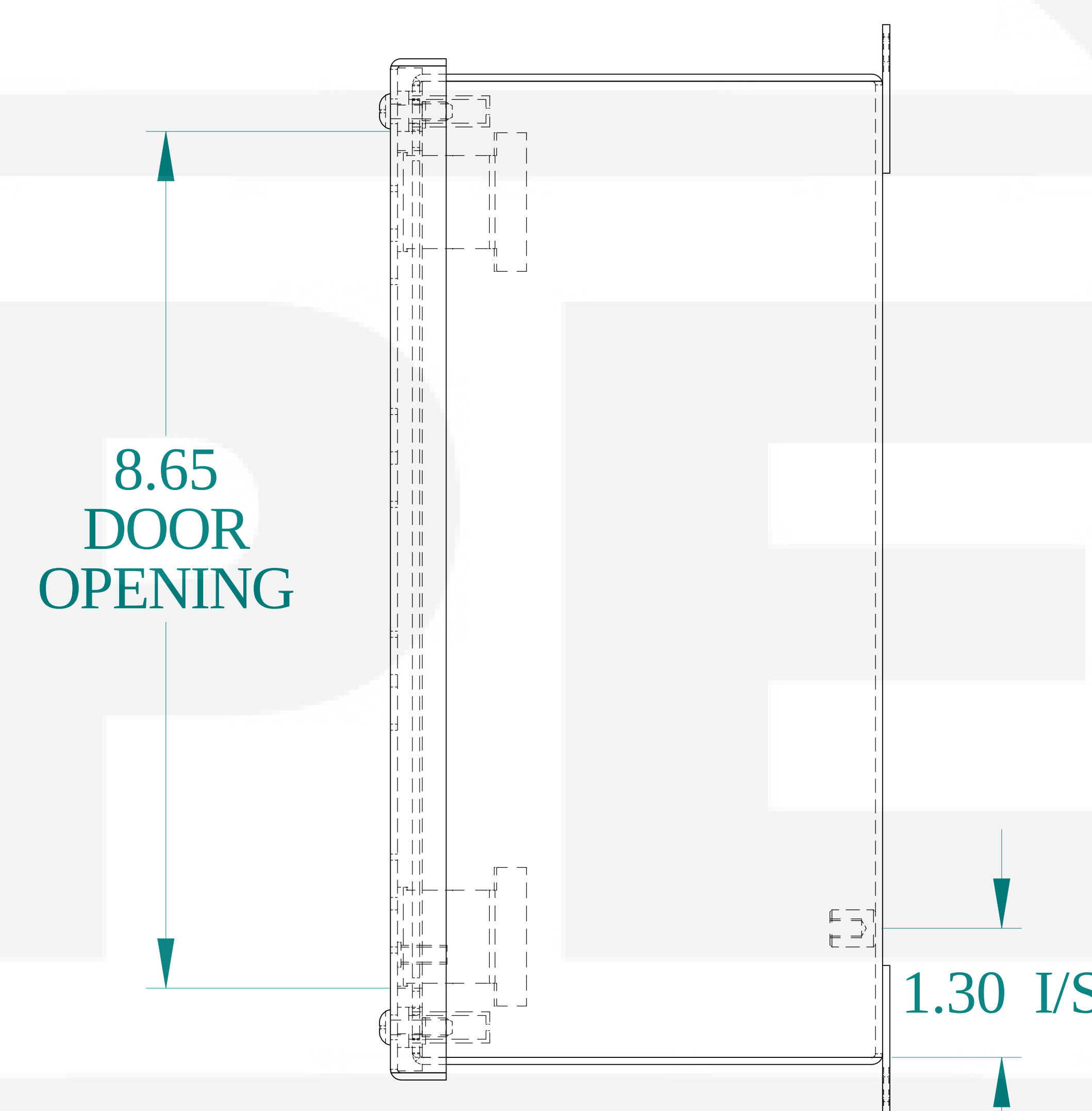
SIDE VIEW
