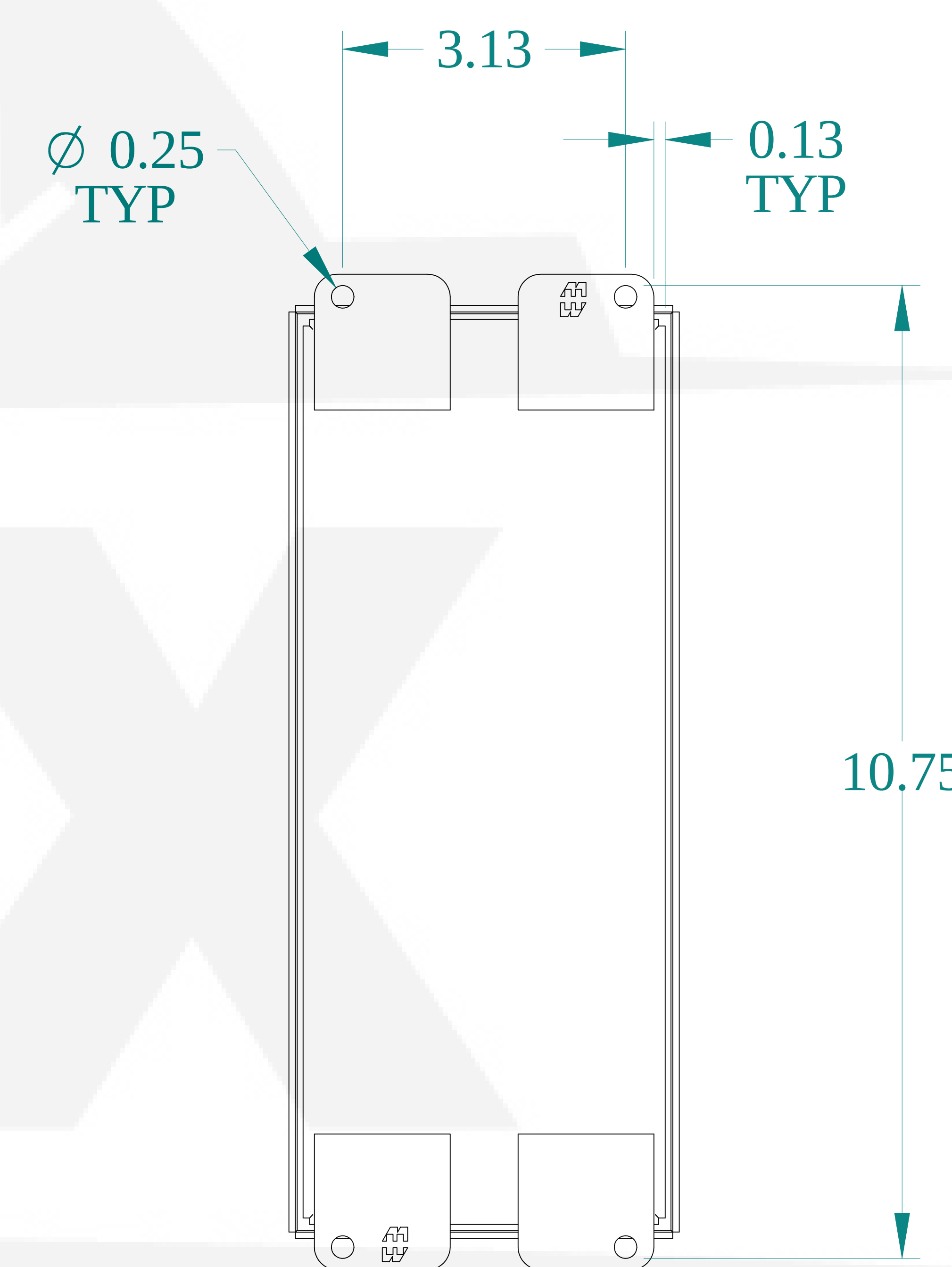
BACK VIEW
