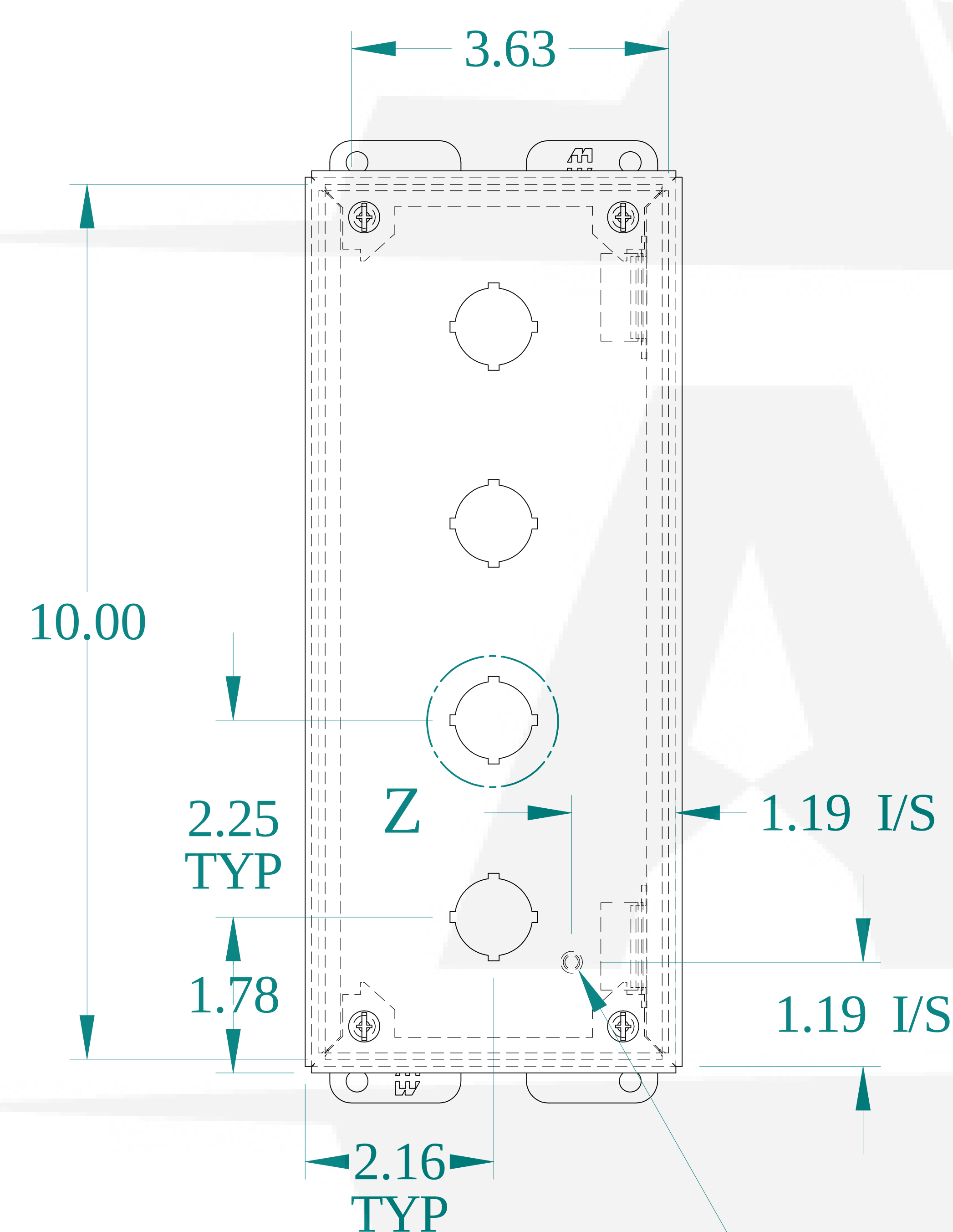
FRONT VIEW
