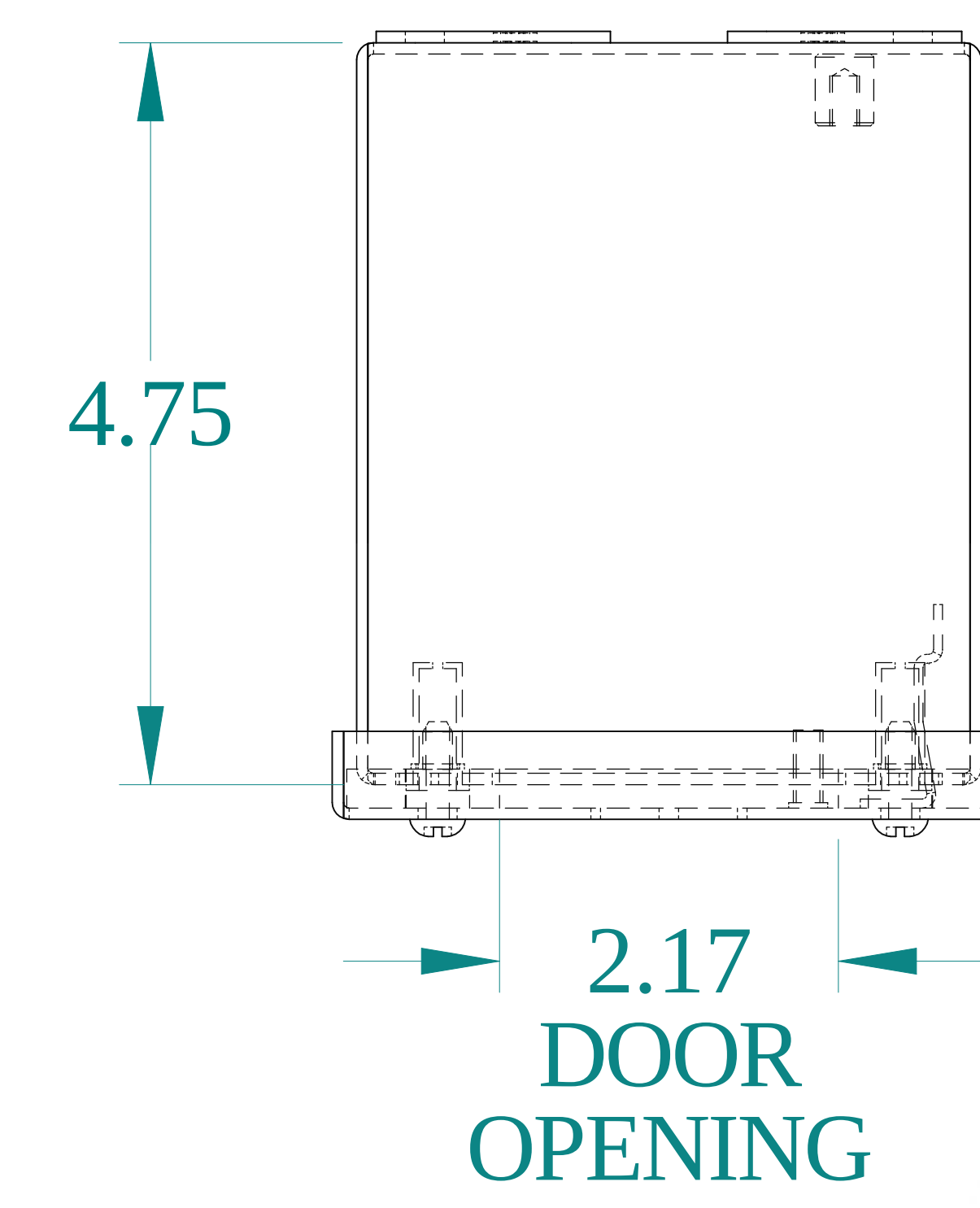
TOP VIEW
