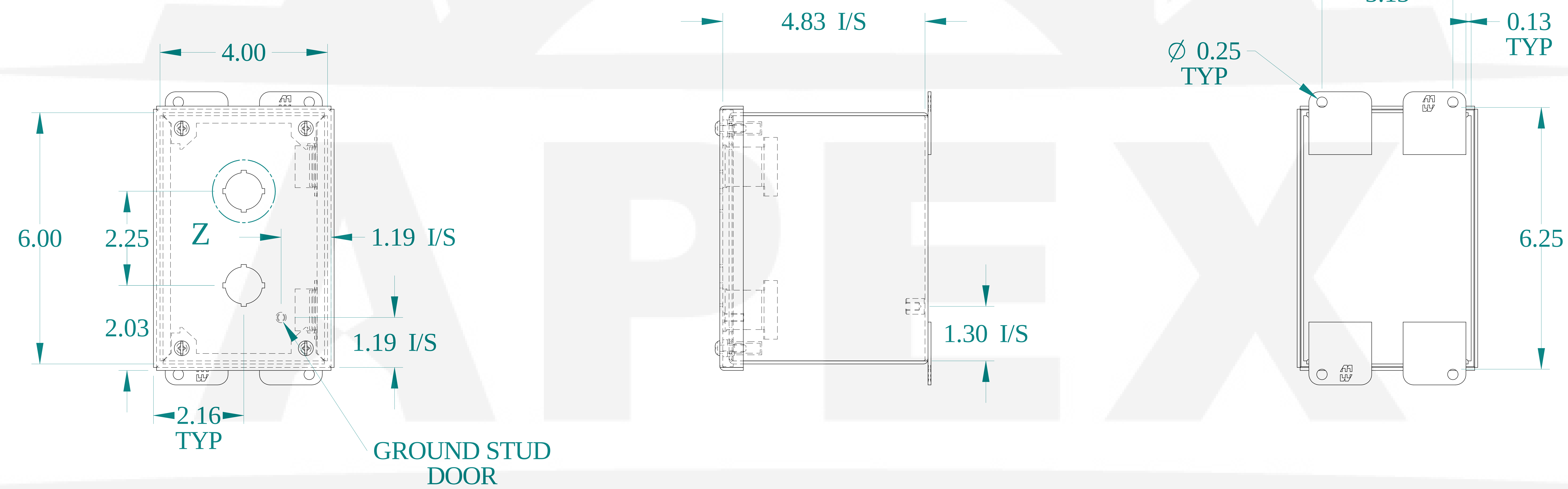
BACK VIEW
