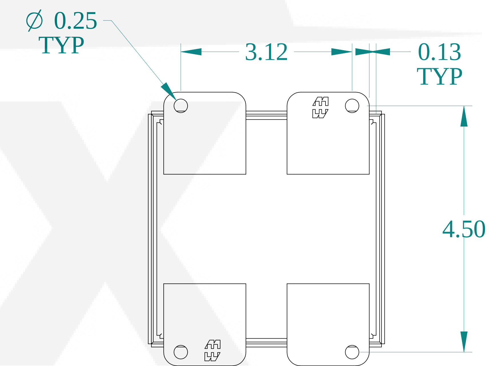
BACK VIEW
