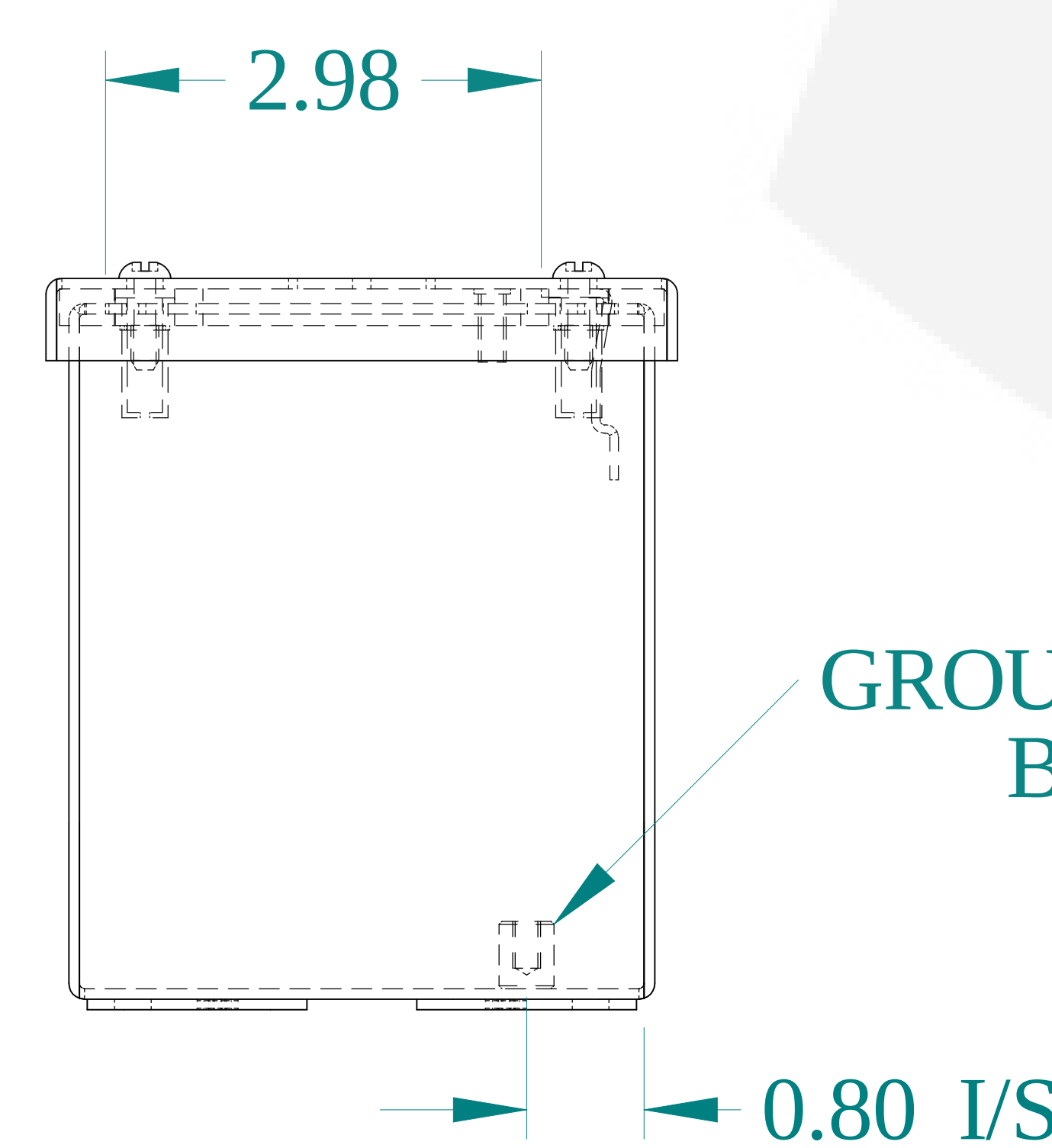
BOTTOM VIEW
