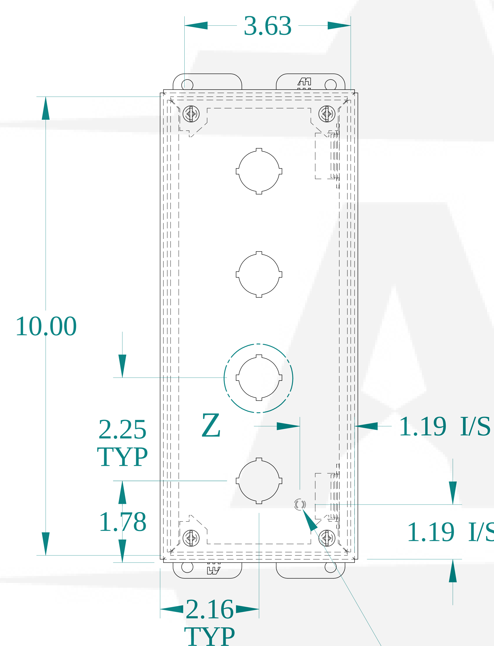
FRONT VIEW
