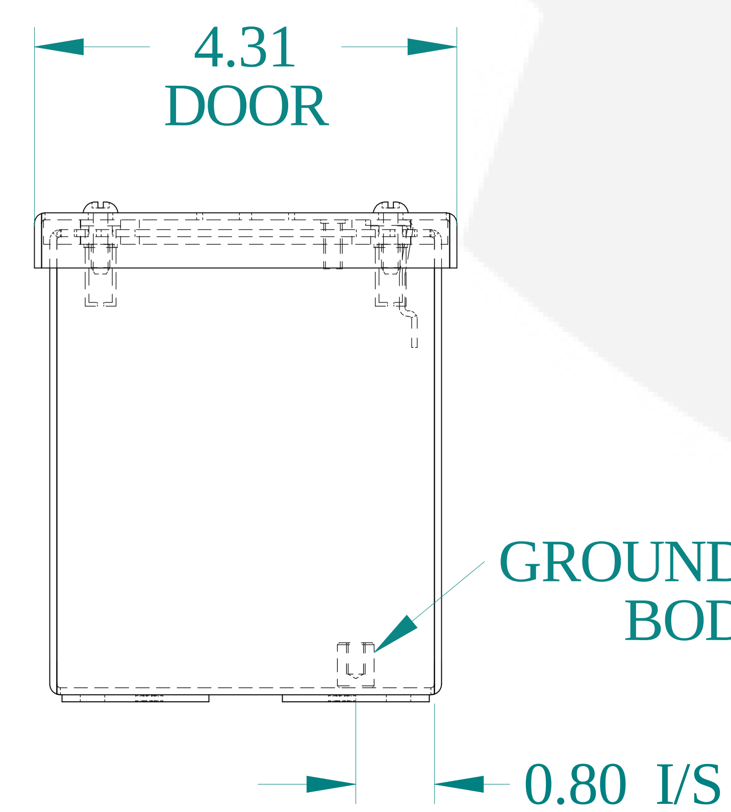
BOTTOM VIEW
