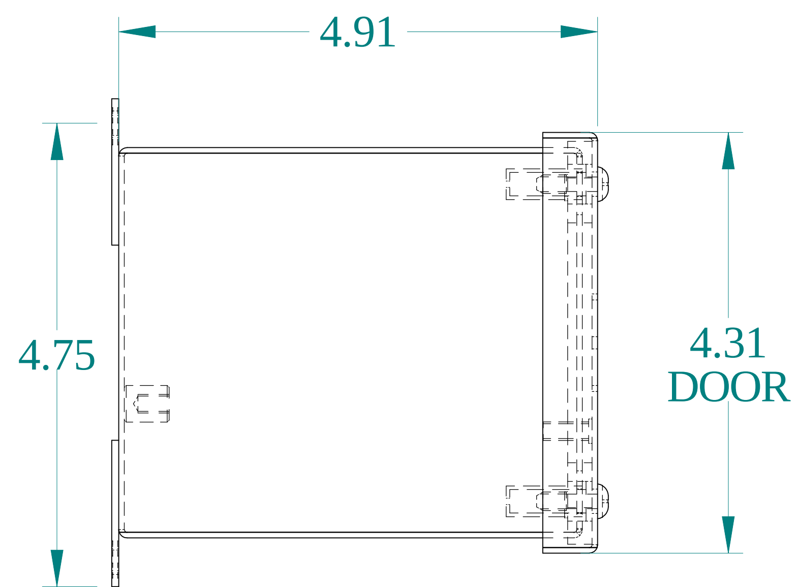
SIDE VIEW
