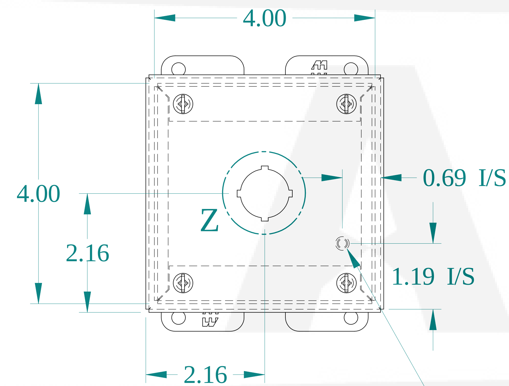
FRONT VIEW
