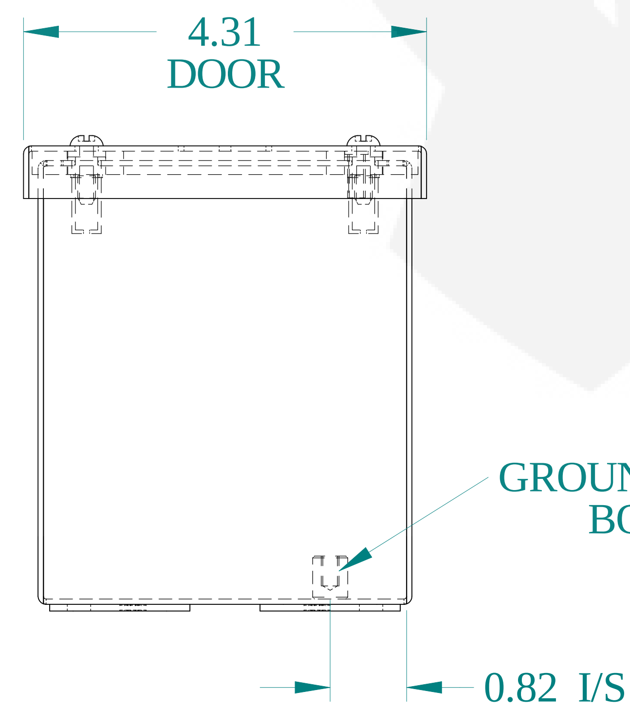
BOTTOM VIEW
