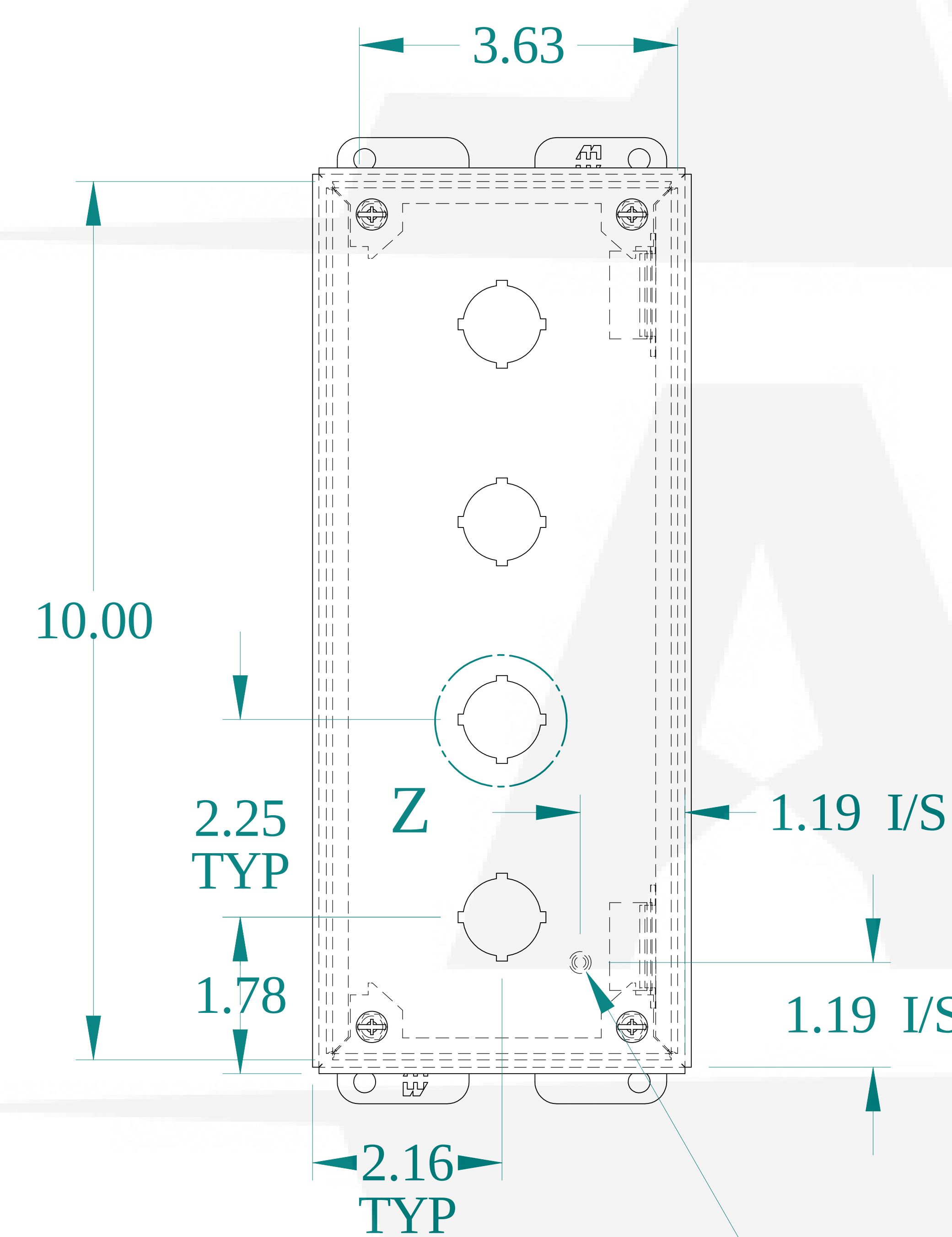
FRONT VIEW
