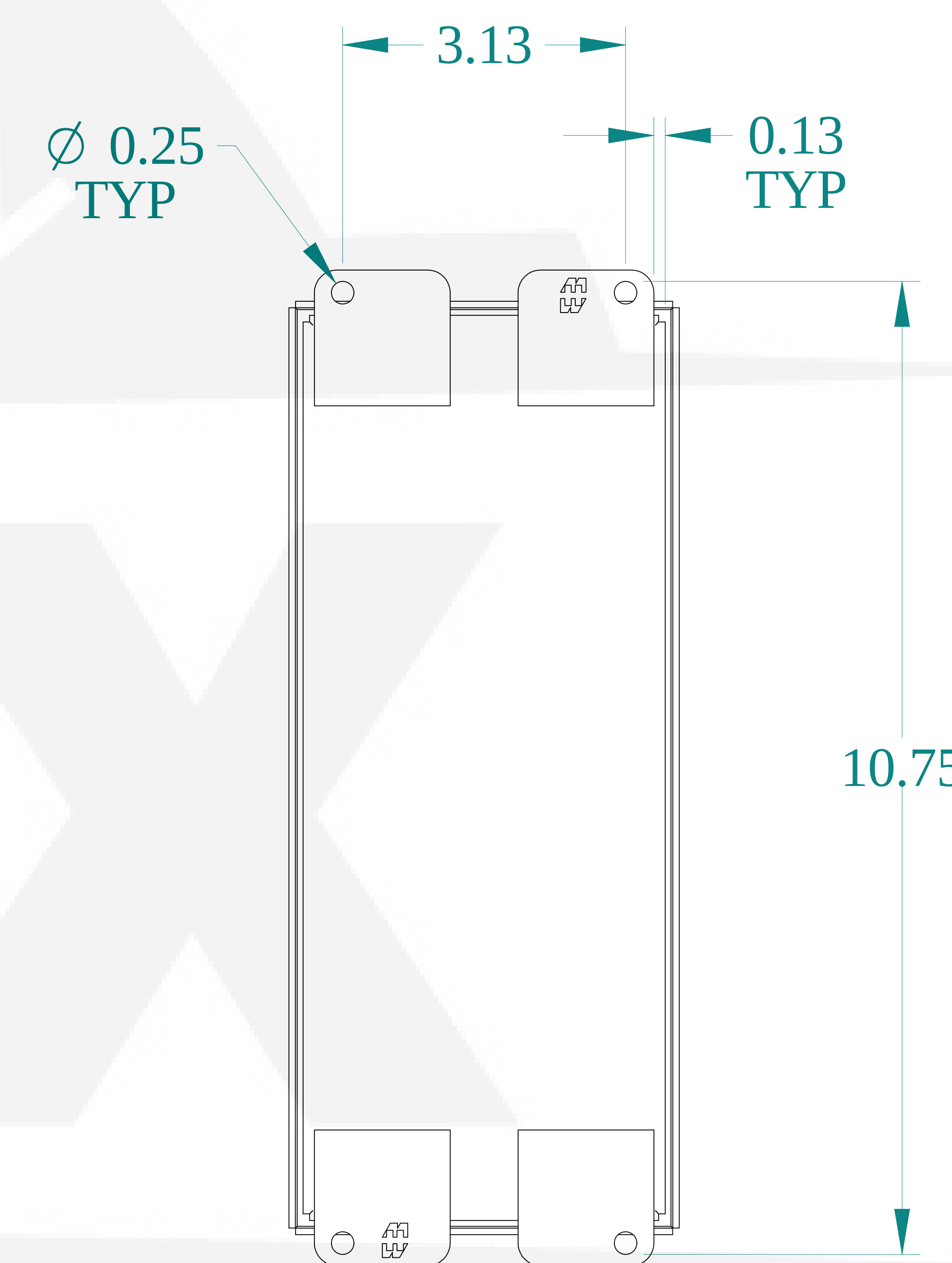
BACK VIEW
