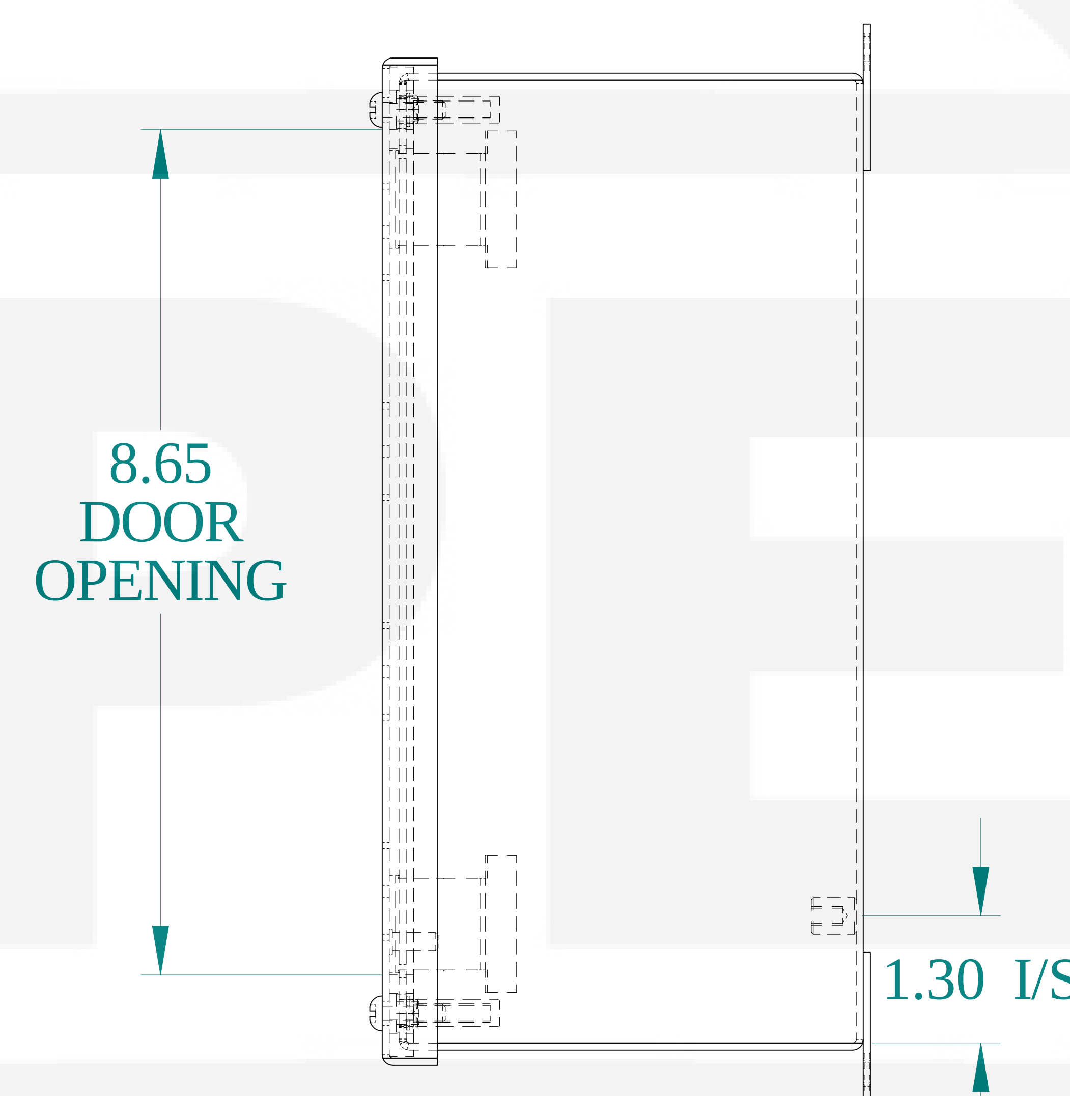
SIDE VIEW
