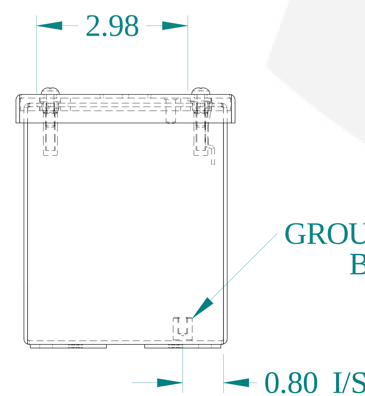
BOTTOM VIEW
