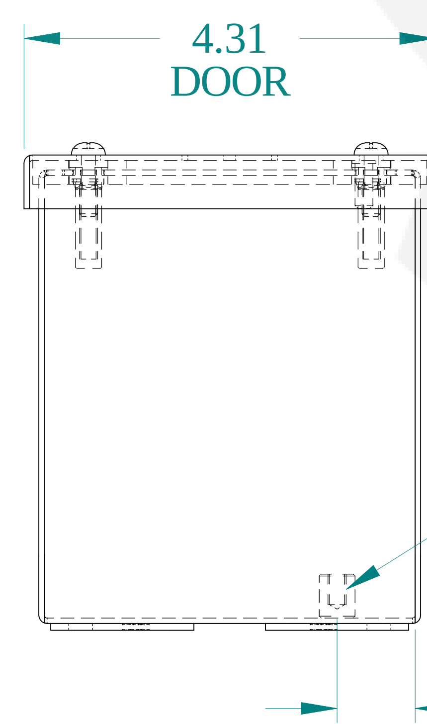
BOTTOM VIEW
