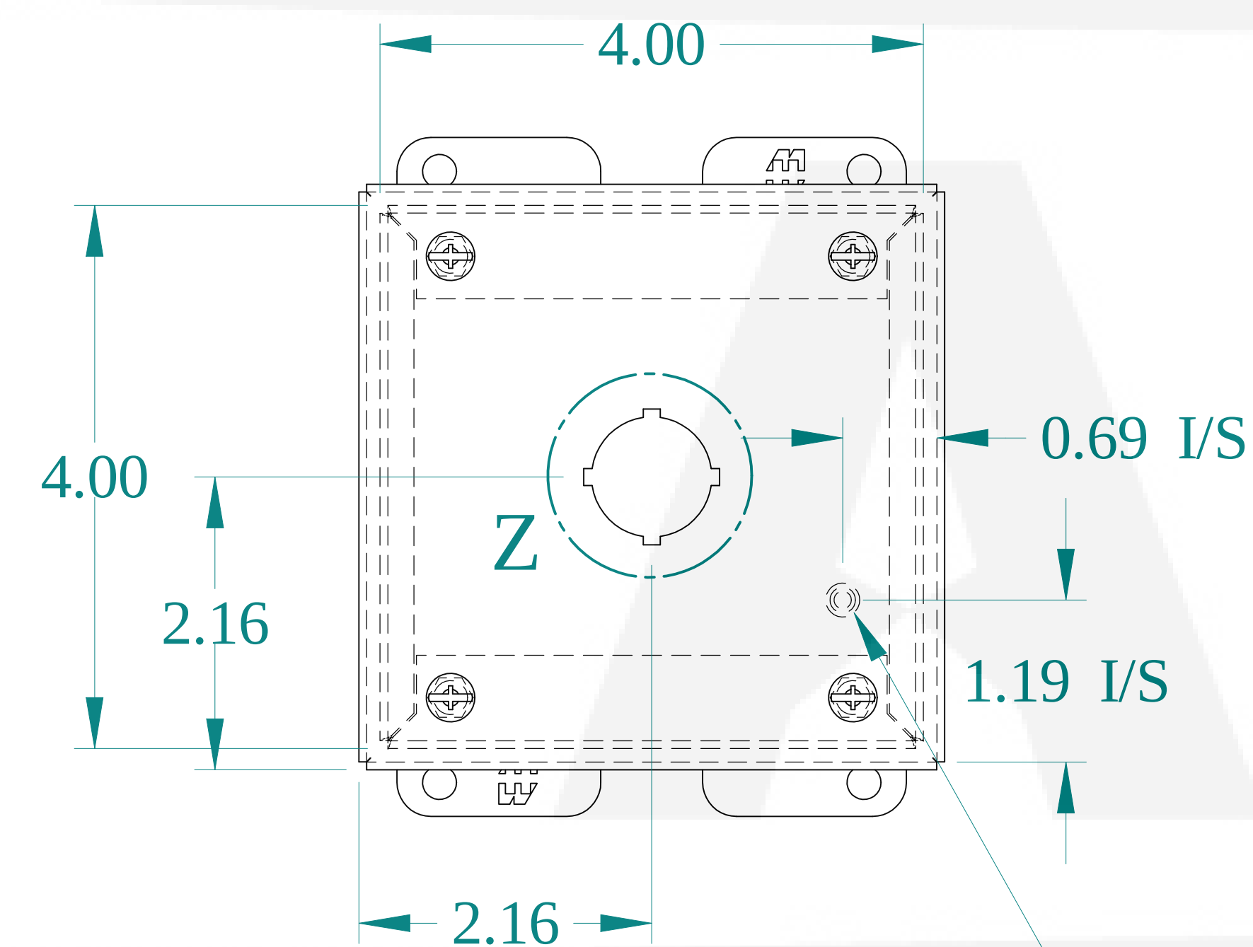
FRONT VIEW
