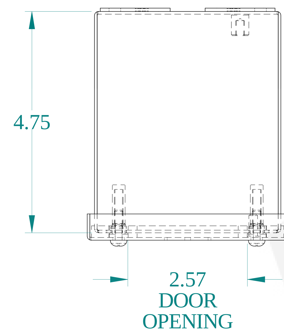
TOP VIEW
