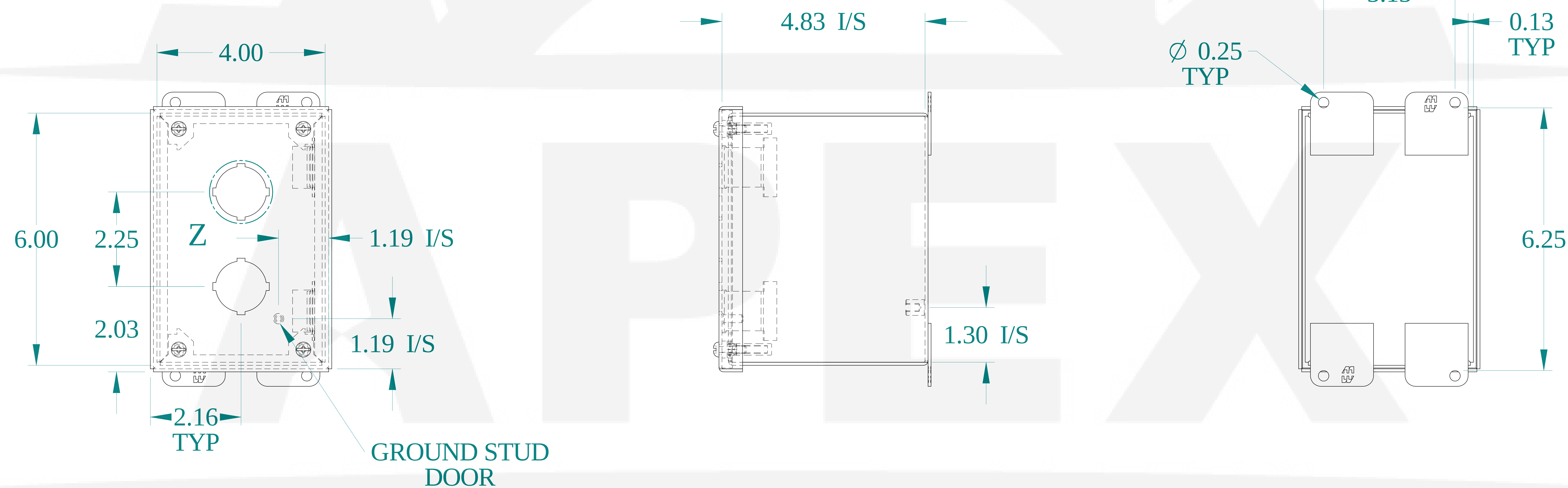
BACK VIEW
