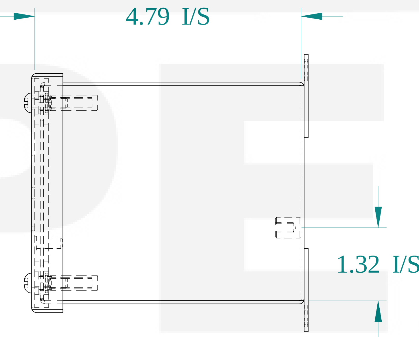
SIDE VIEW
