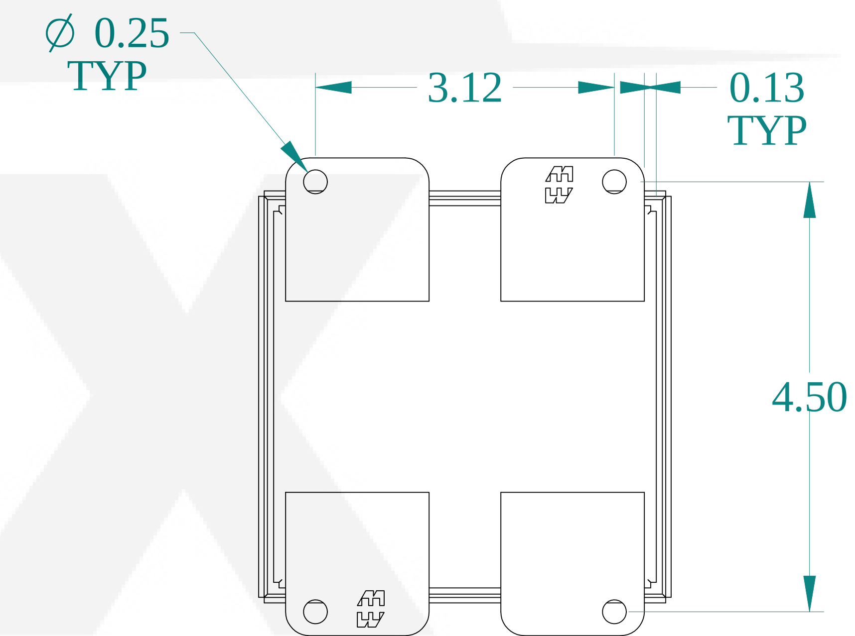
BACK VIEW
