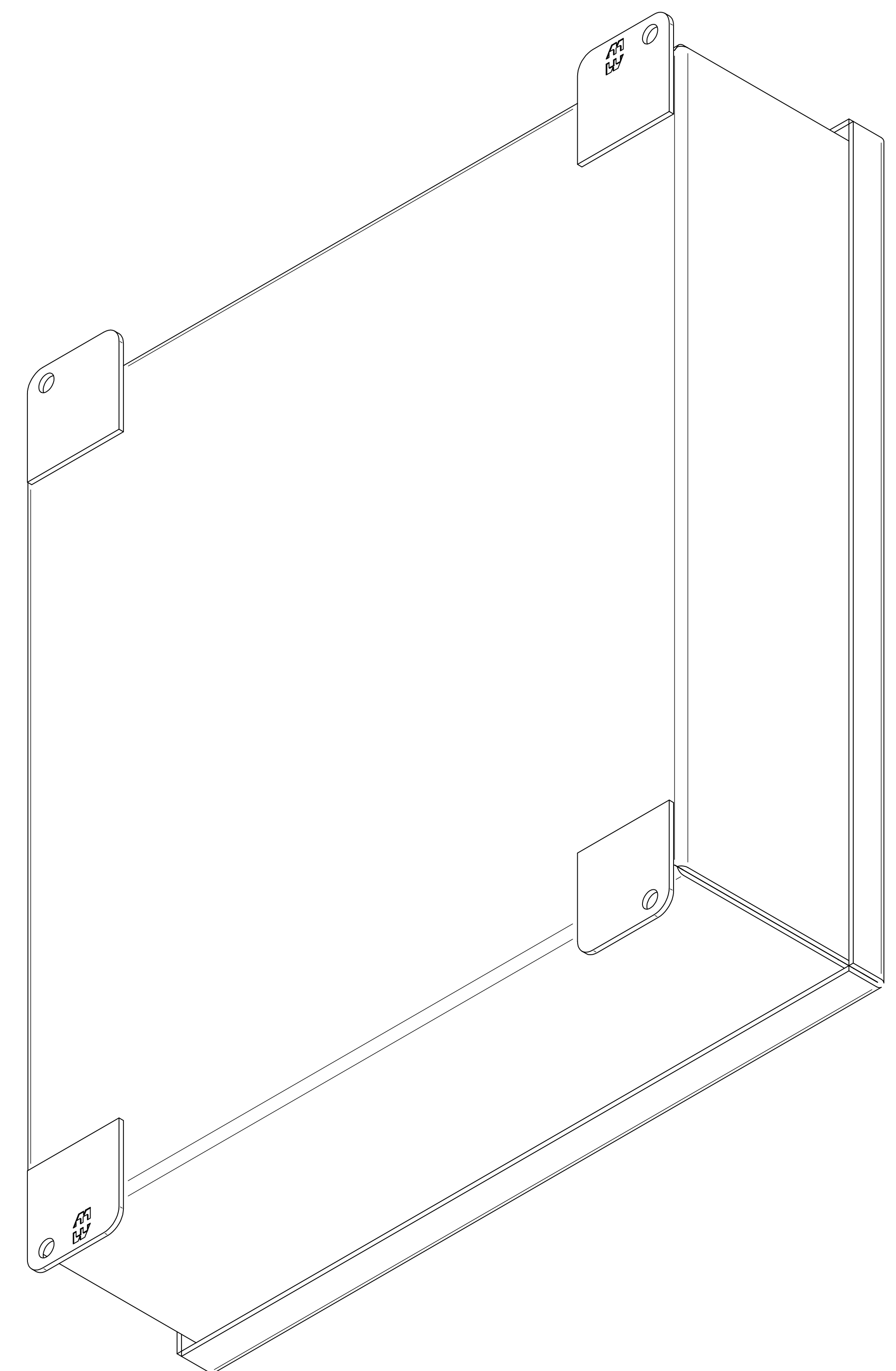
ISOMETRIC VIEWS
