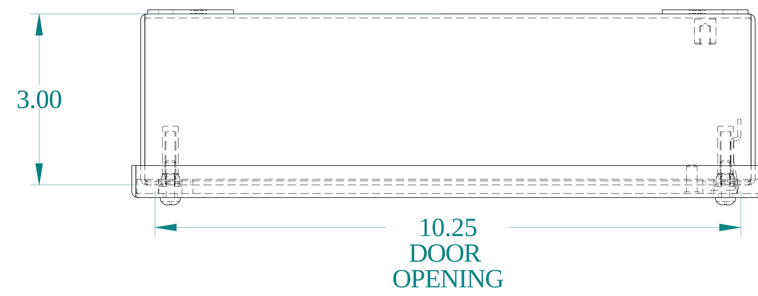
TOP VIEW
