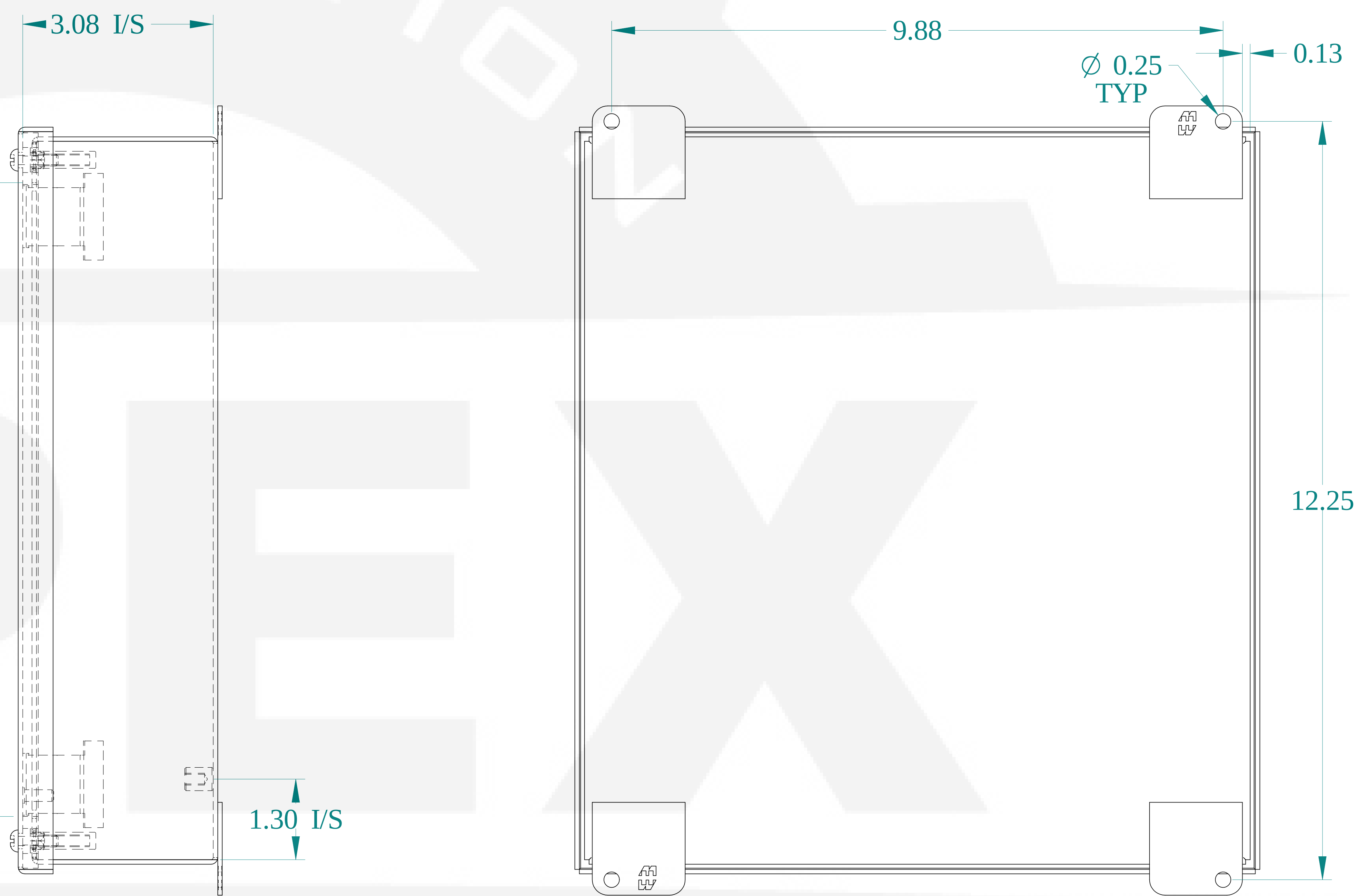
BACK VIEW
