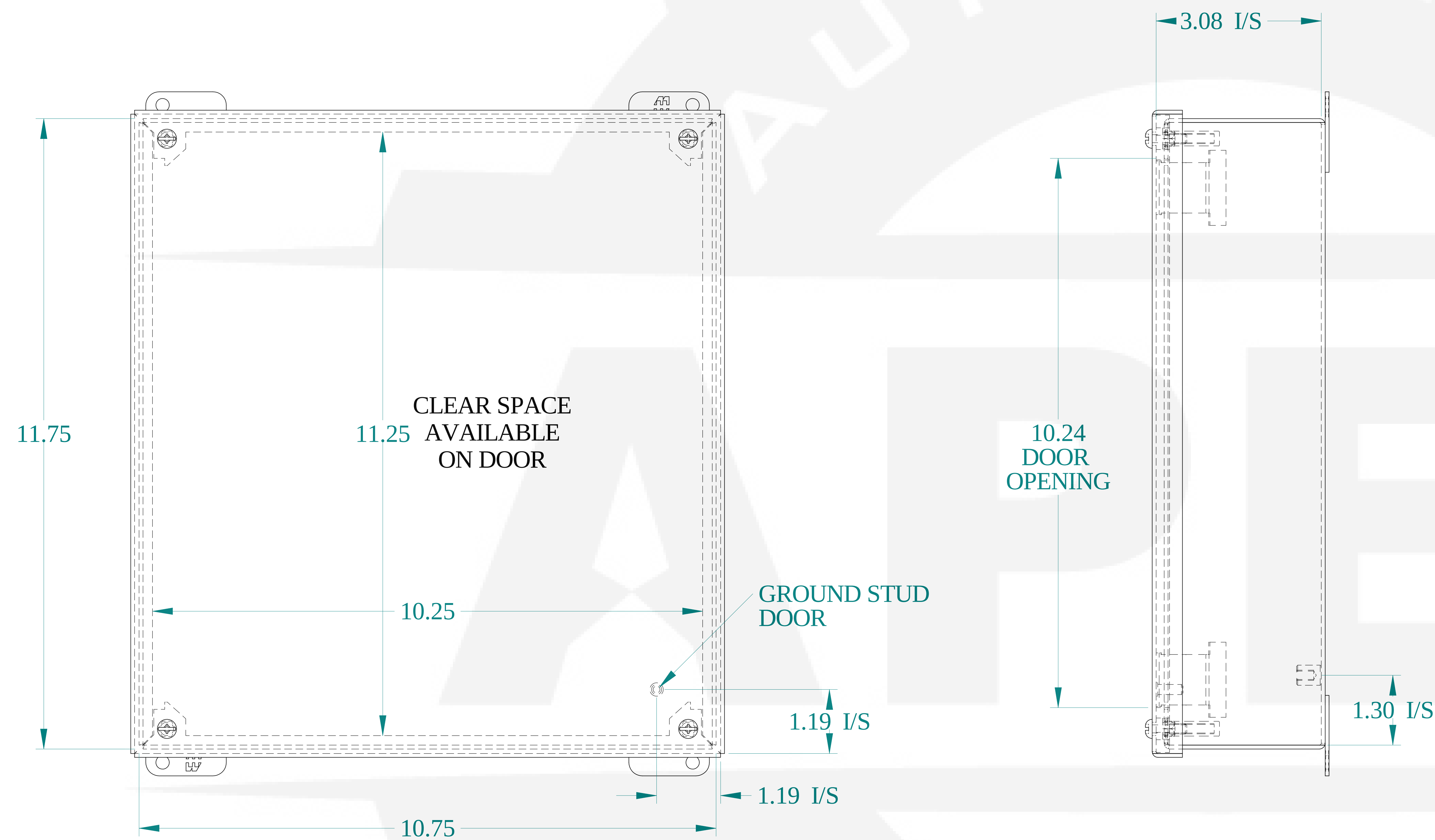
FRONT VIEW
