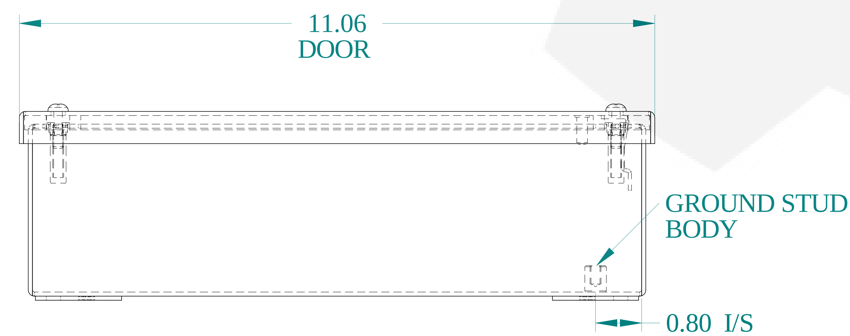
BOTTOM VIEW
