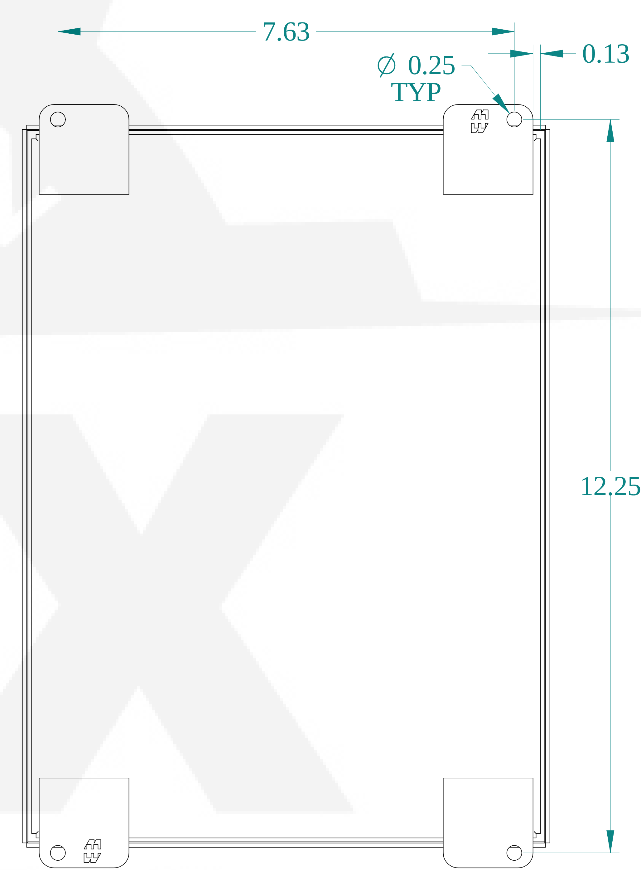
BACK VIEW
