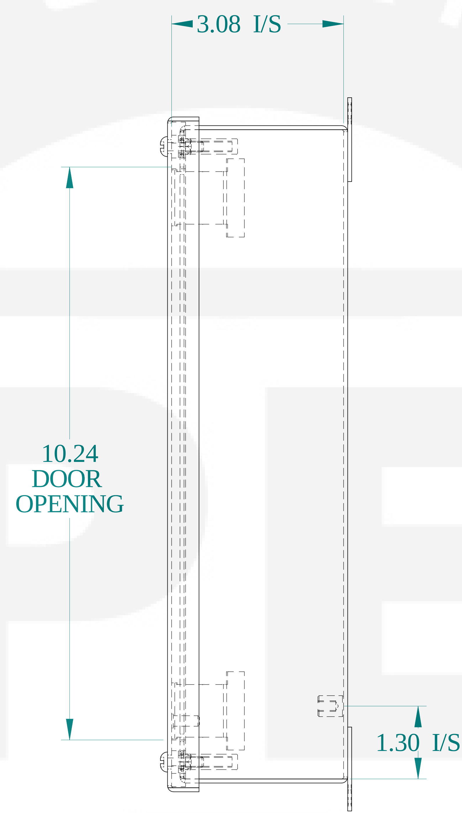
SIDE VIEW
