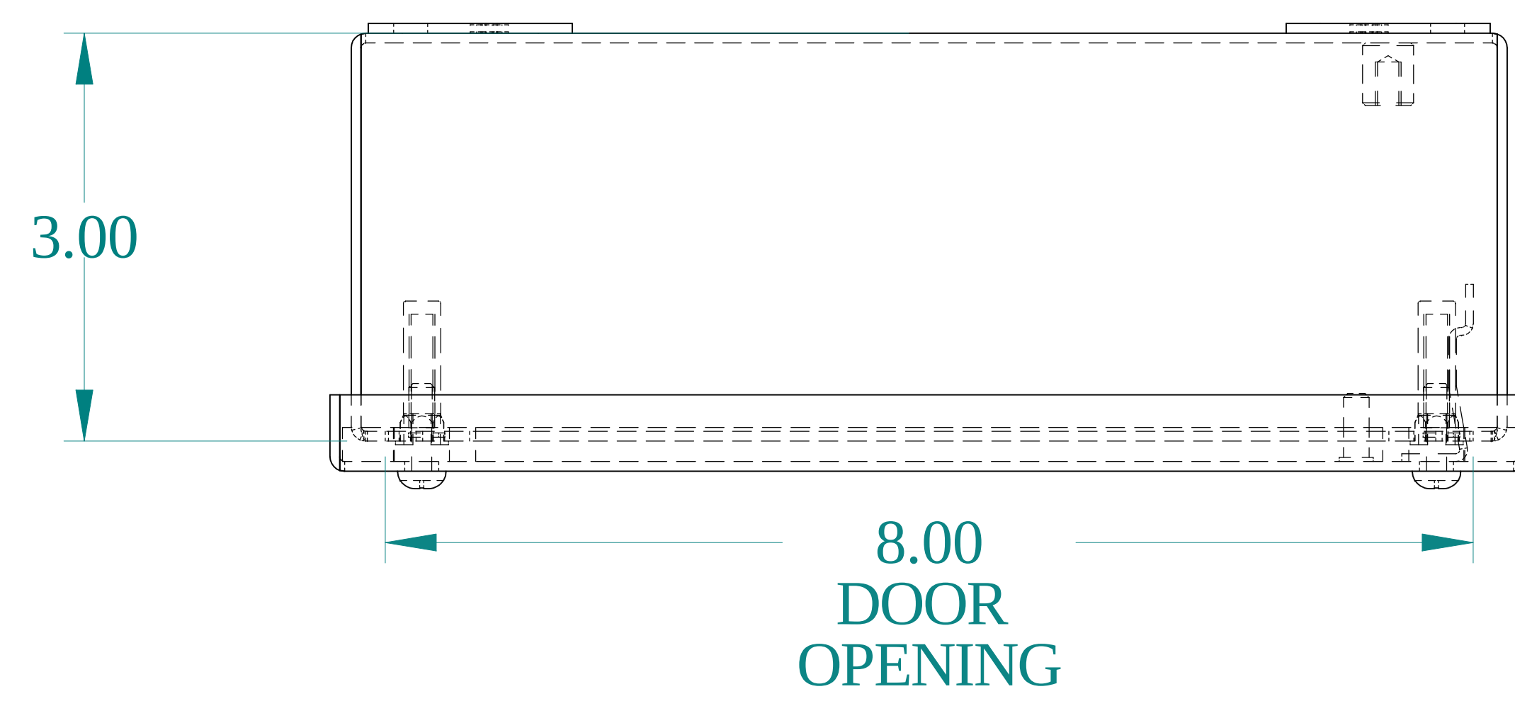
TOP VIEW
