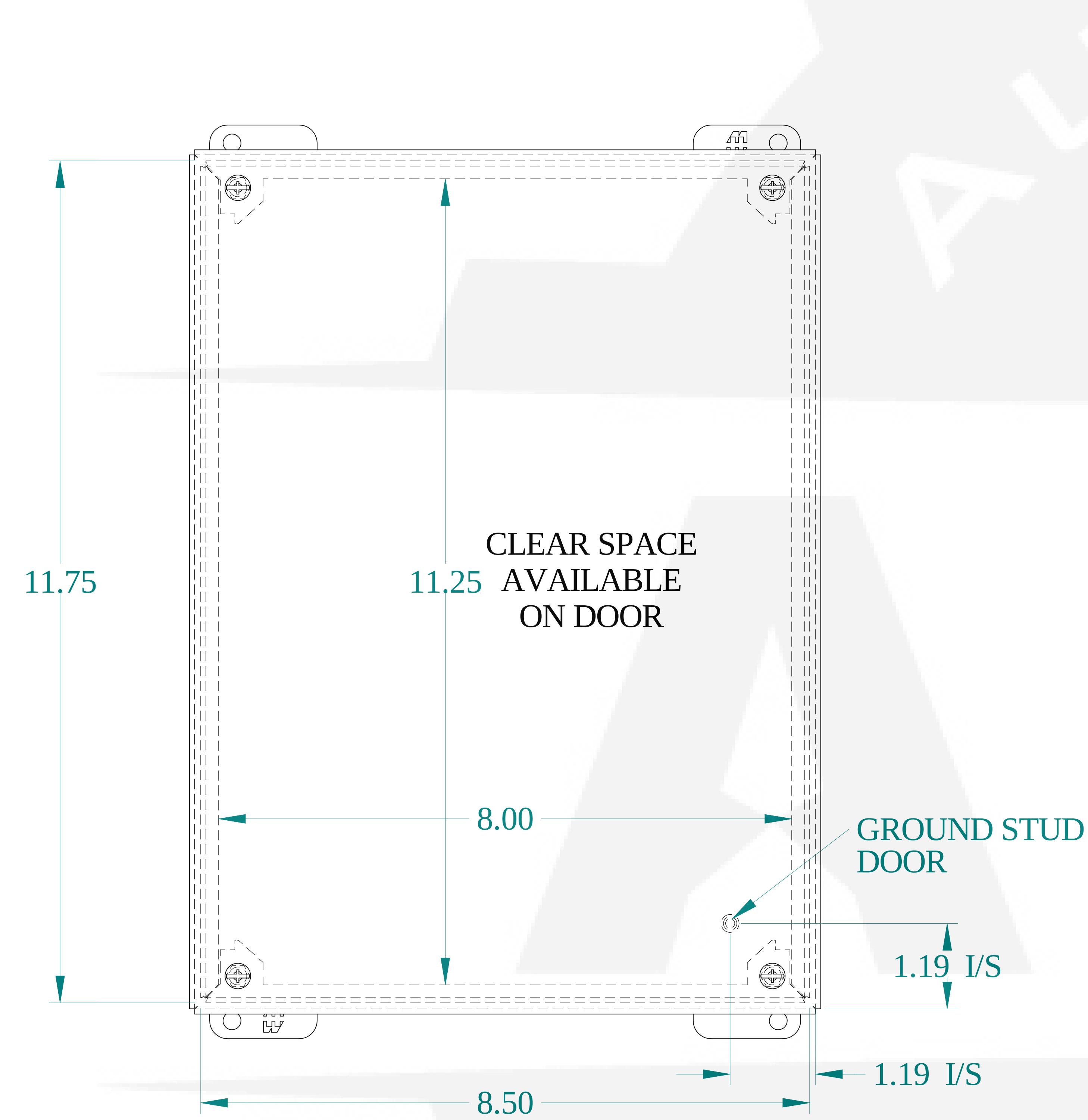
FRONT VIEW
