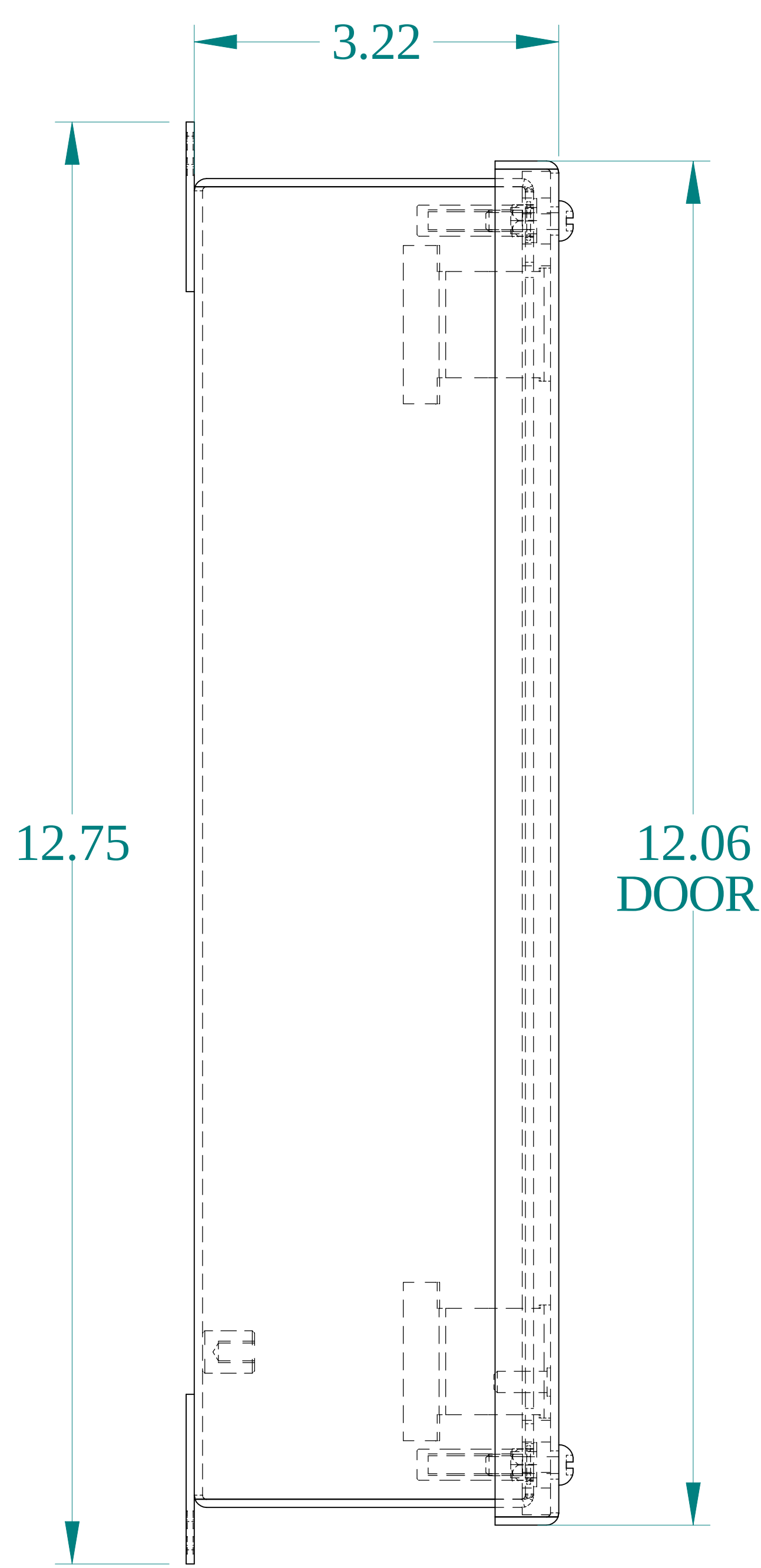
SIDE VIEW
