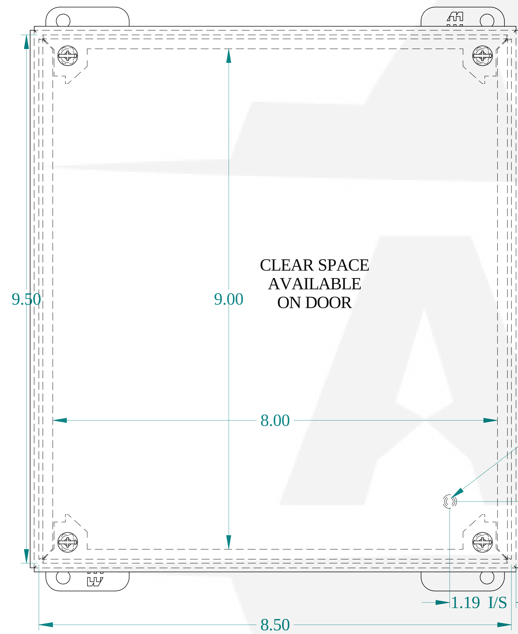
FRONT VIEW
