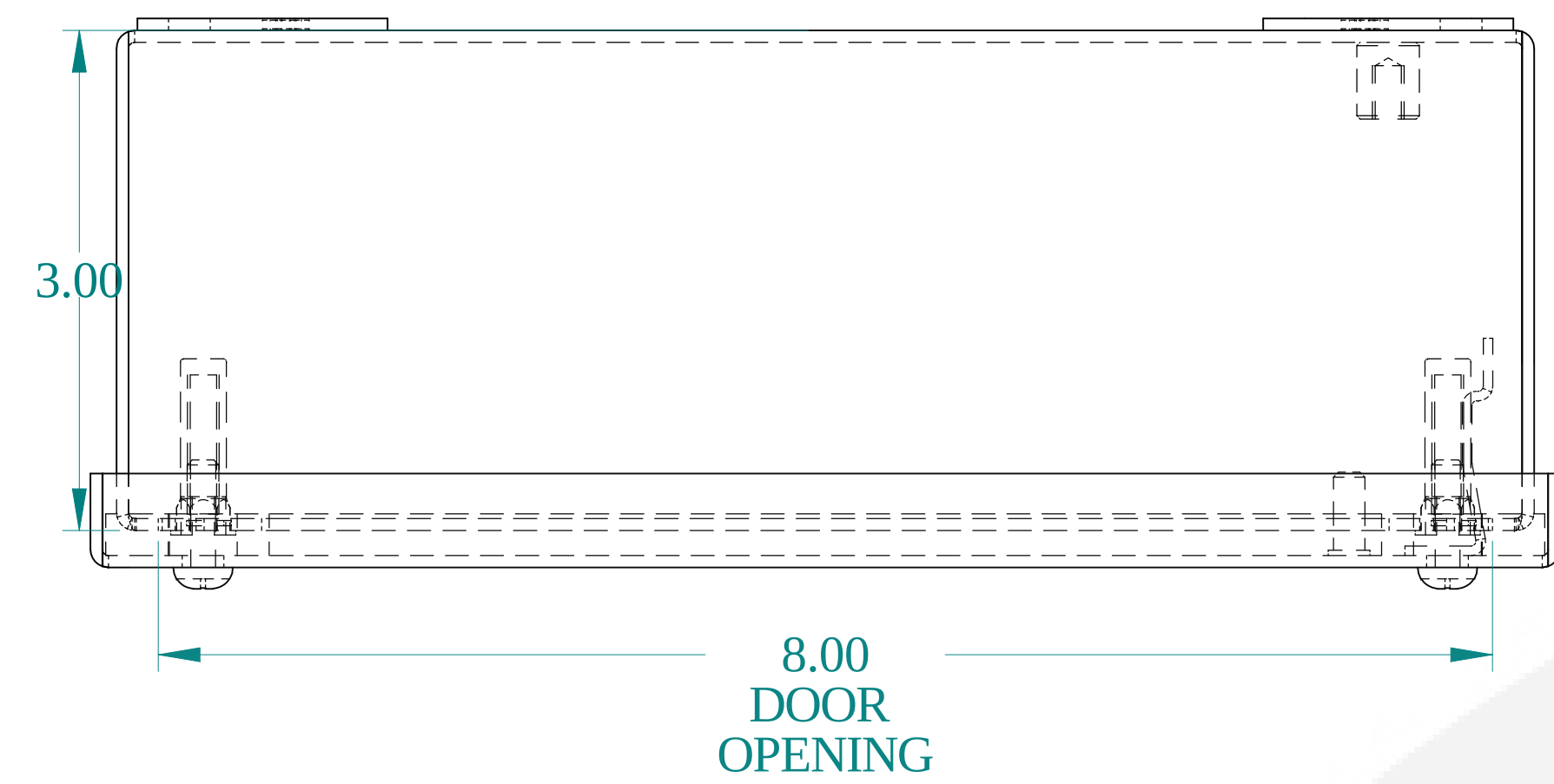
TOP VIEW
