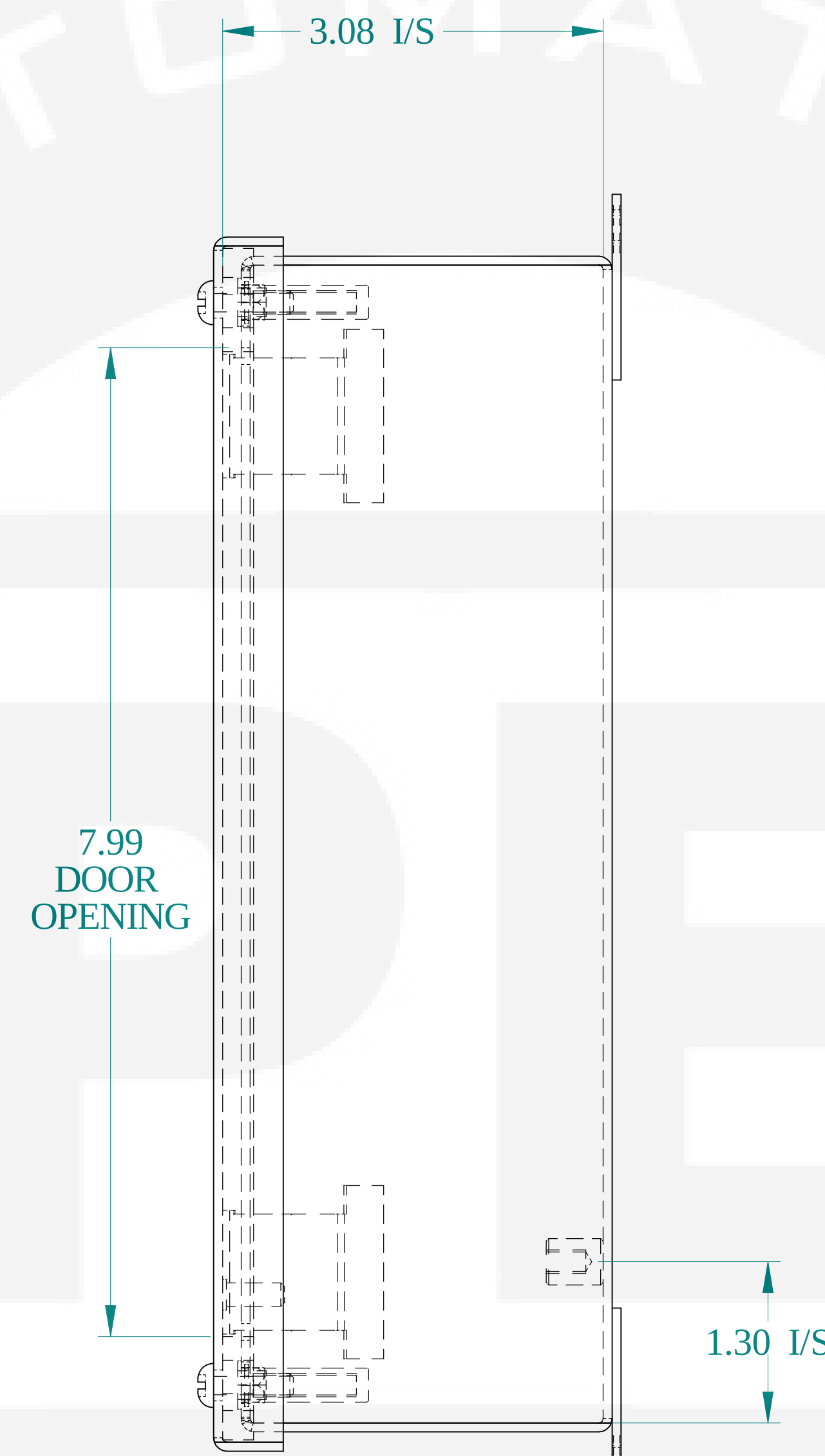
SIDE VIEW
