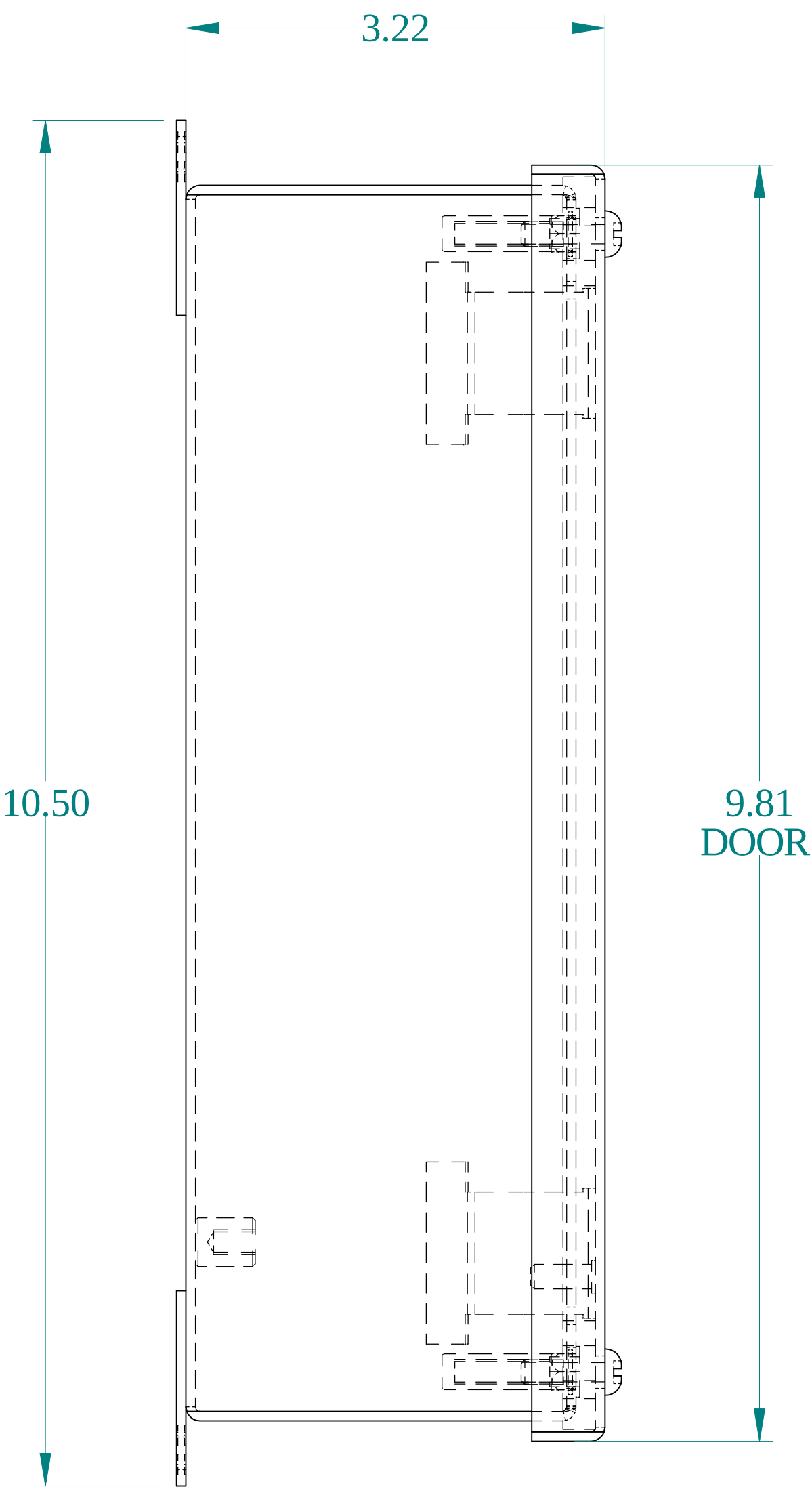
SIDE VIEW
