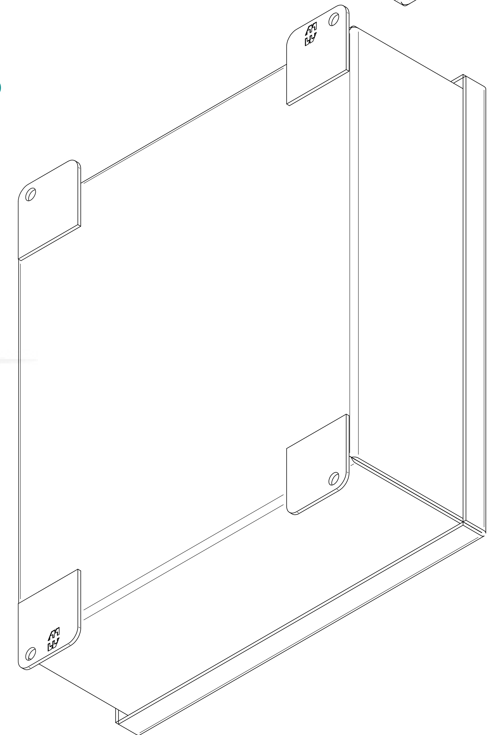
ISOMETRIC VIEWS
