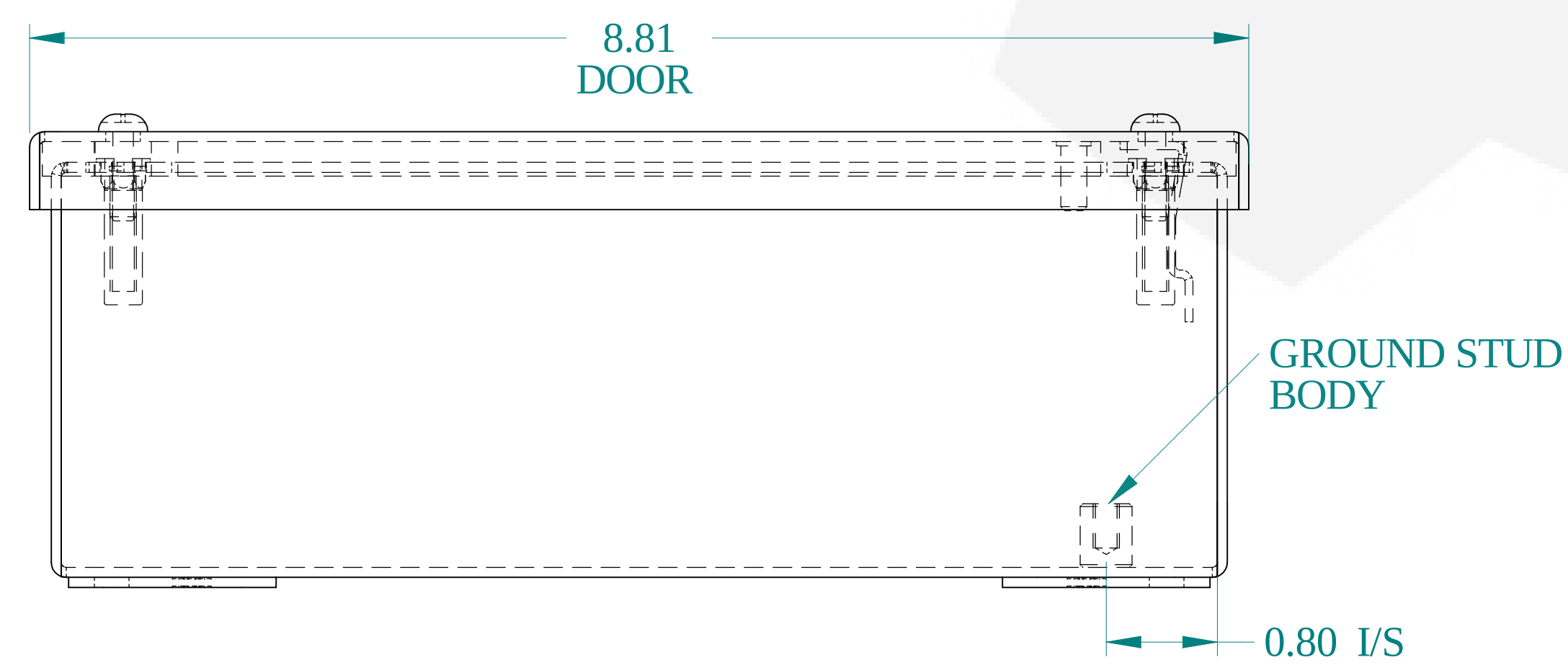
BOTTOM VIEW
