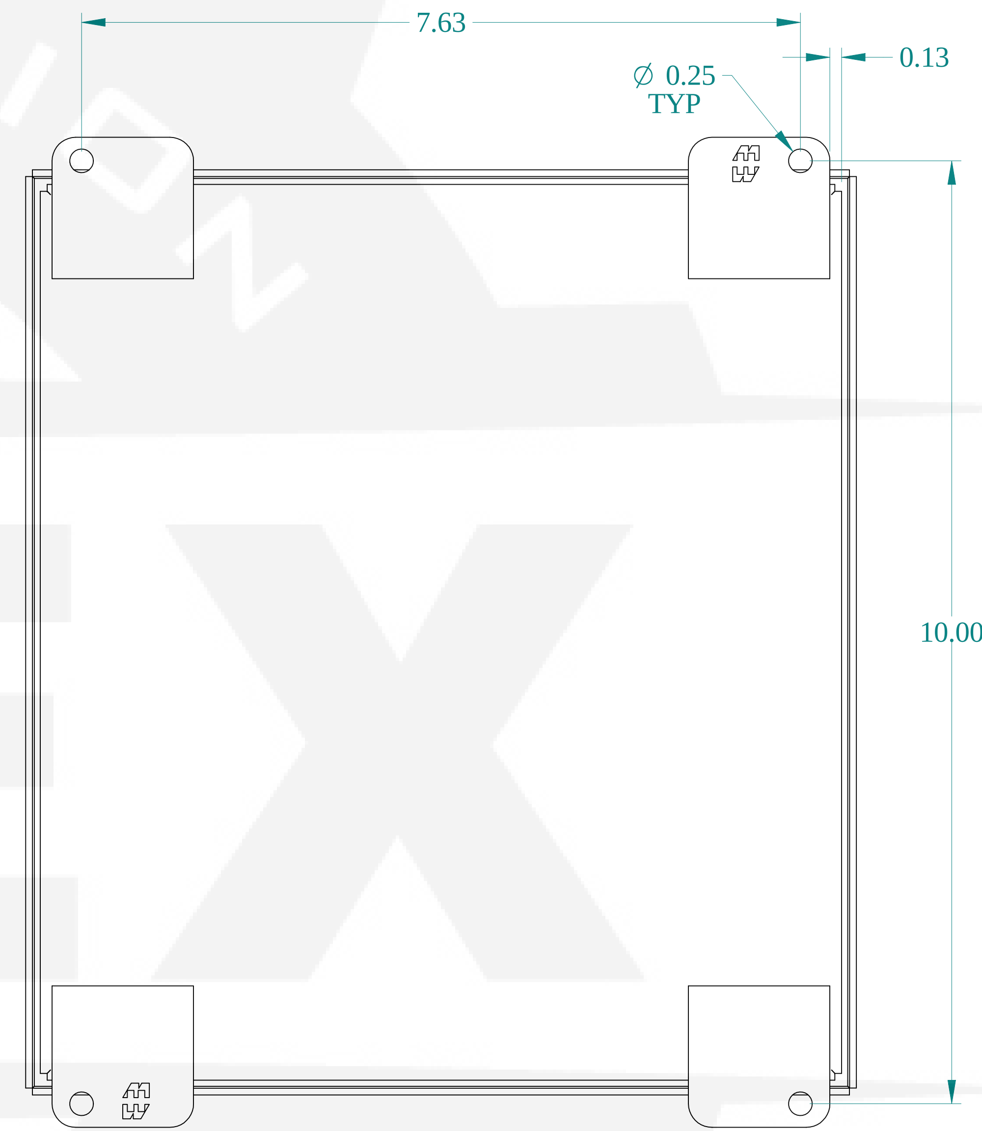
BACK VIEW
