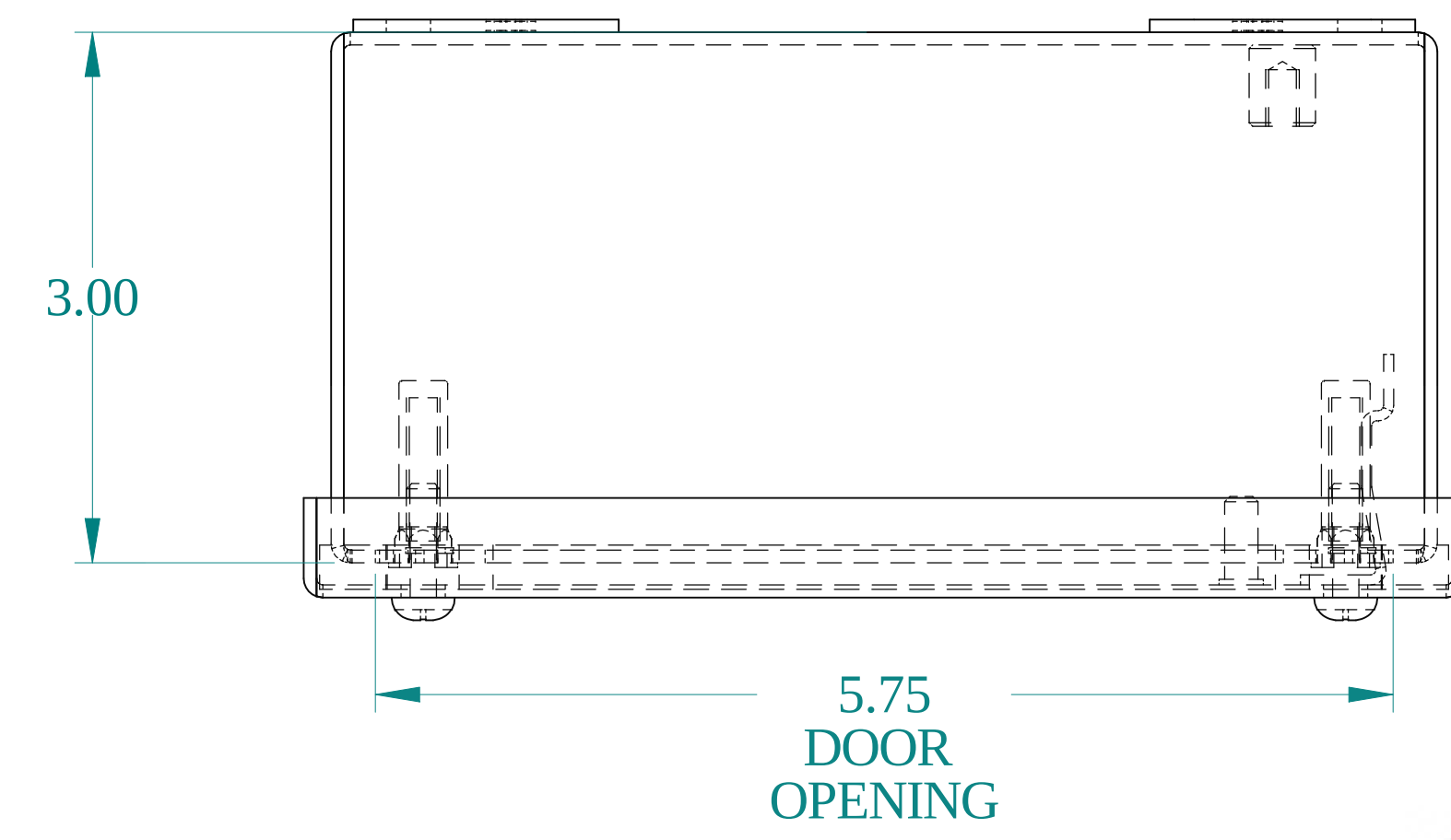
TOP VIEW
