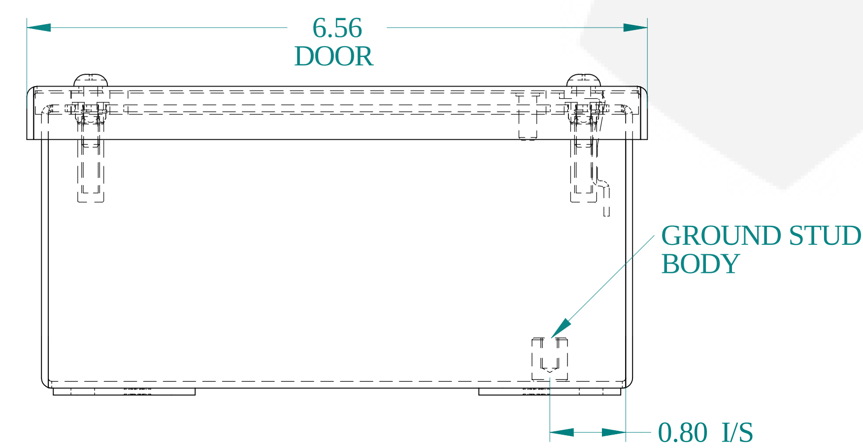
BOTTOM VIEW
