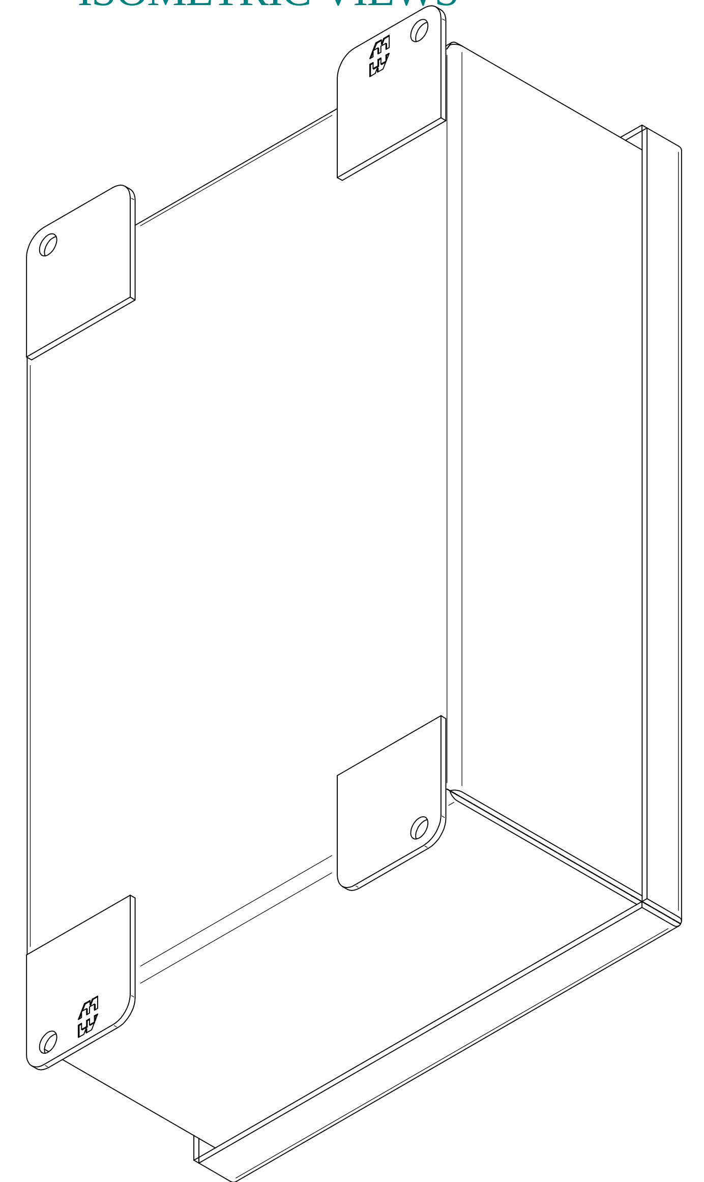
ISOMETRIC VIEWS
