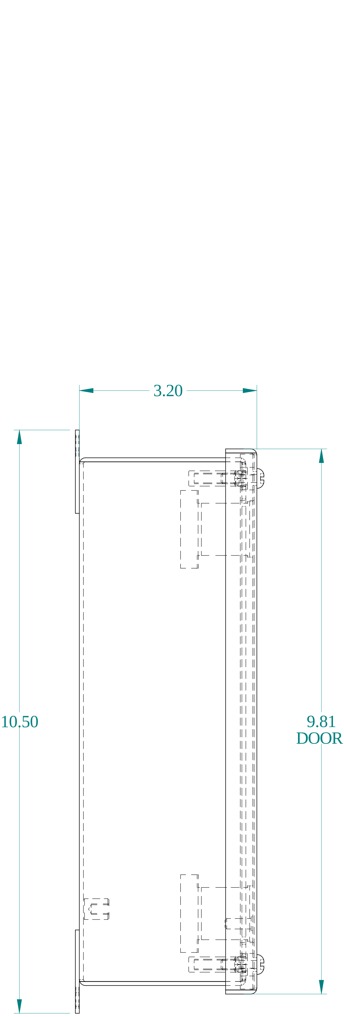
SIDE VIEW
