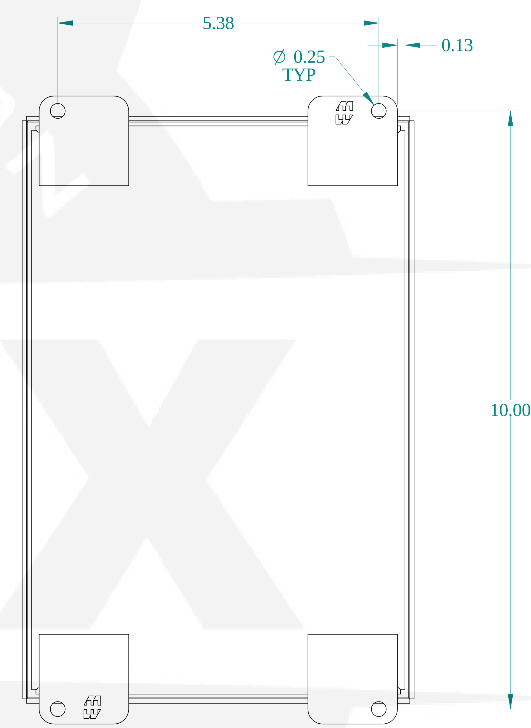
BACK VIEW
