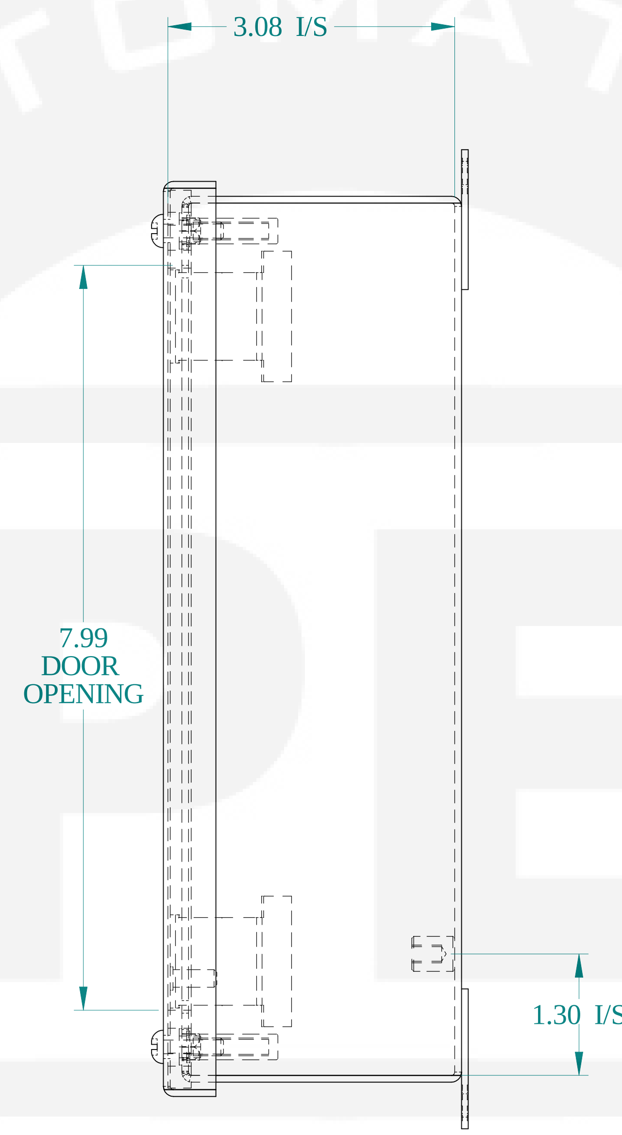
SIDE VIEW
