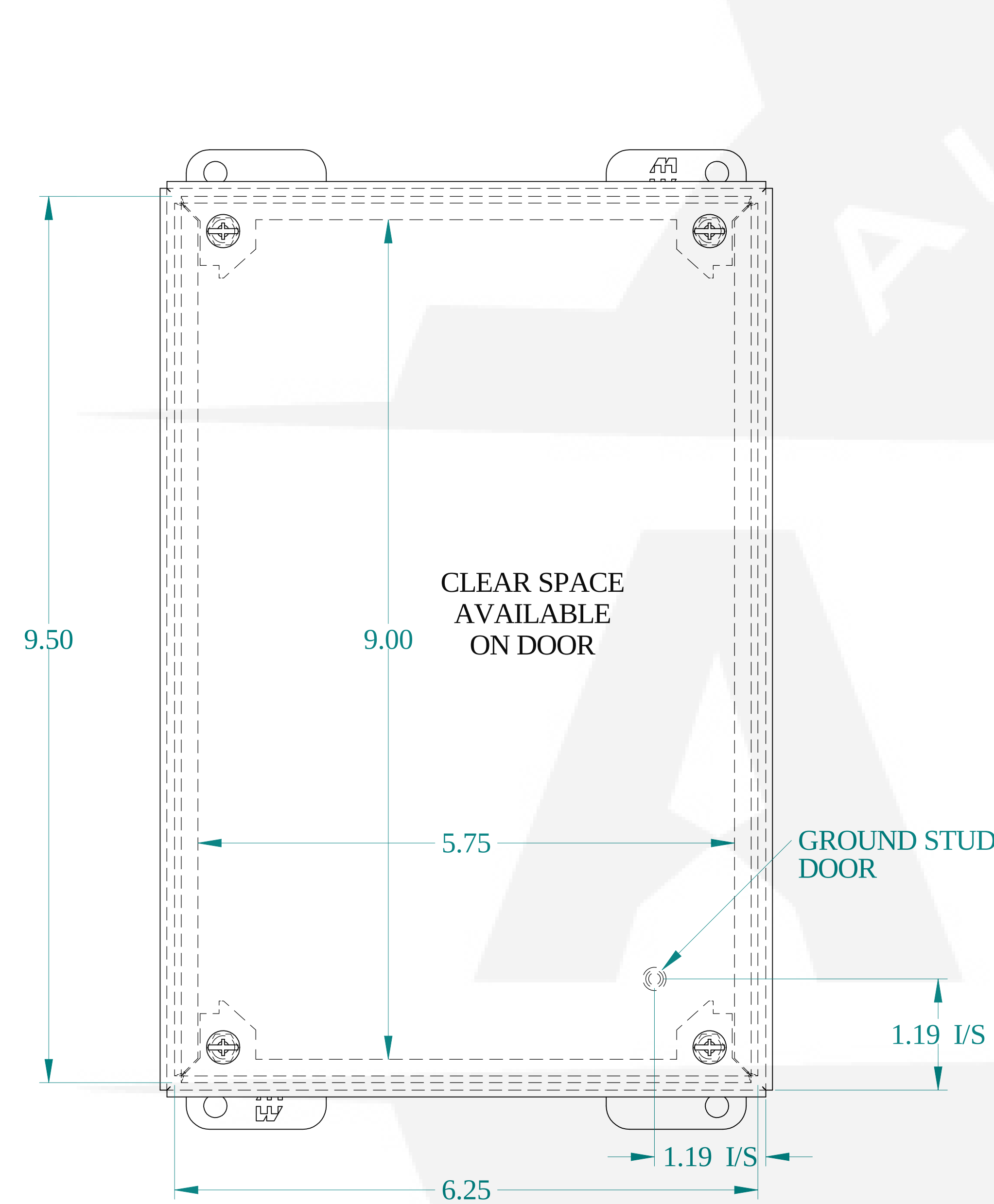
FRONT VIEW
