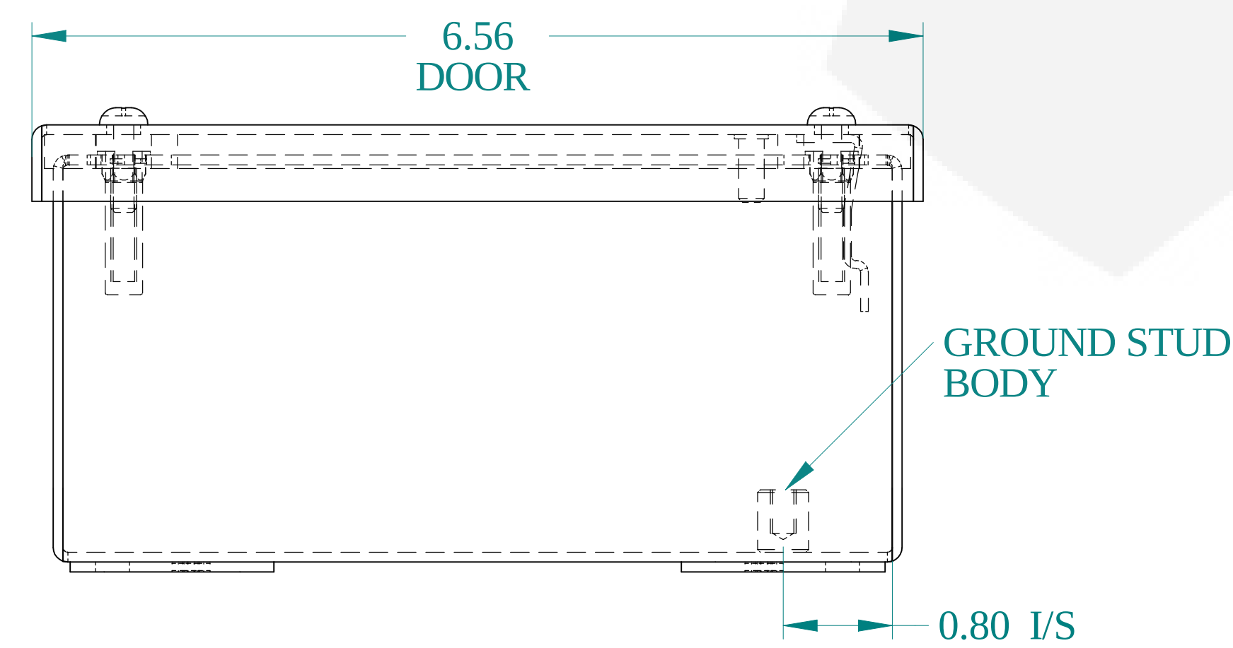
BOTTOM VIEW
