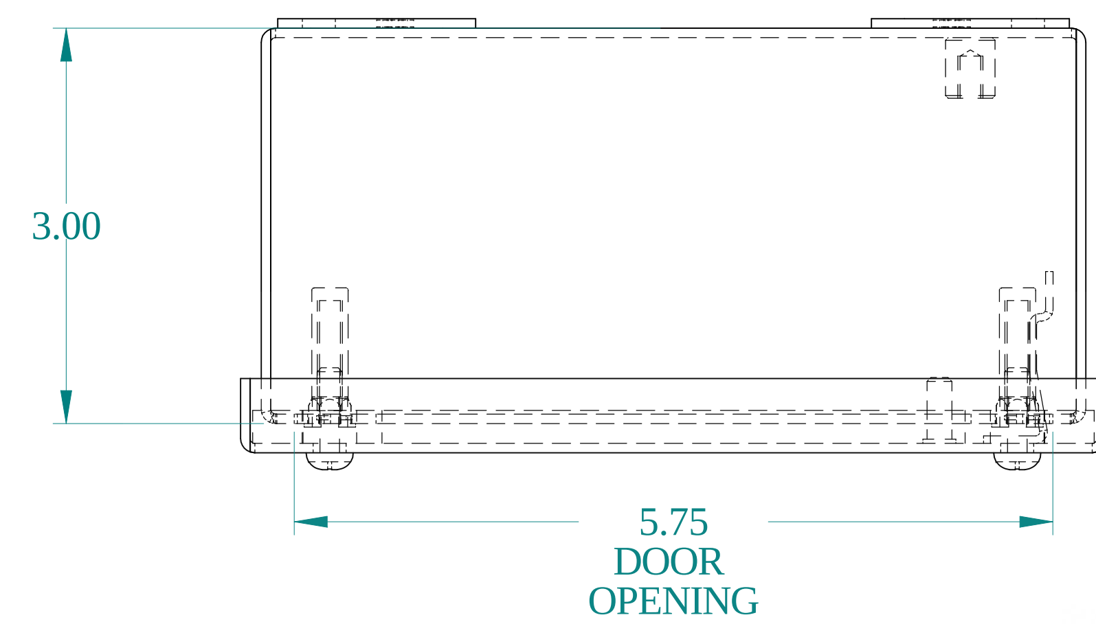
TOP VIEW
