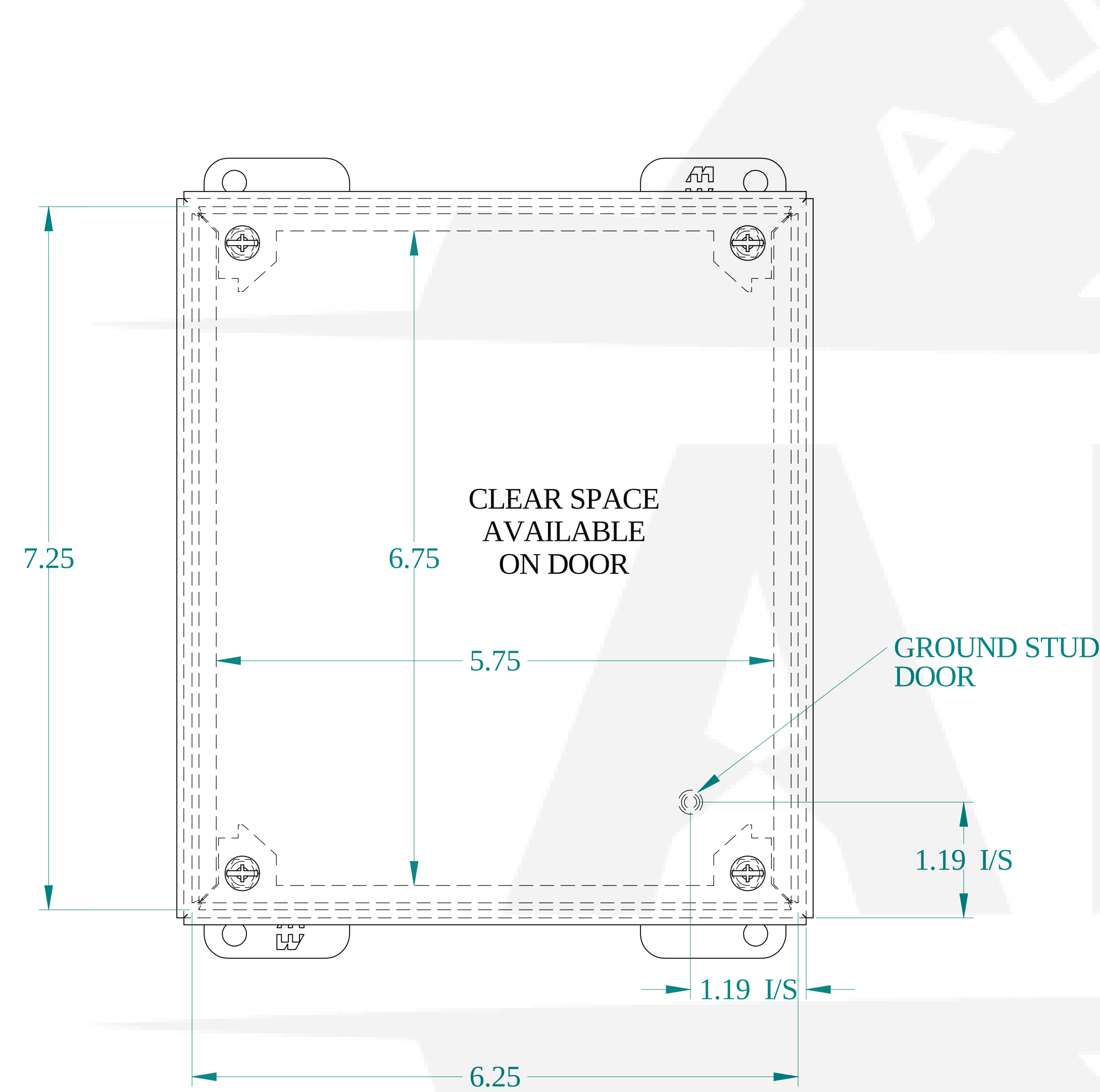
FRONT VIEW
