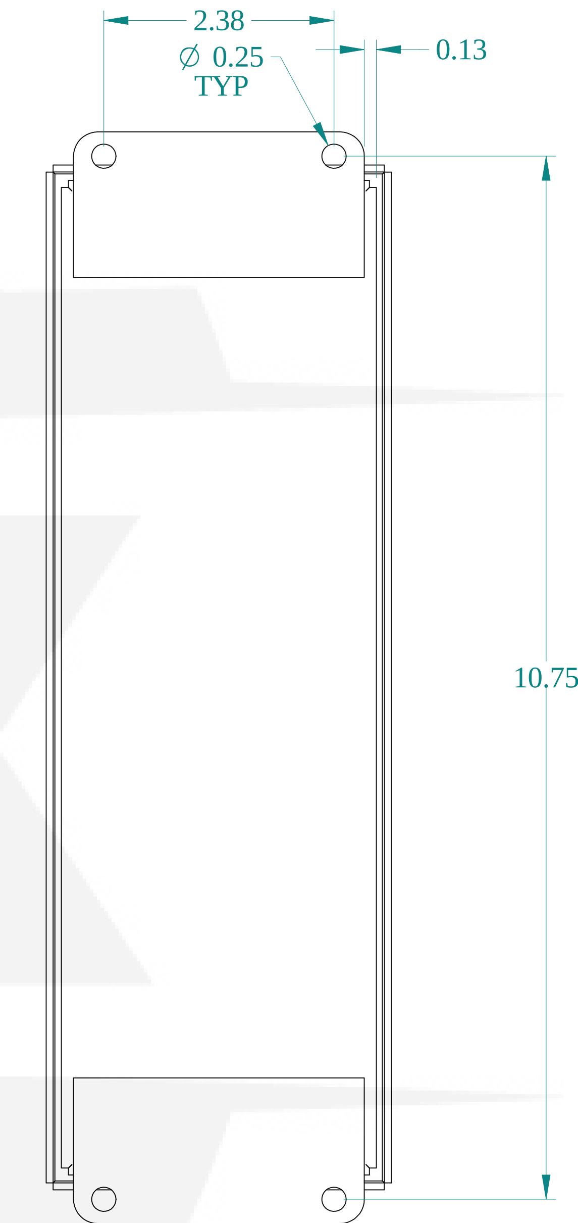
BACK VIEW
