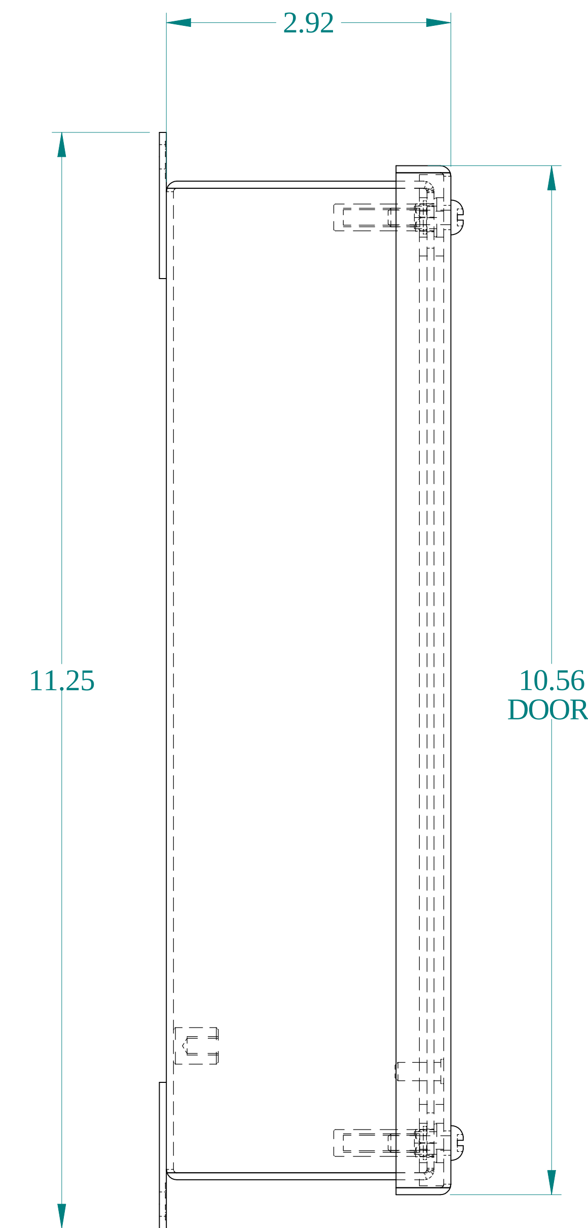
SIDE VIEW
