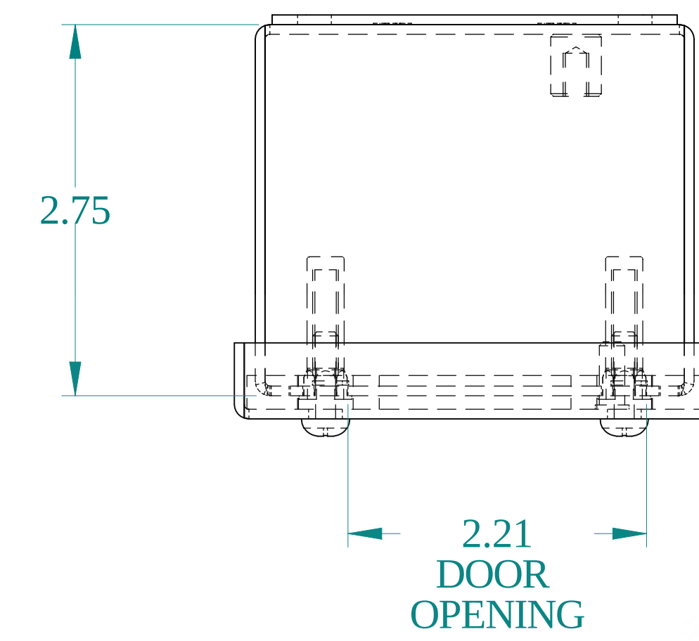
TOP VIEW
