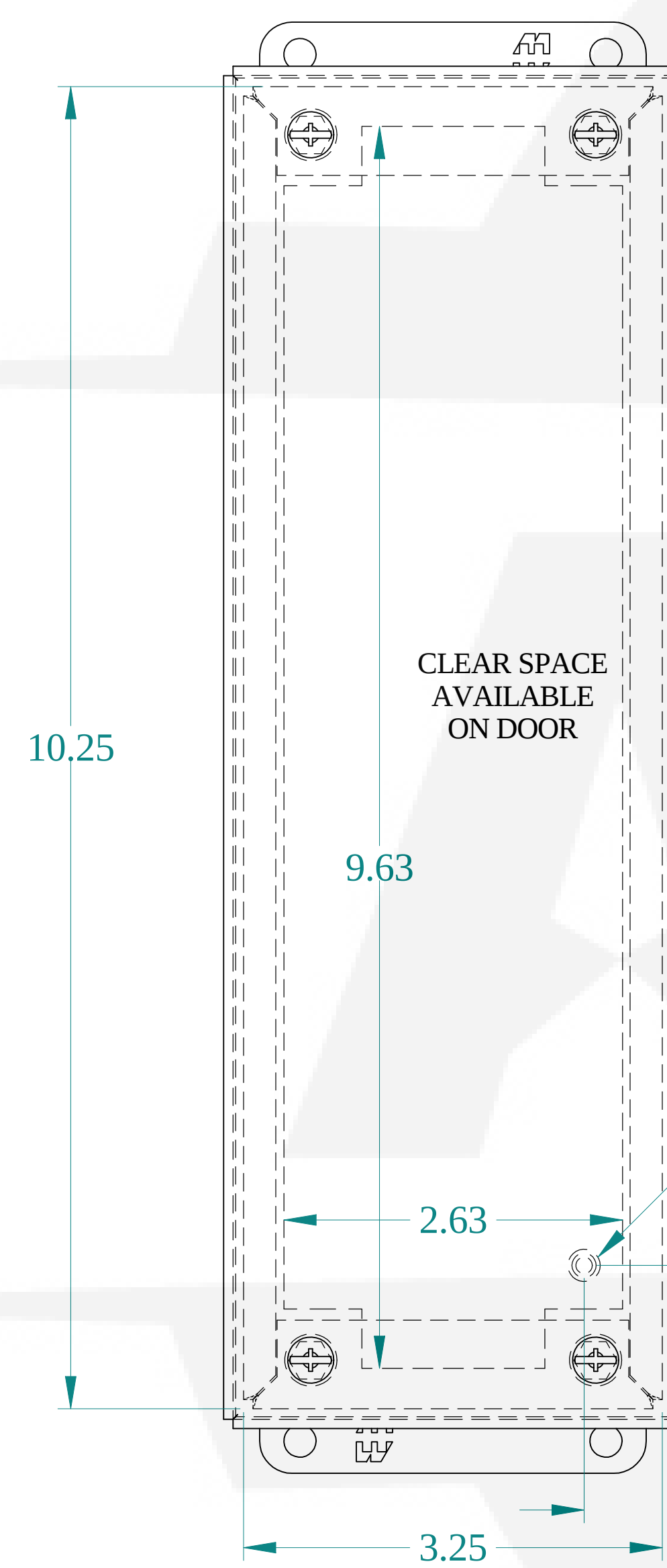
FRONT VIEW
