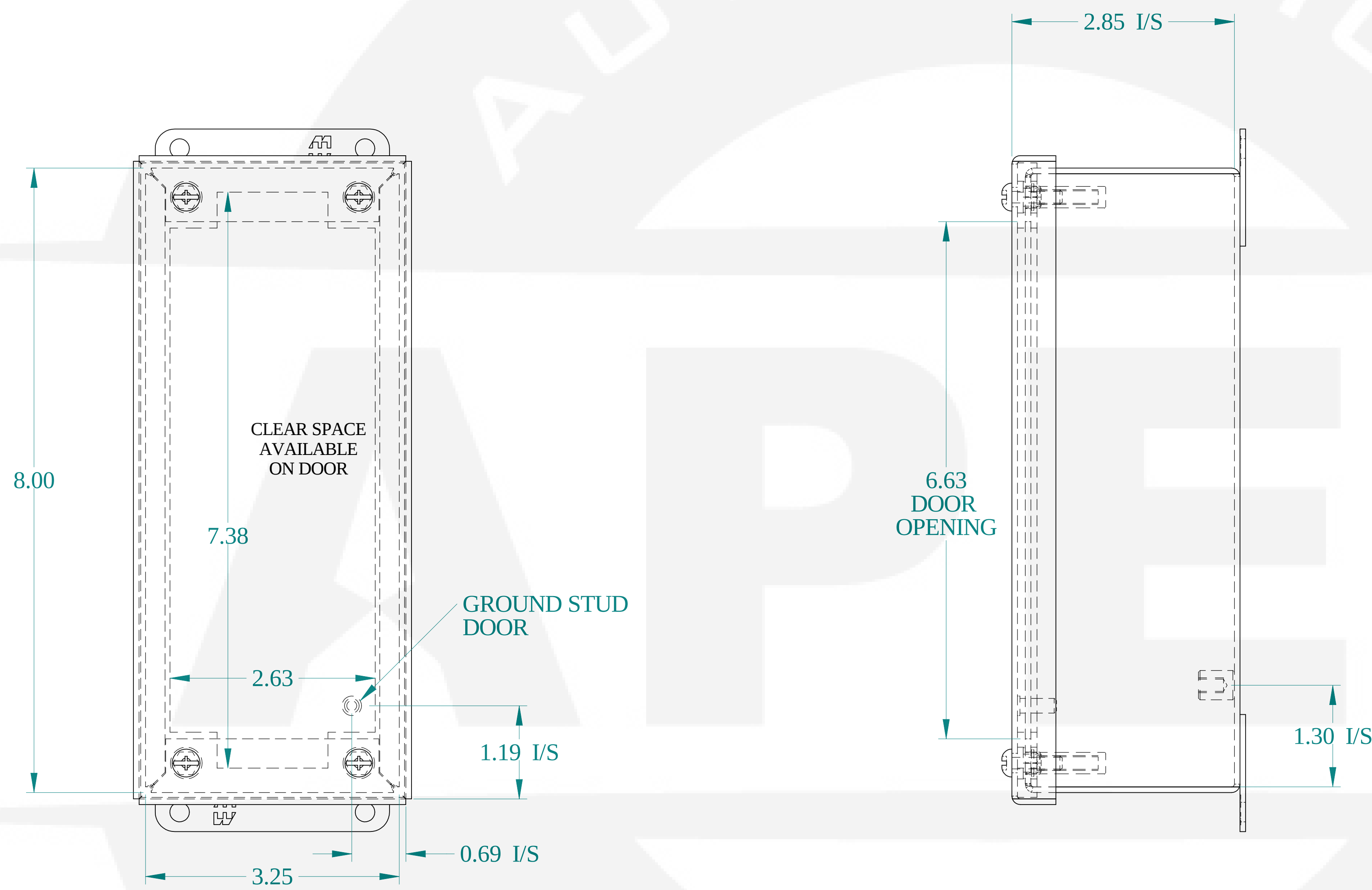
FRONT VIEW
