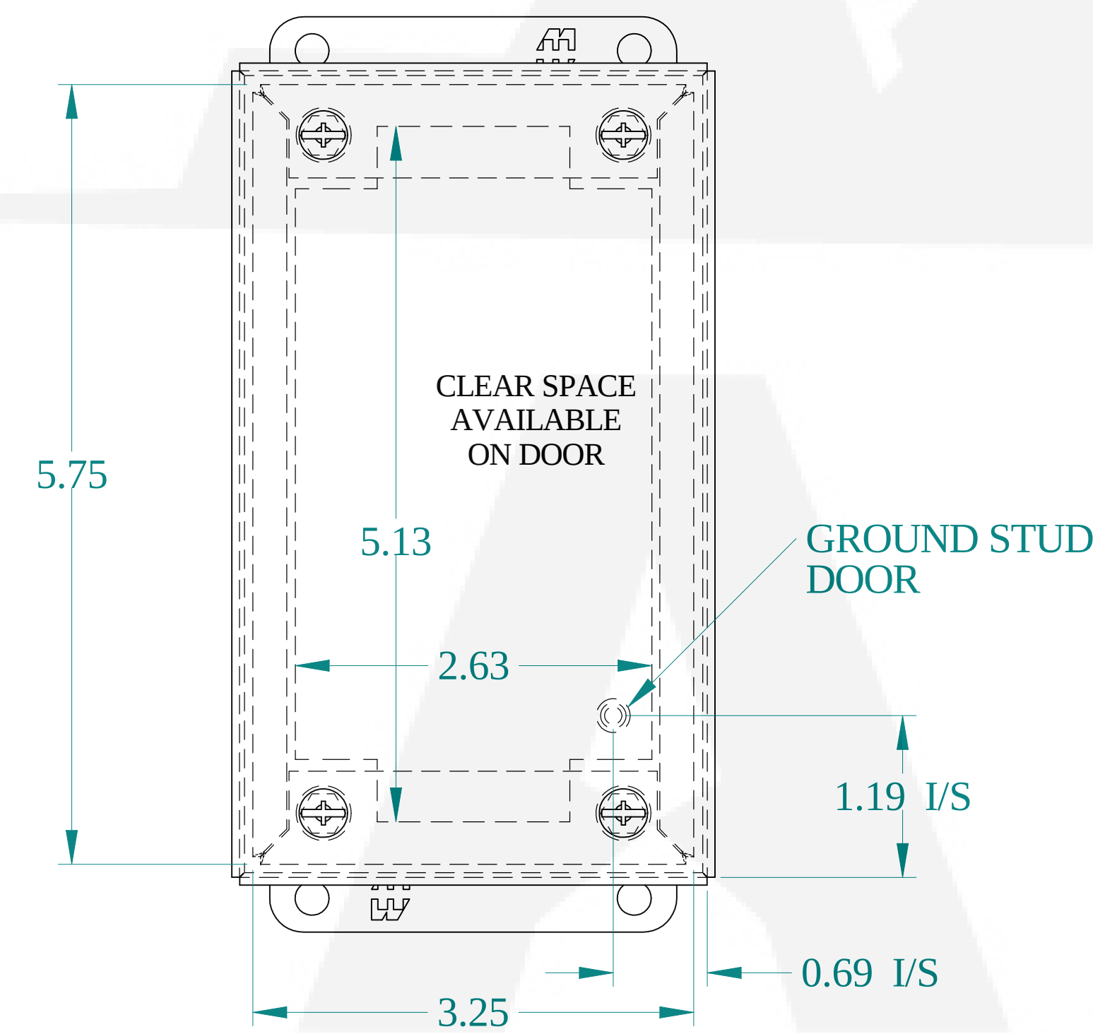
FRONT VIEW
