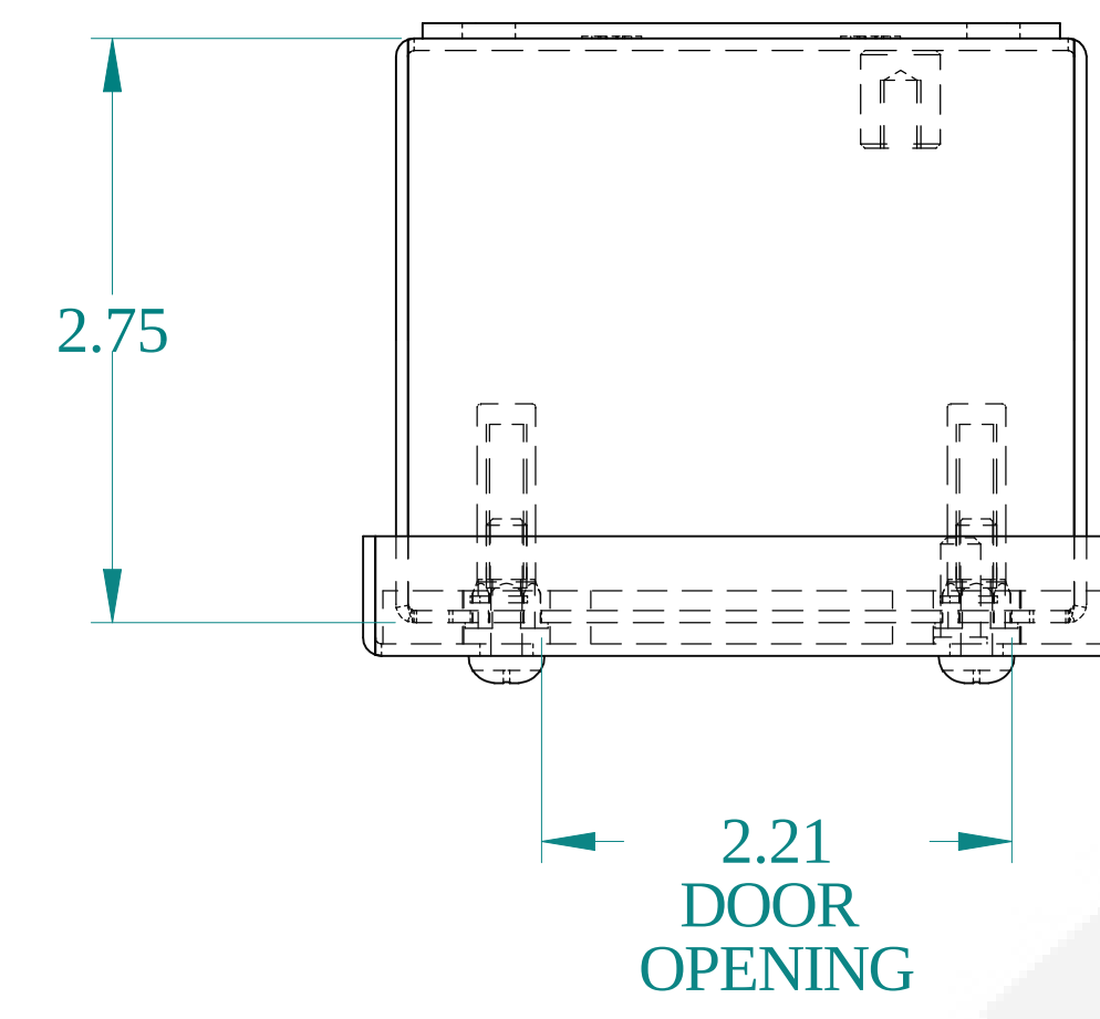
TOP VIEW
