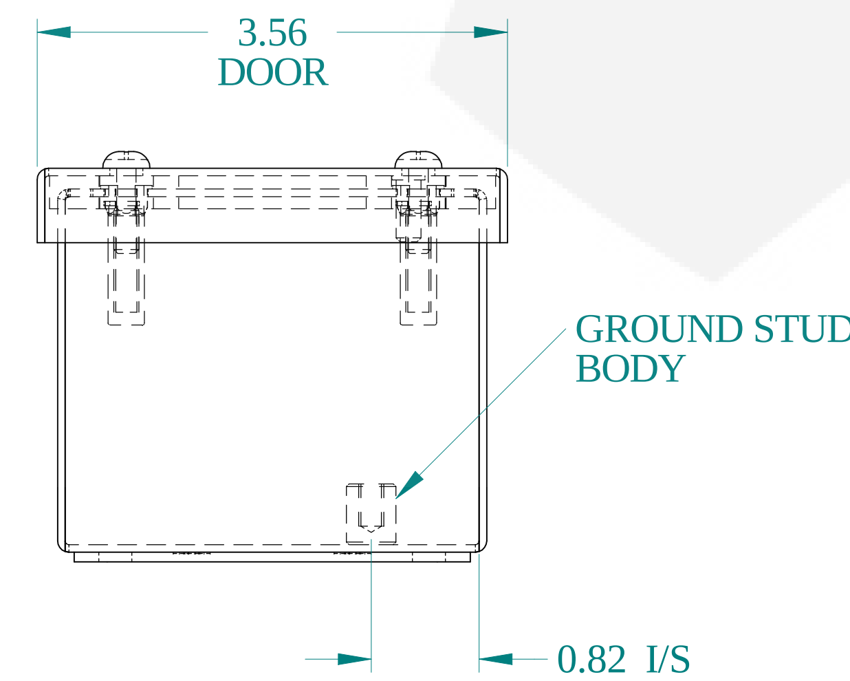
BOTTOM VIEW
