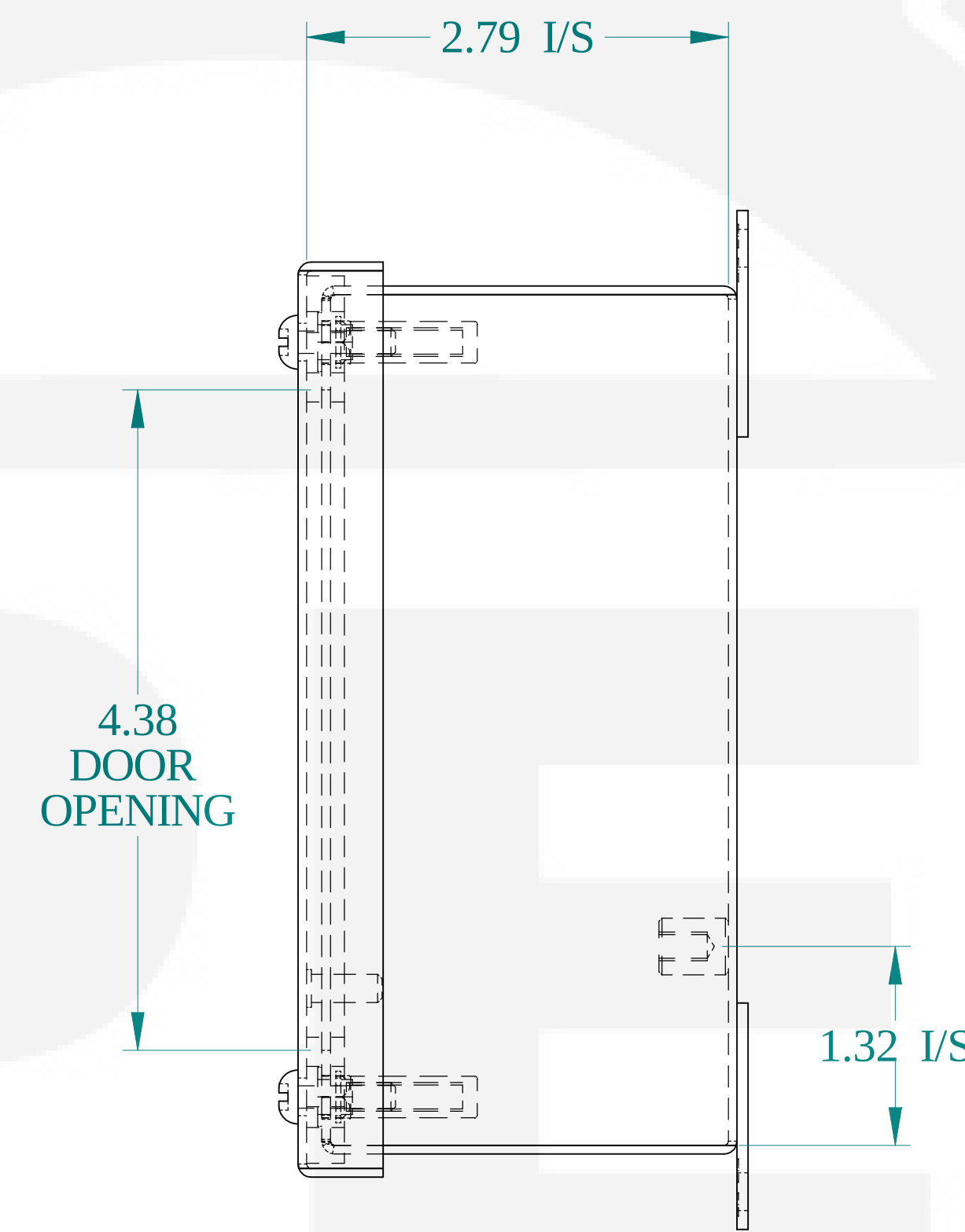
SIDE VIEW
