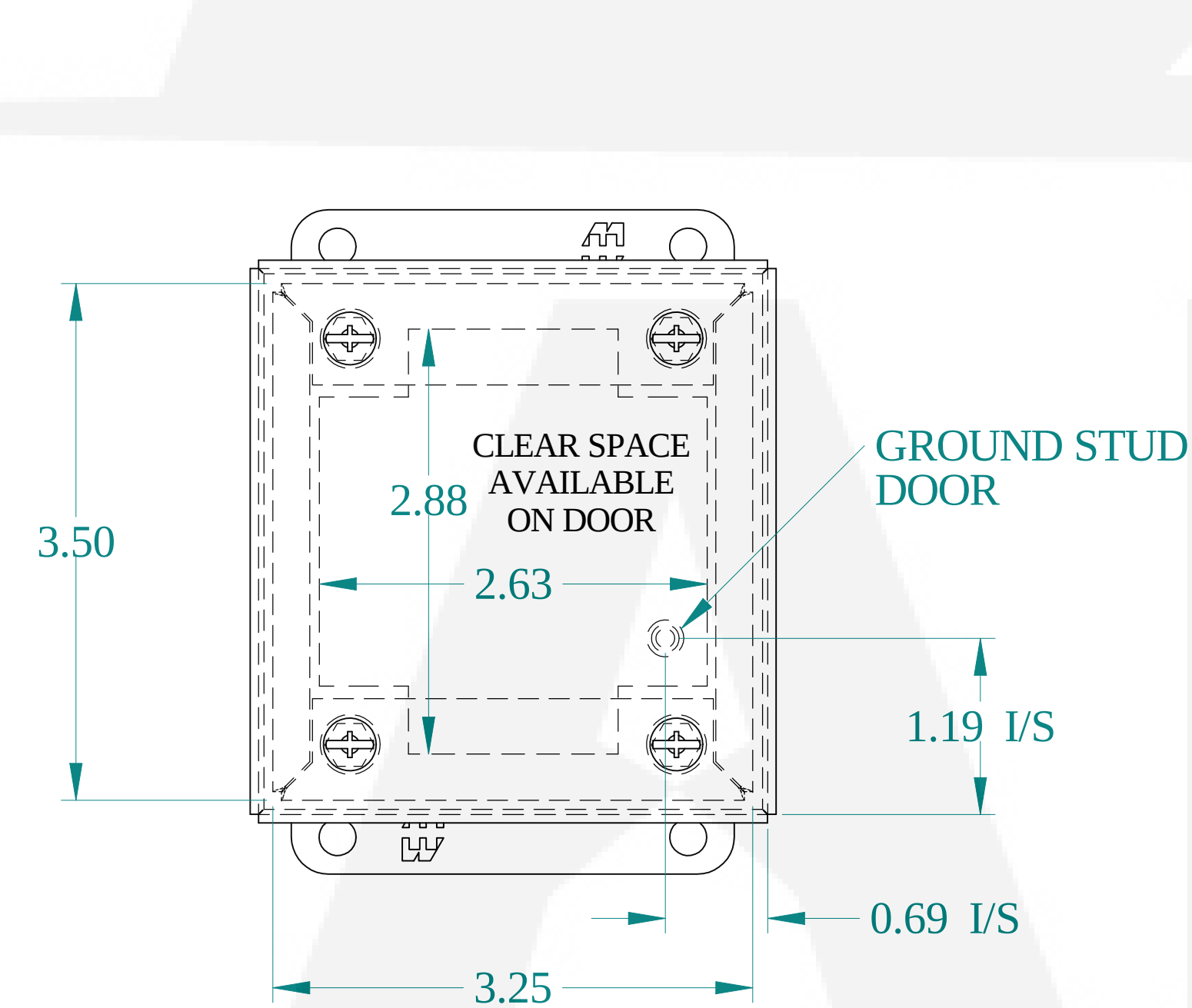
FRONT VIEW
