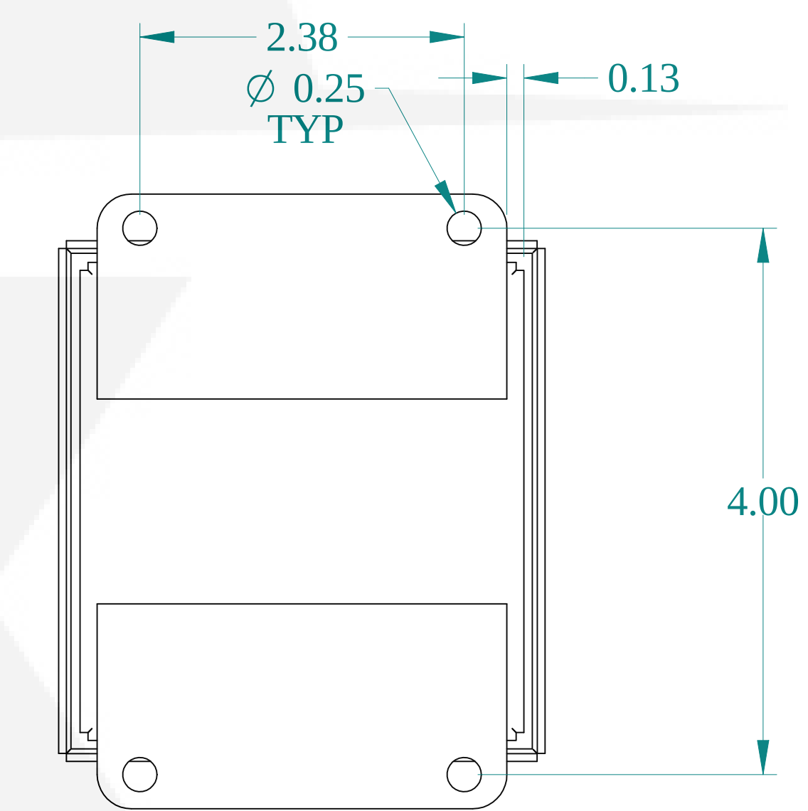
BACK VIEW
