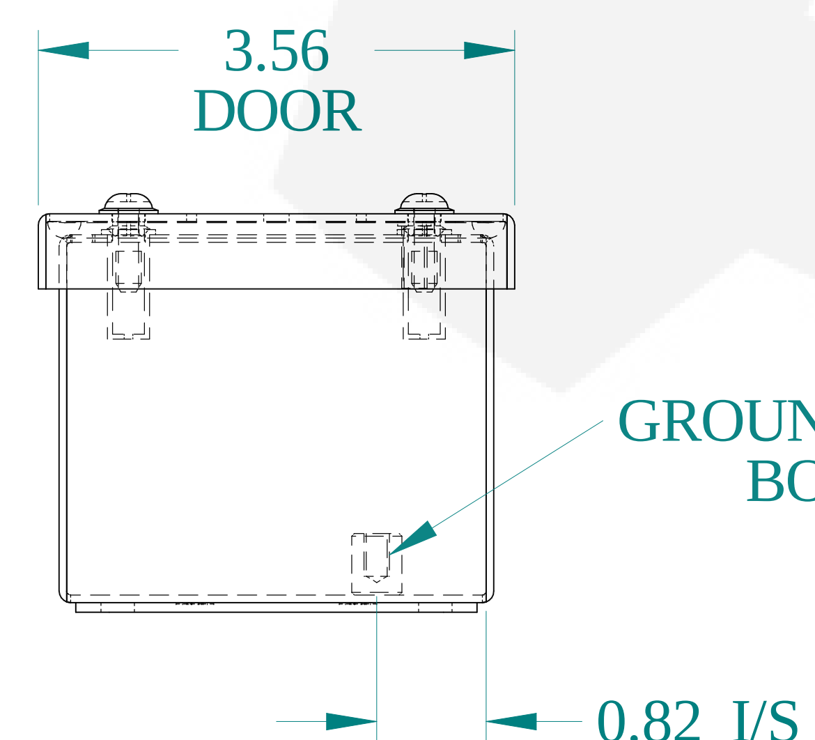
BOTTOM VIEW
