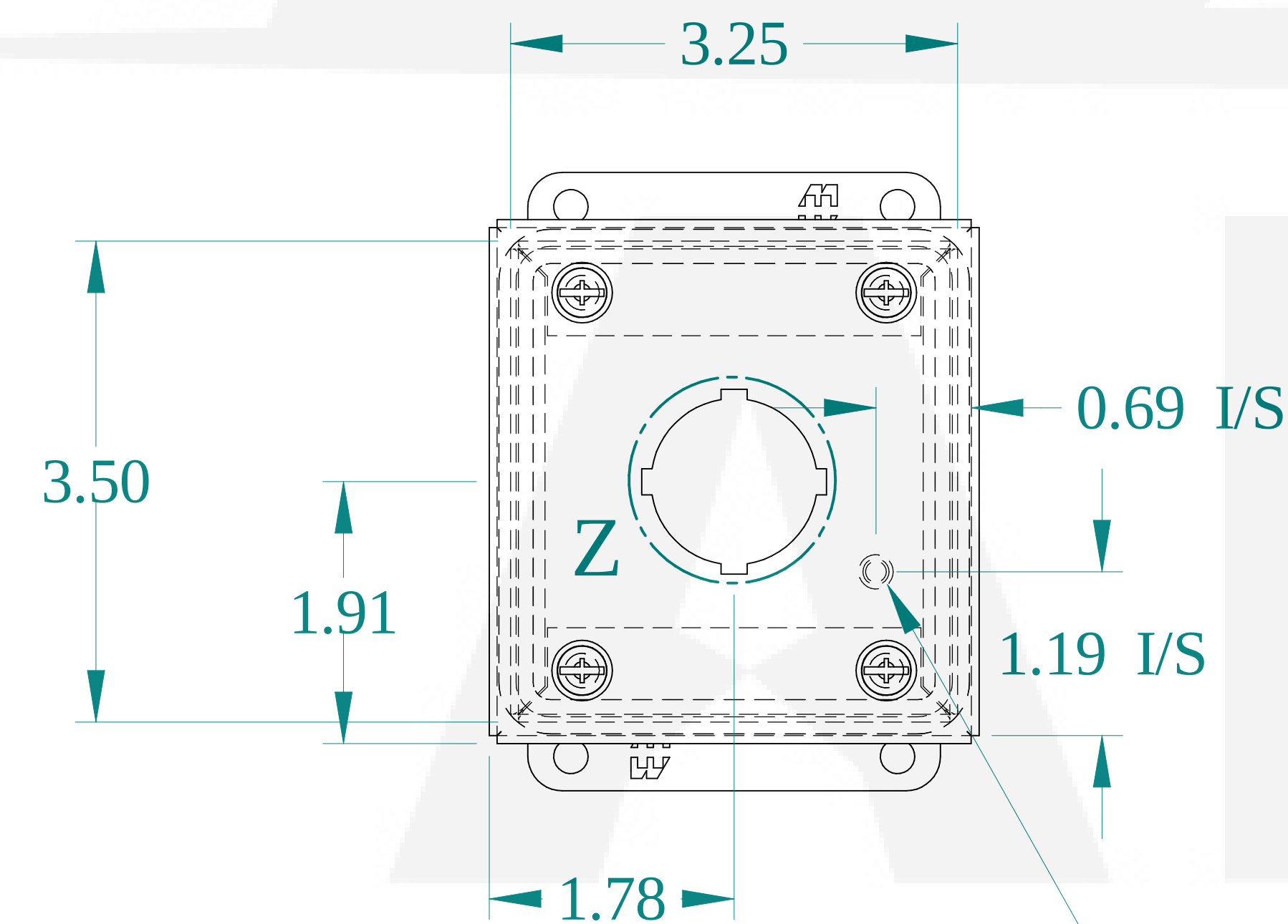
FRONT VIEW
