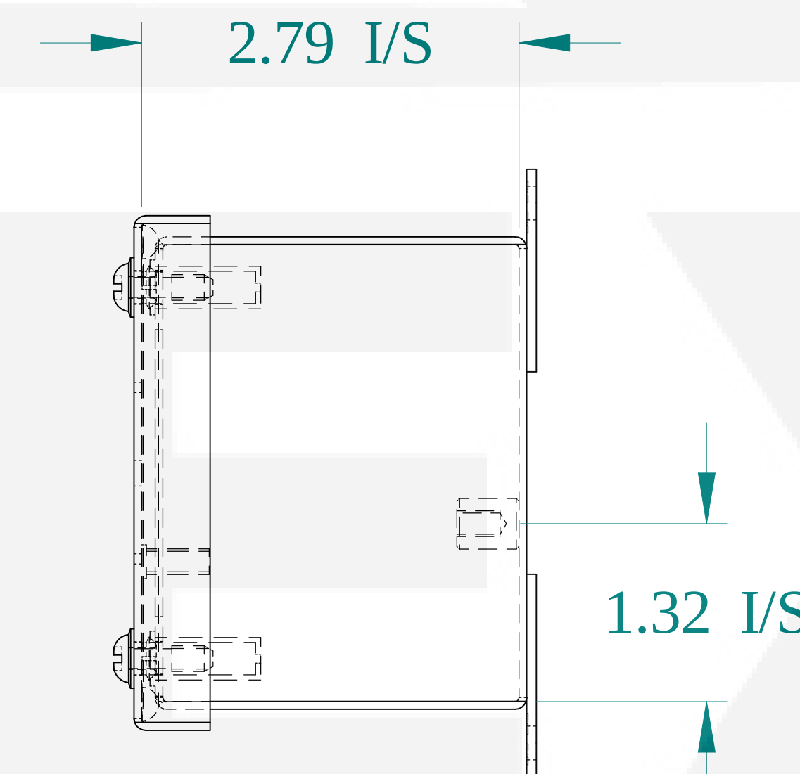
SIDE VIEW
