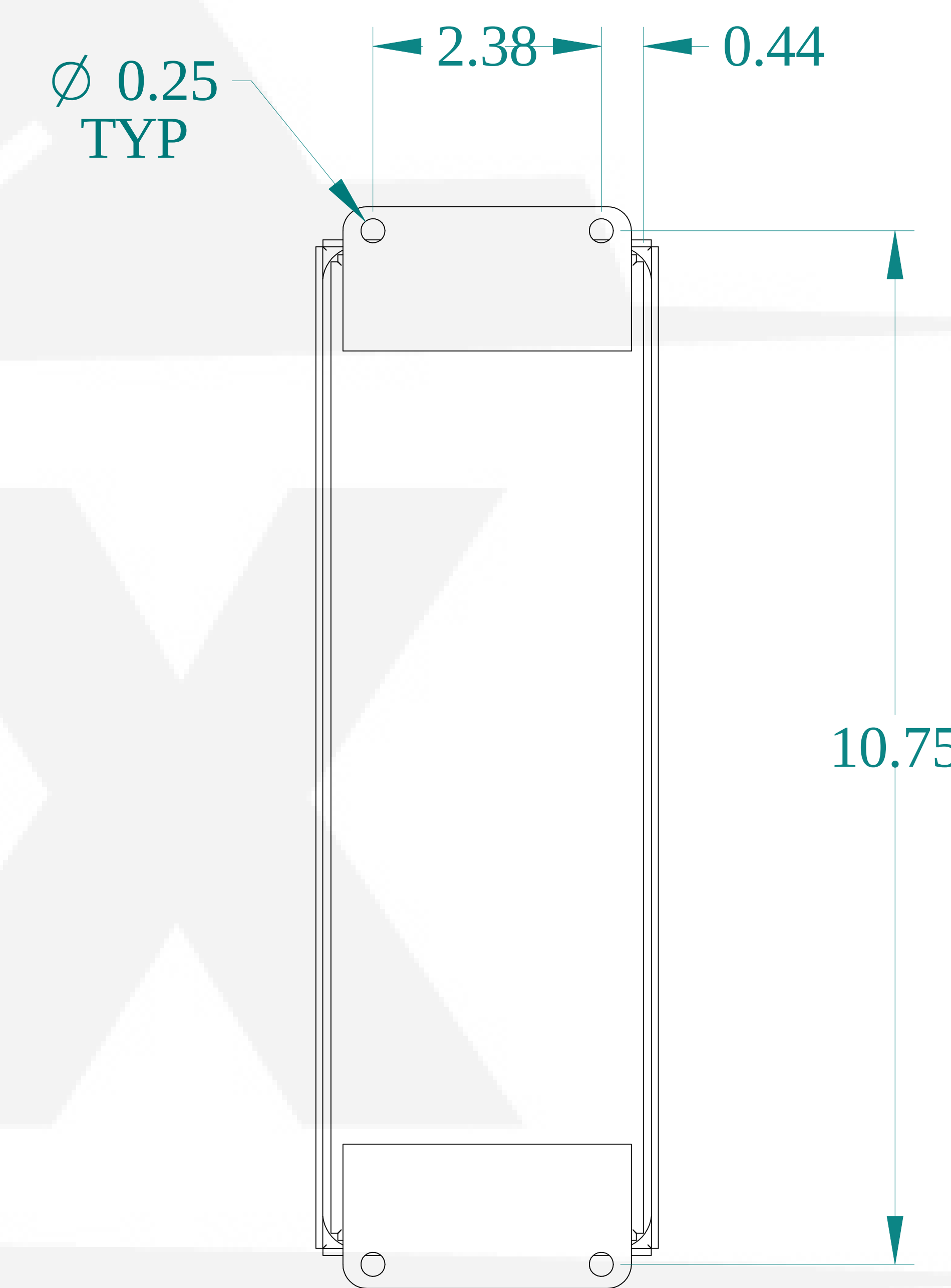
BACK VIEW
