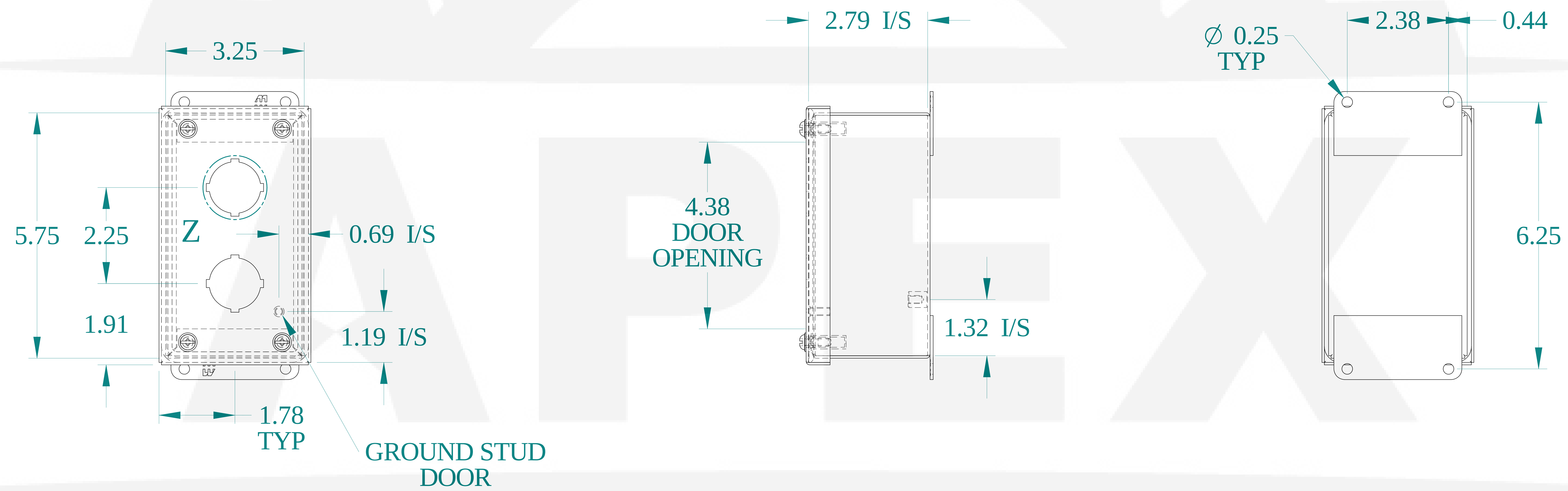
BACK VIEW
