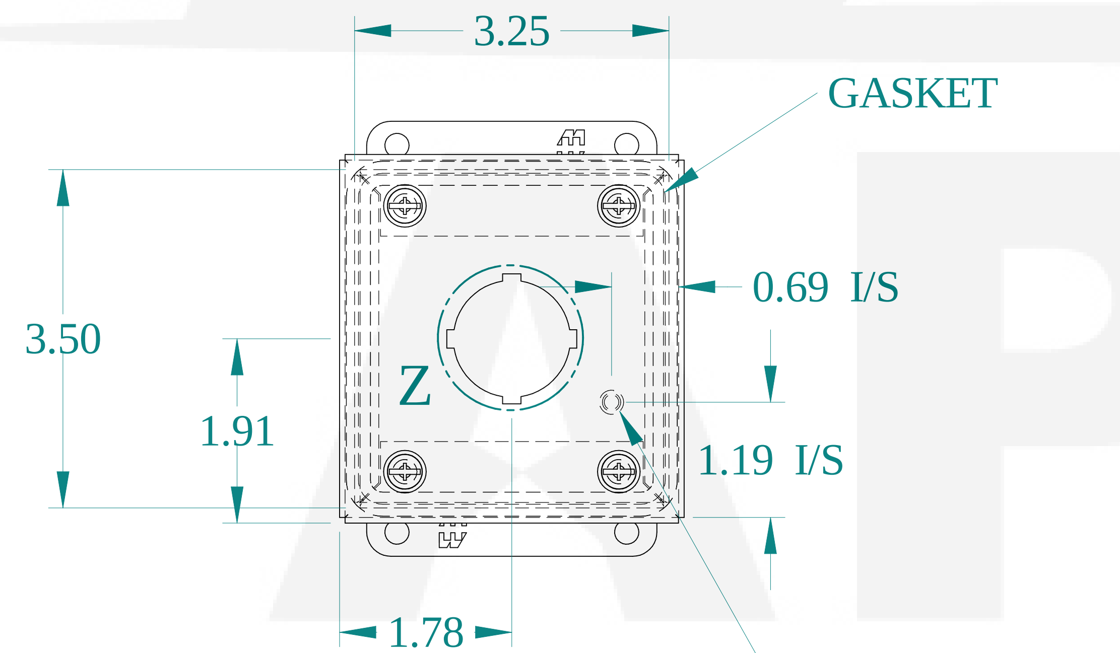
FRONT VIEW
