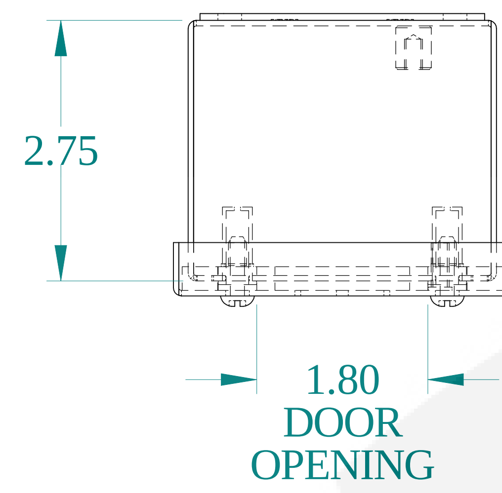
TOP VIEW
