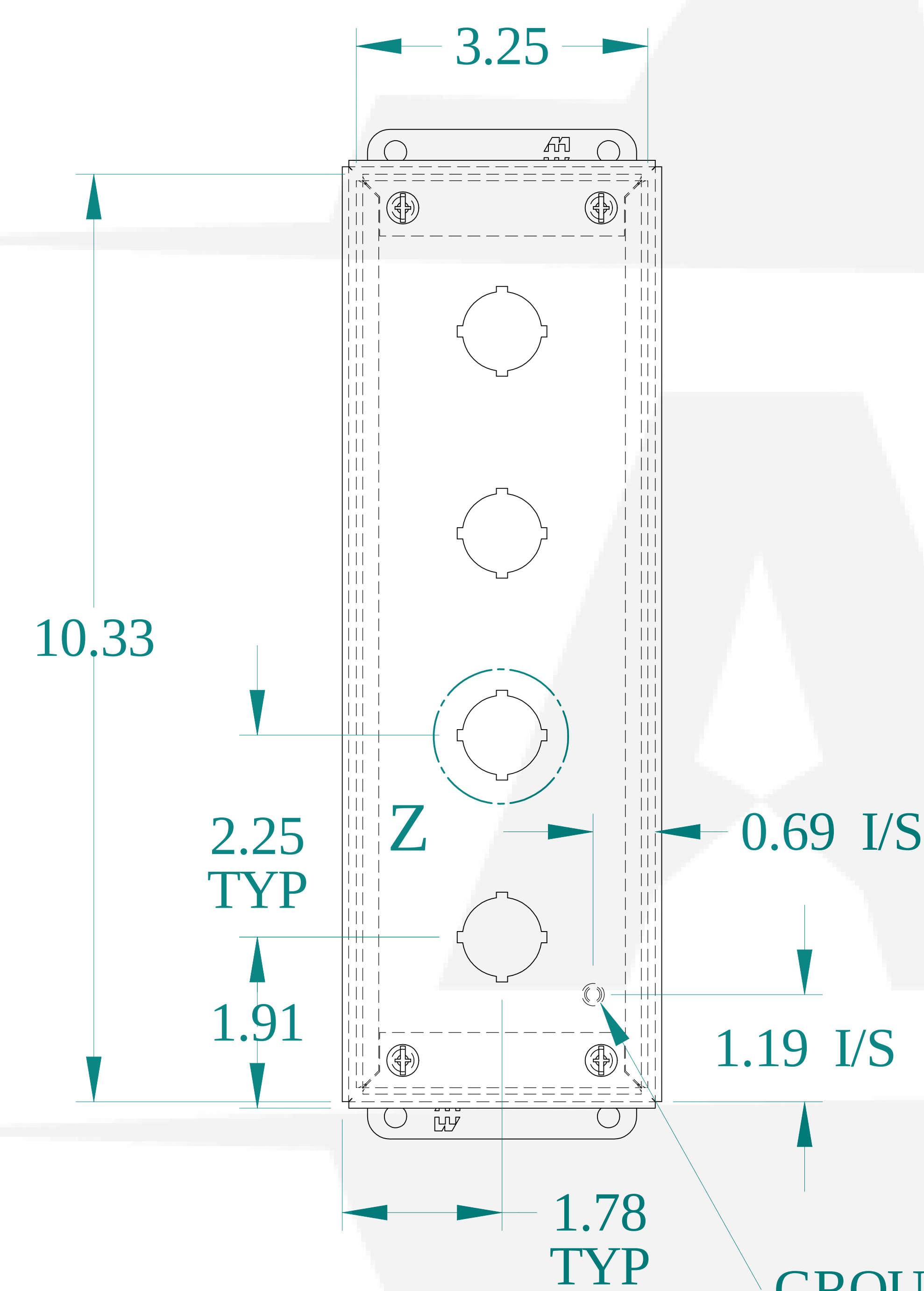
FRONT VIEW
