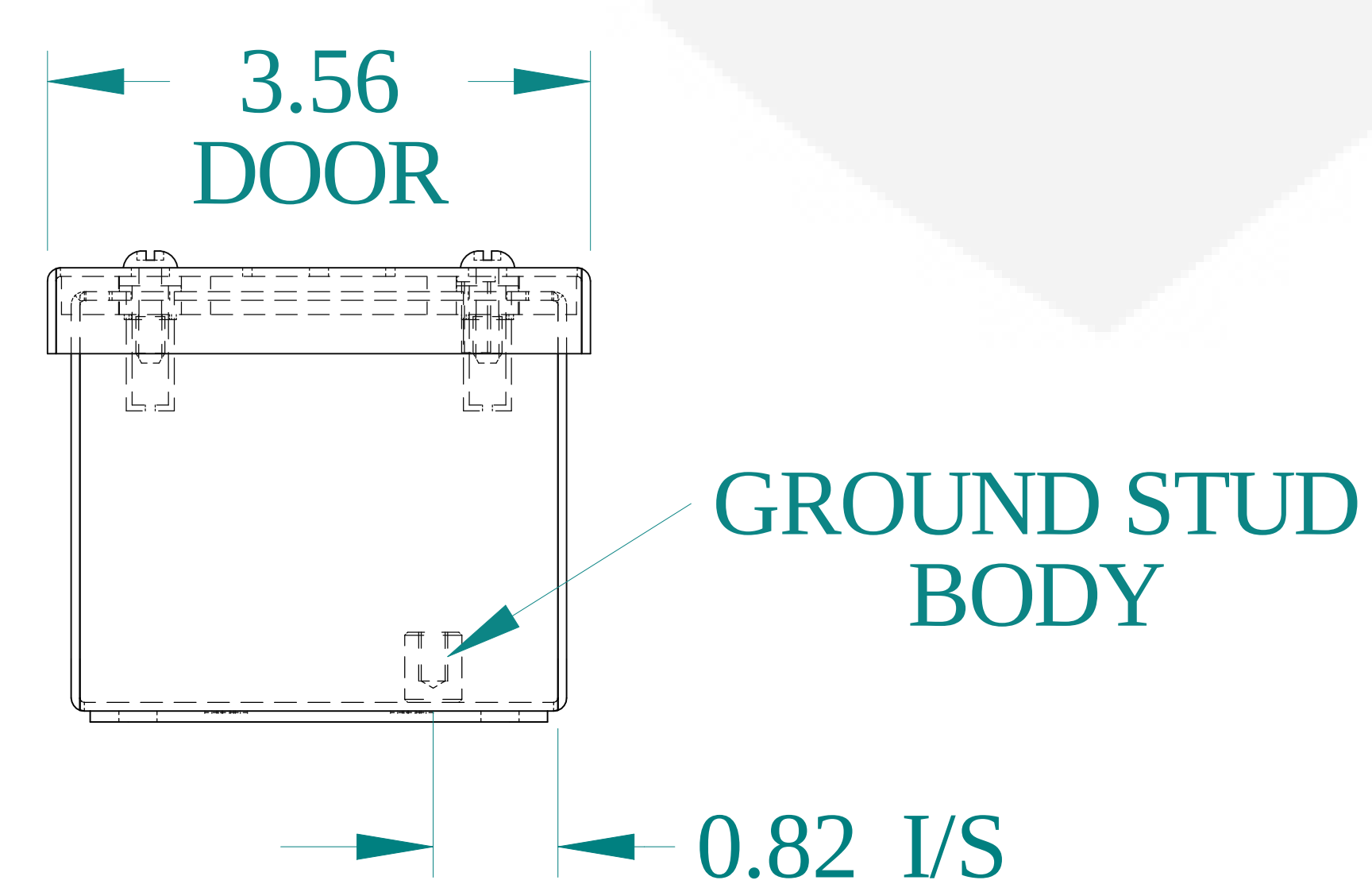
BOTTOM VIEW
