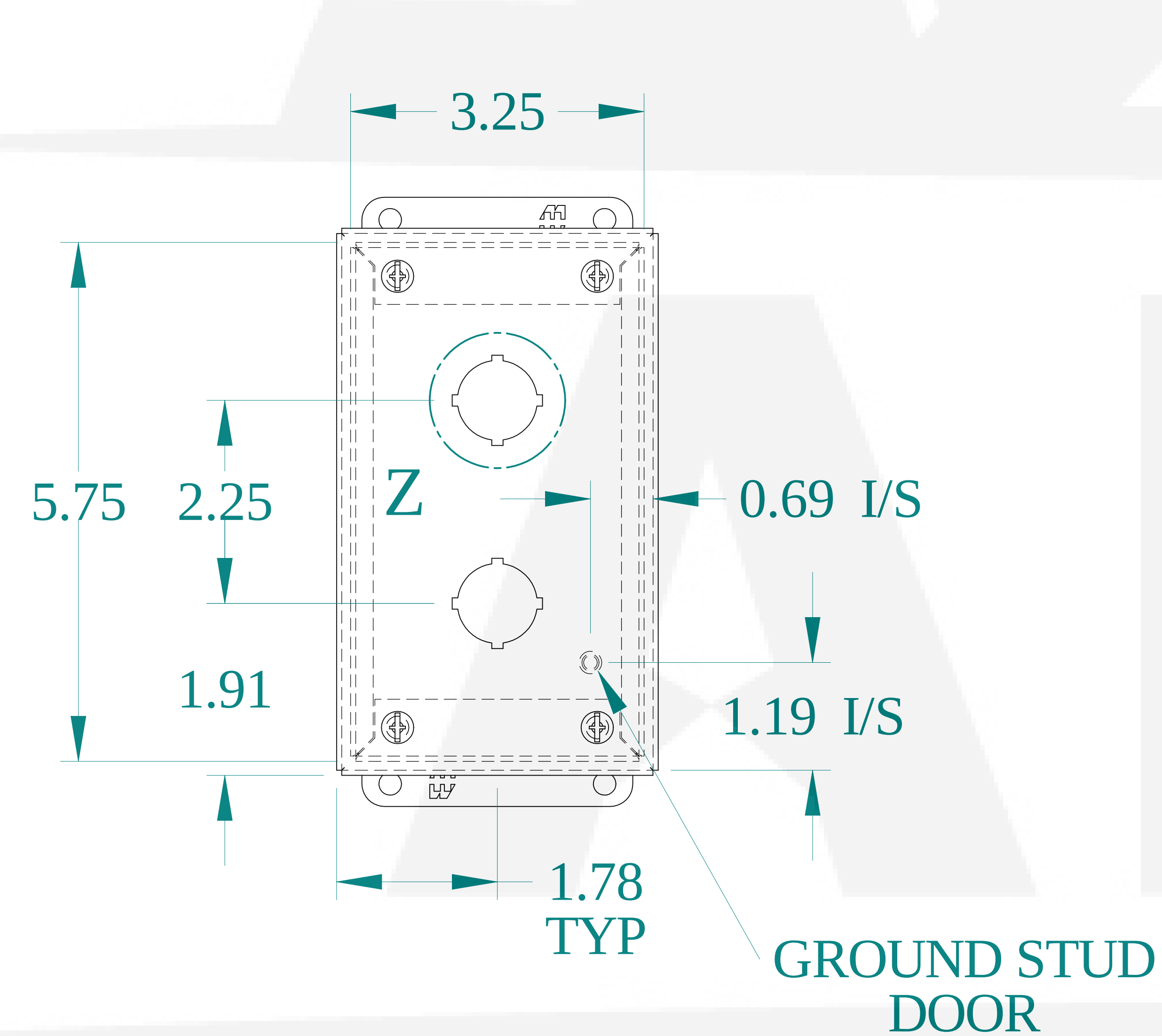
FRONT VIEW
