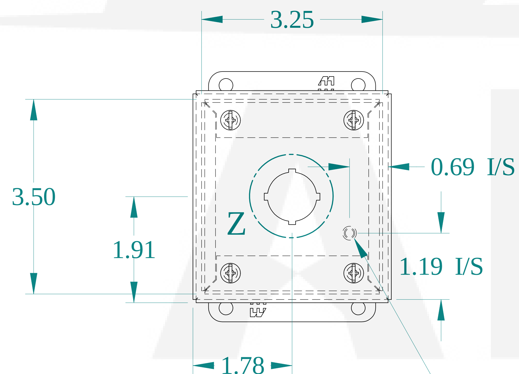
FRONT VIEW
