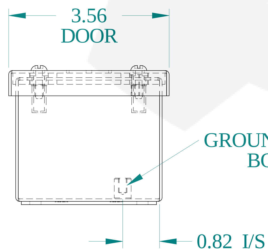
BOTTOM VIEW
