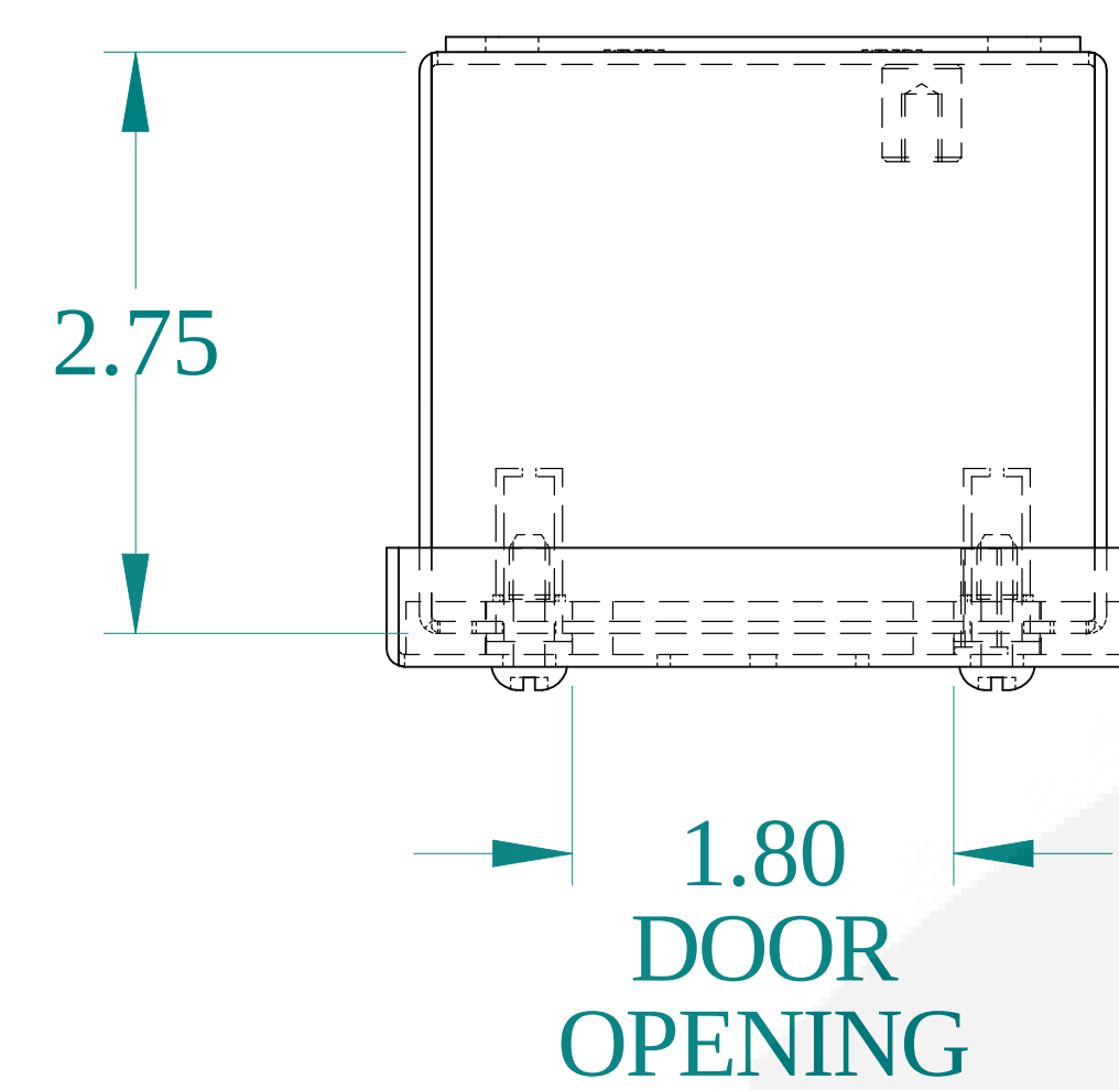
TOP VIEW
