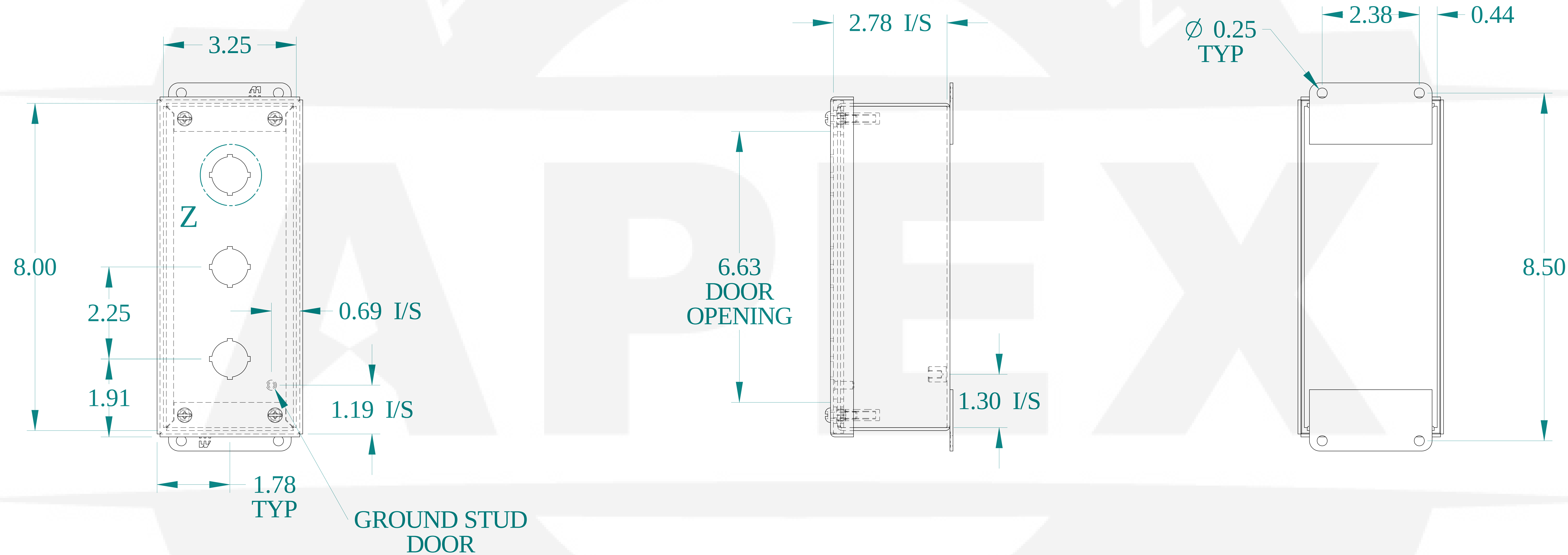
SIDE VIEW
