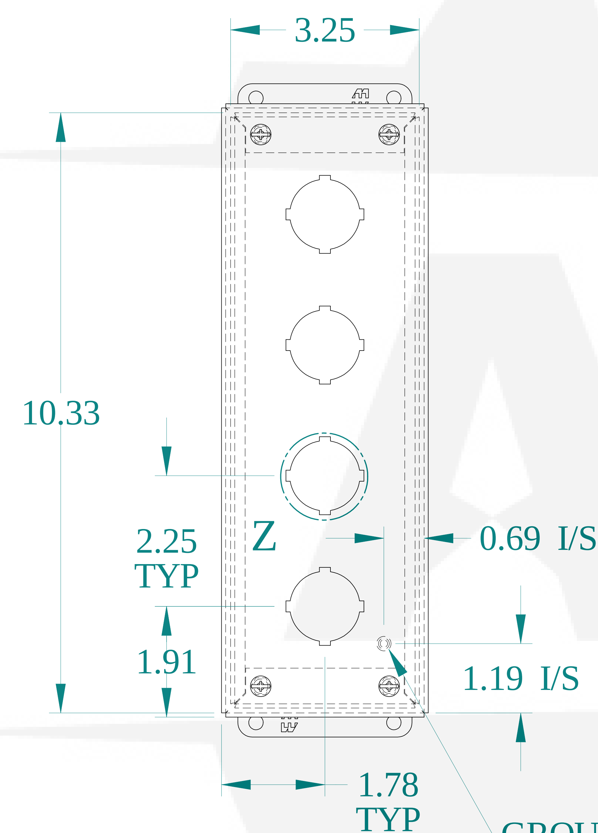
FRONT VIEW
