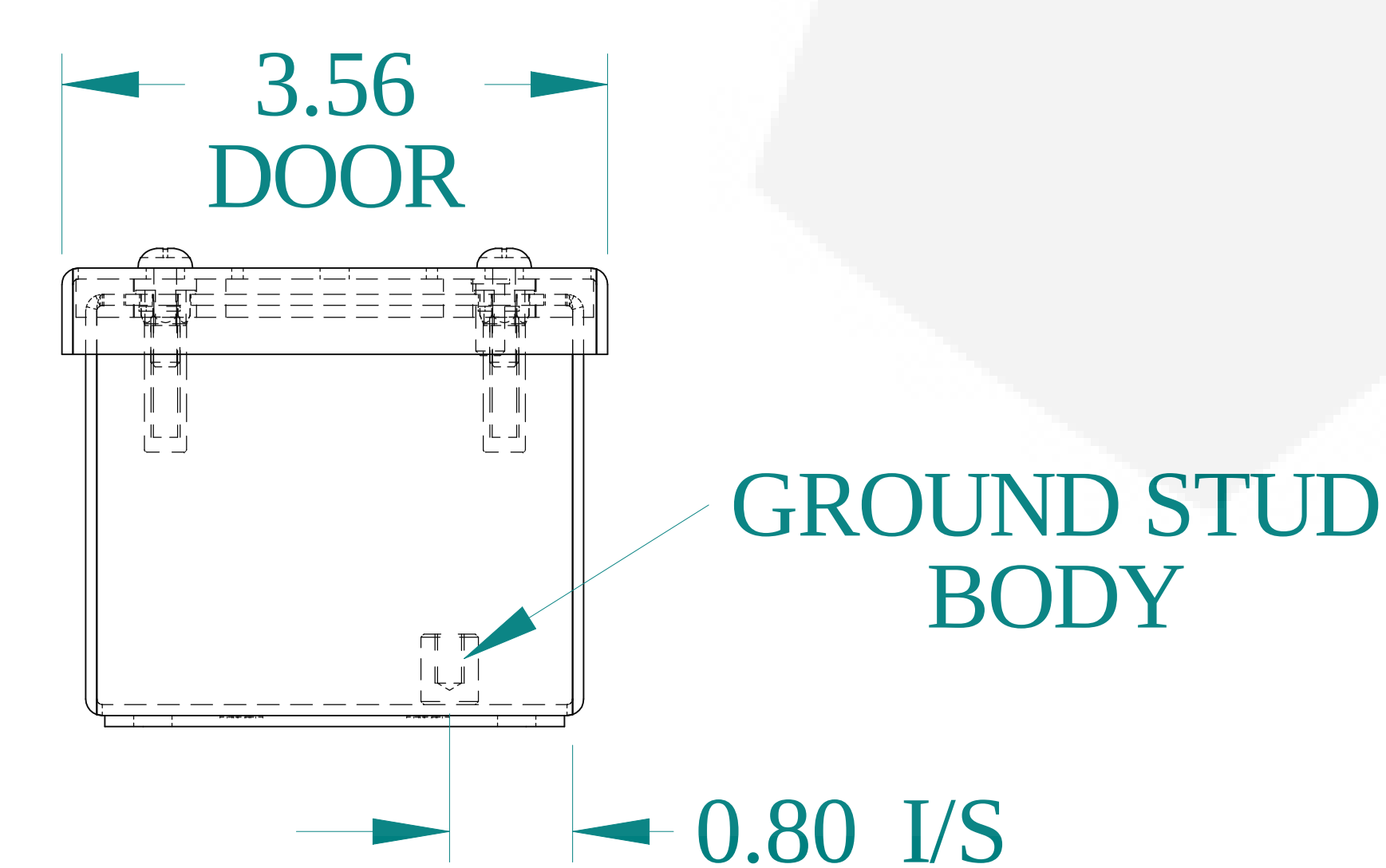
BOTTOM VIEW
