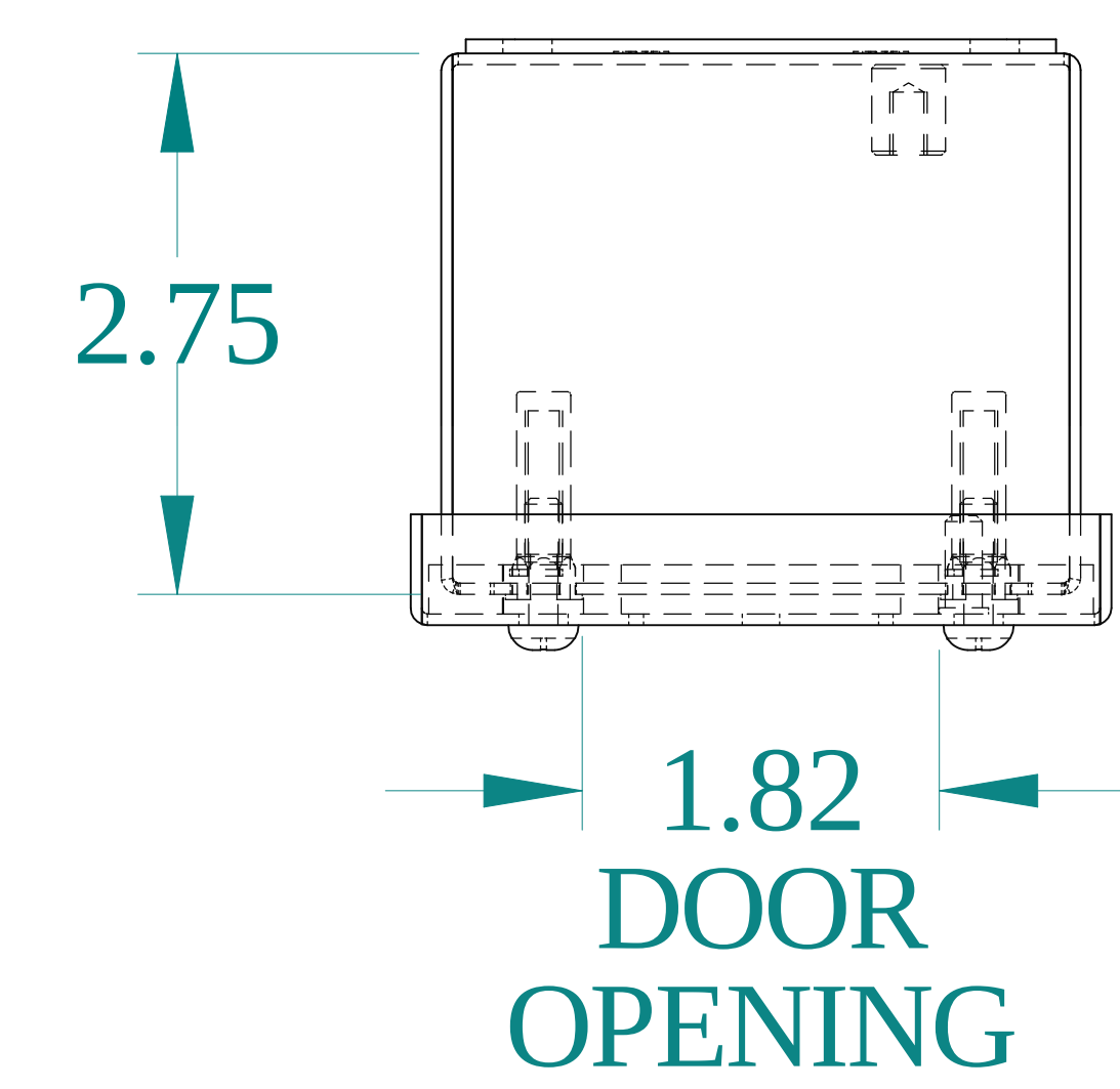
TOP VIEW
