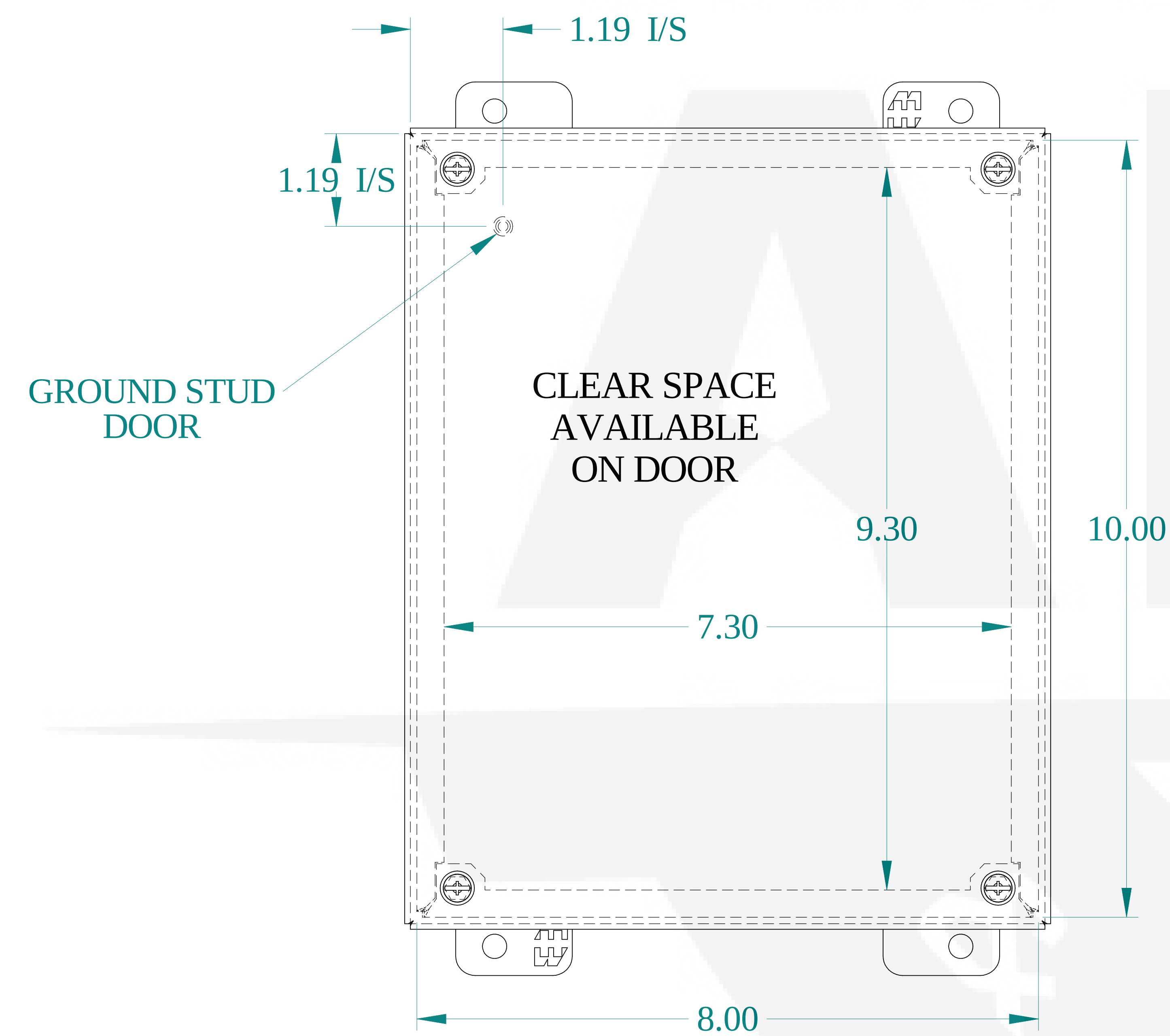
FRONT VIEW
