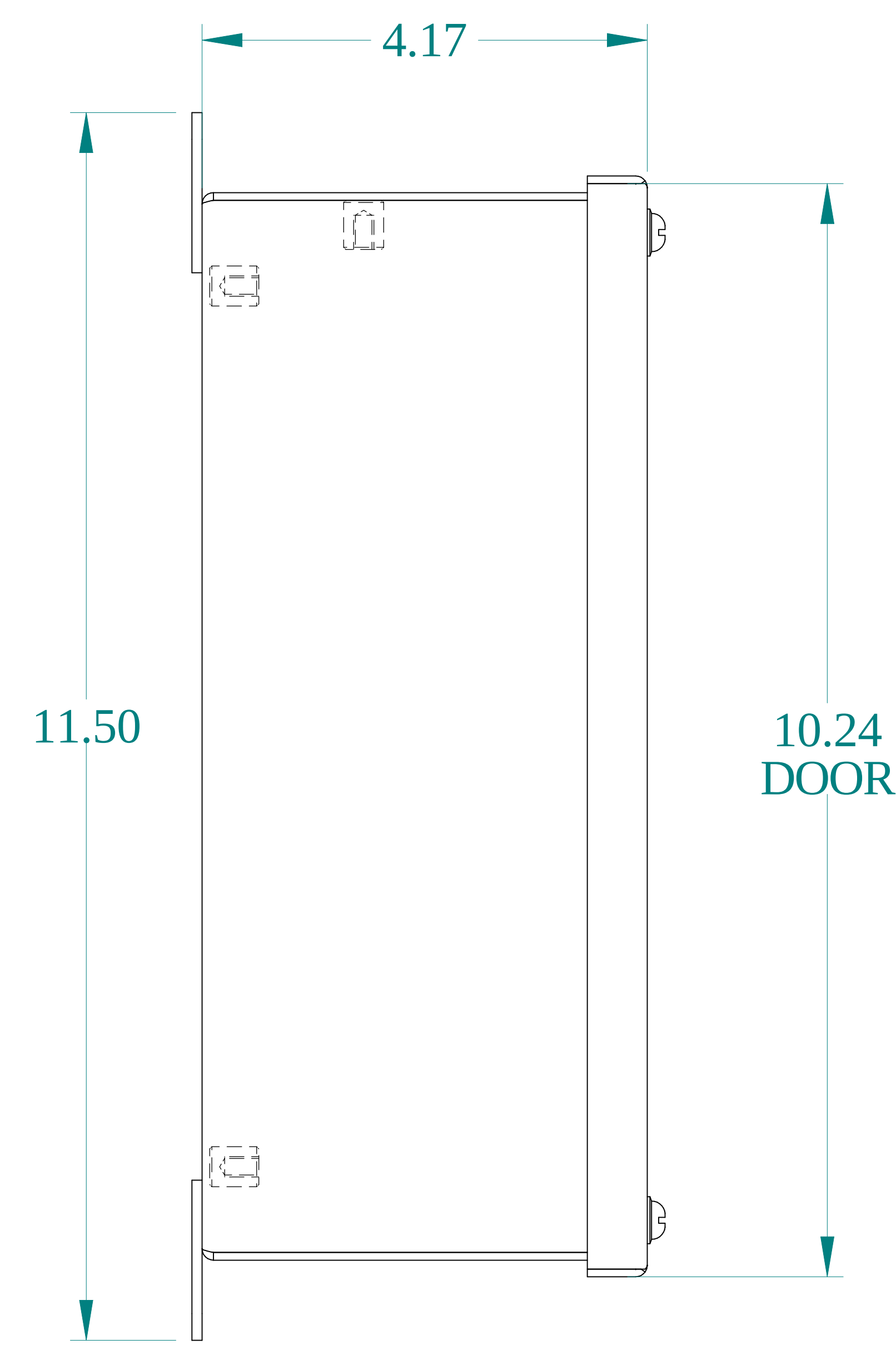
SIDE VIEW
