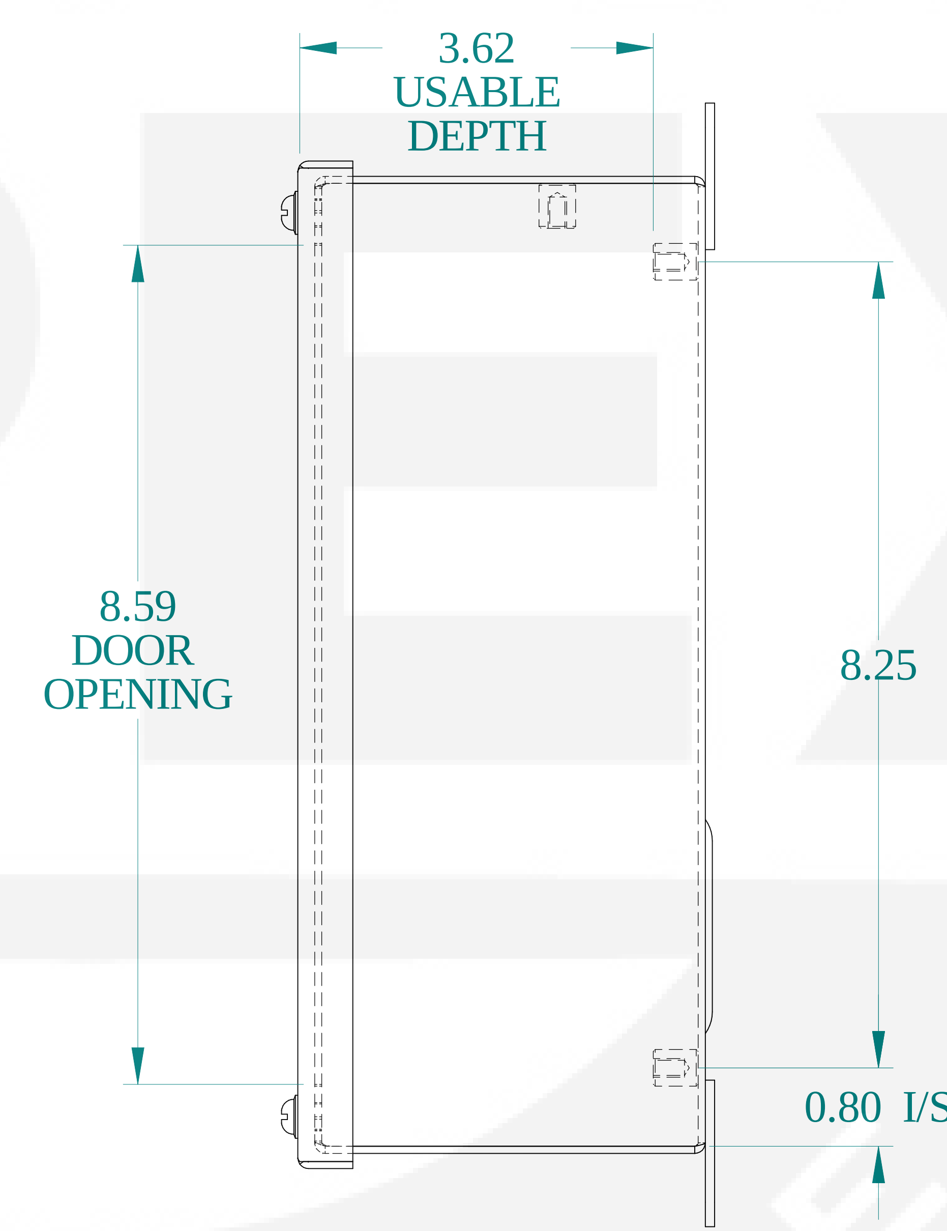
SIDE VIEW
