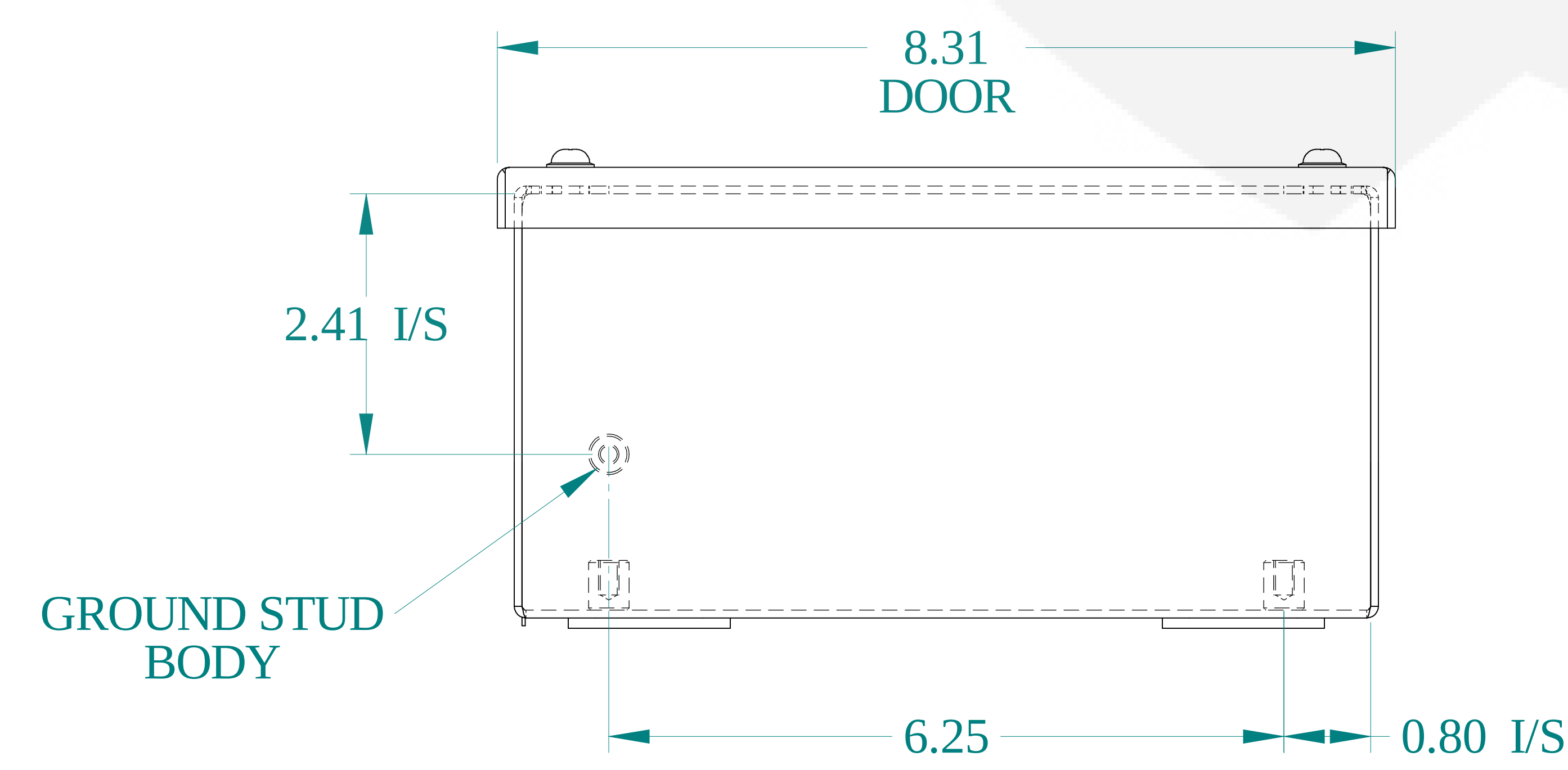
BOTTOM VIEW
