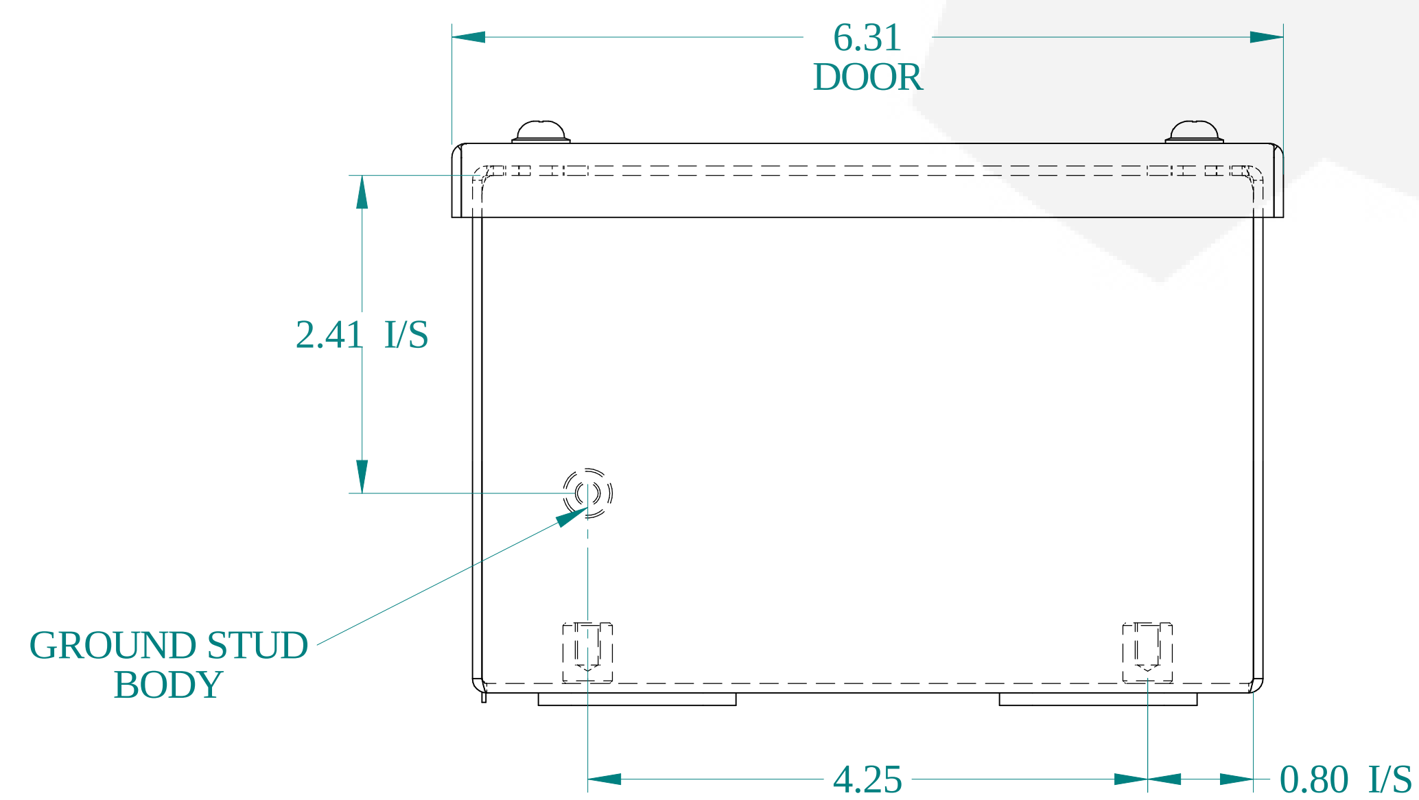
BOTTOM VIEW
