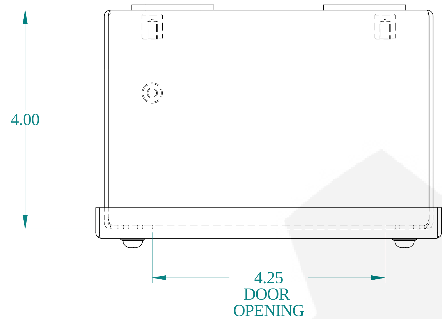
TOP VIEW
