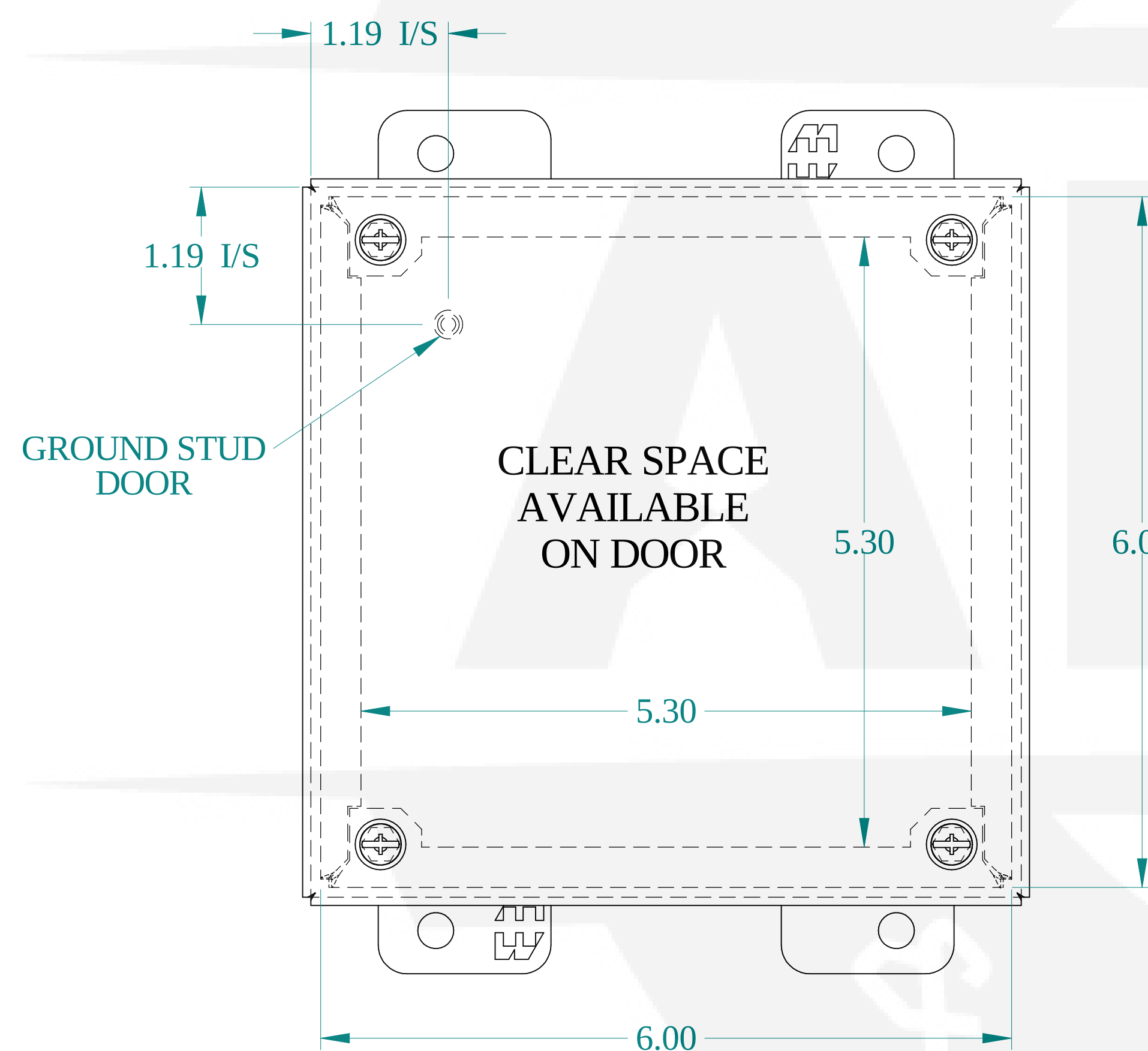
FRONT VIEW
