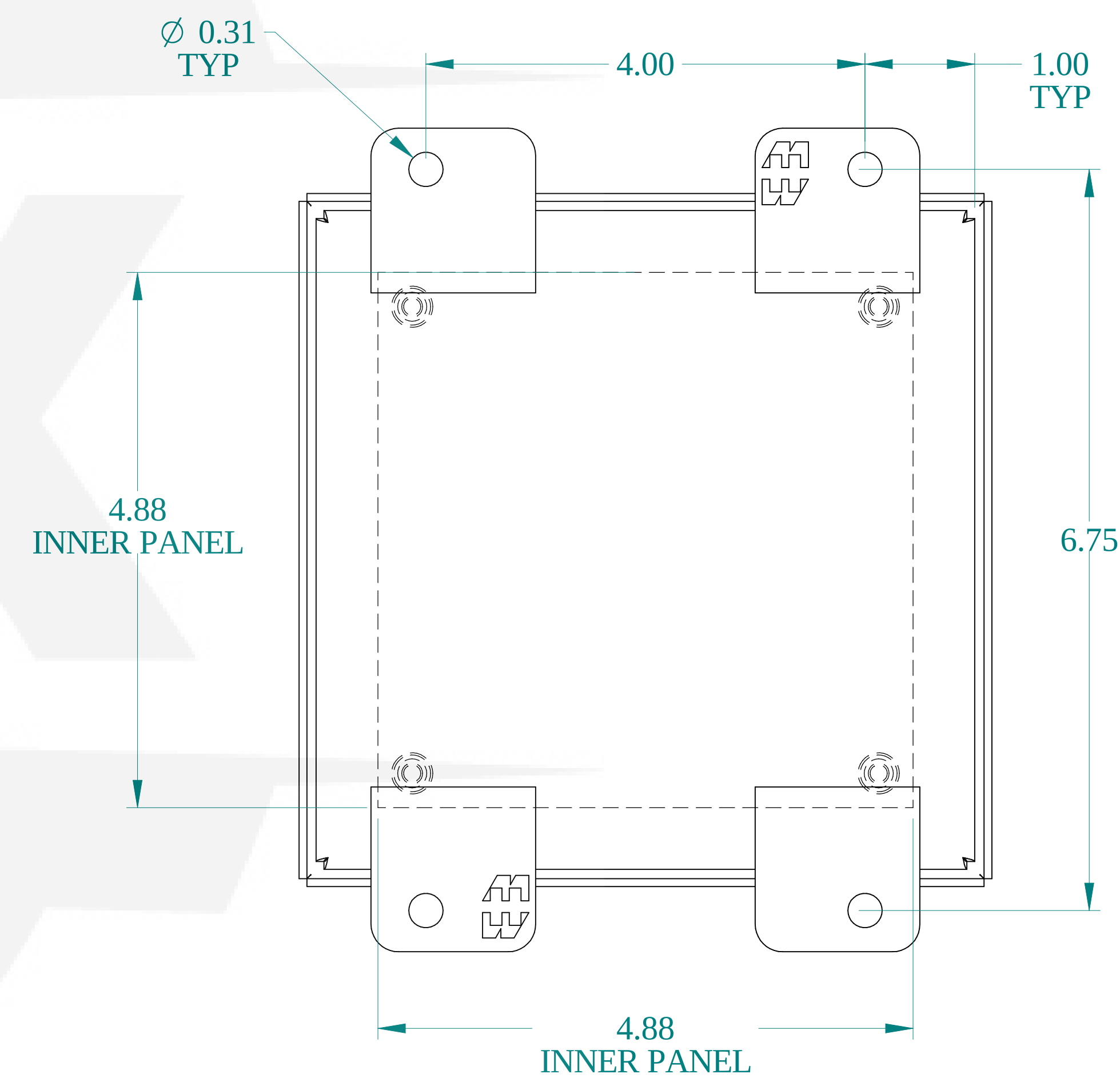
BACK VIEW
