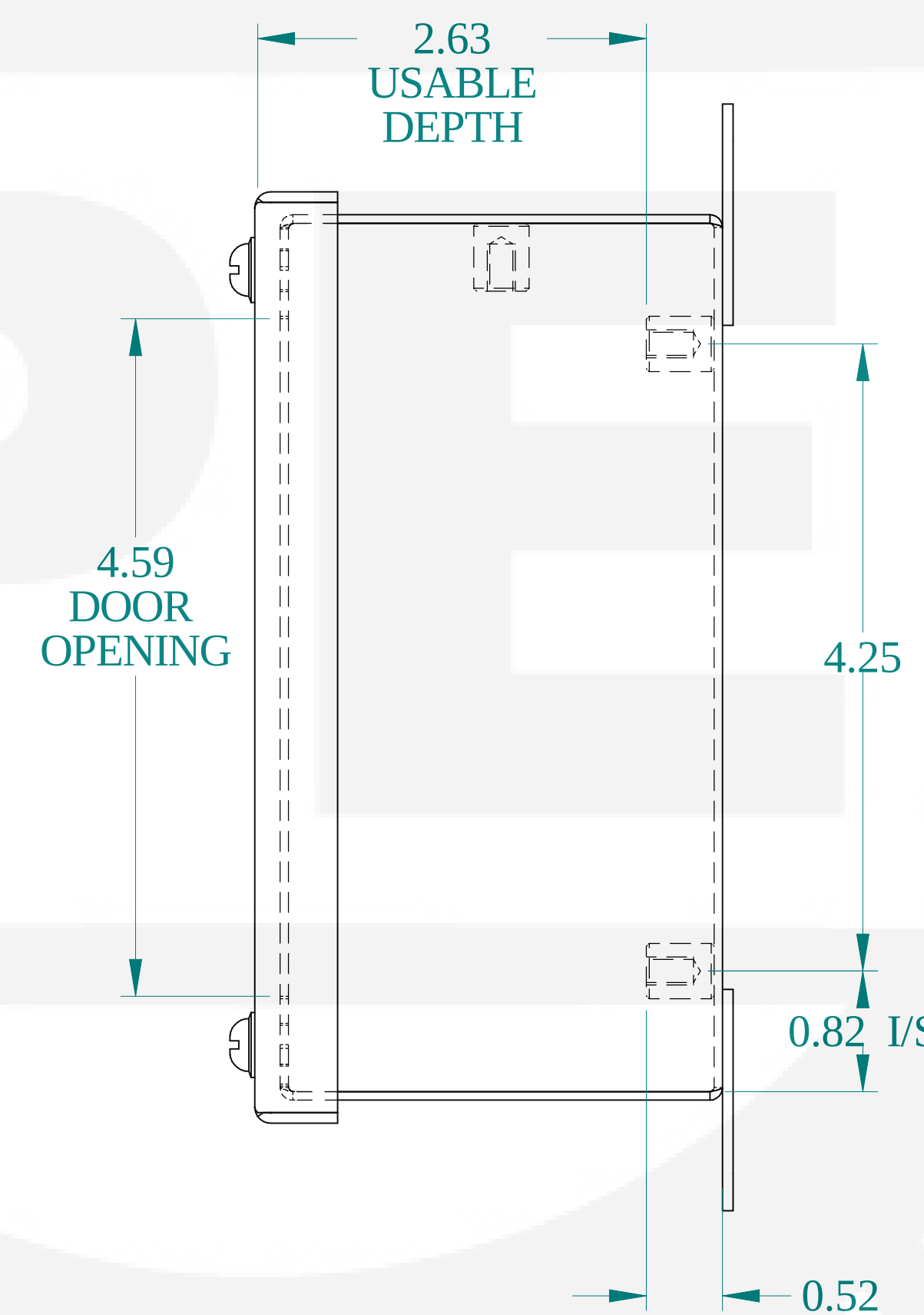
SIDE VIEW
