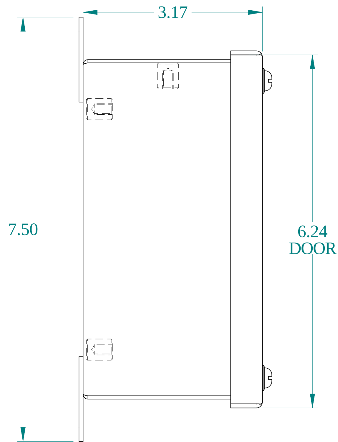
SIDE VIEW
