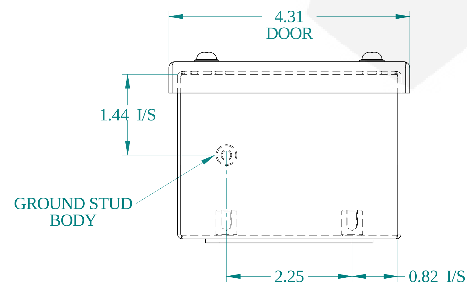
BOTTOM VIEW
