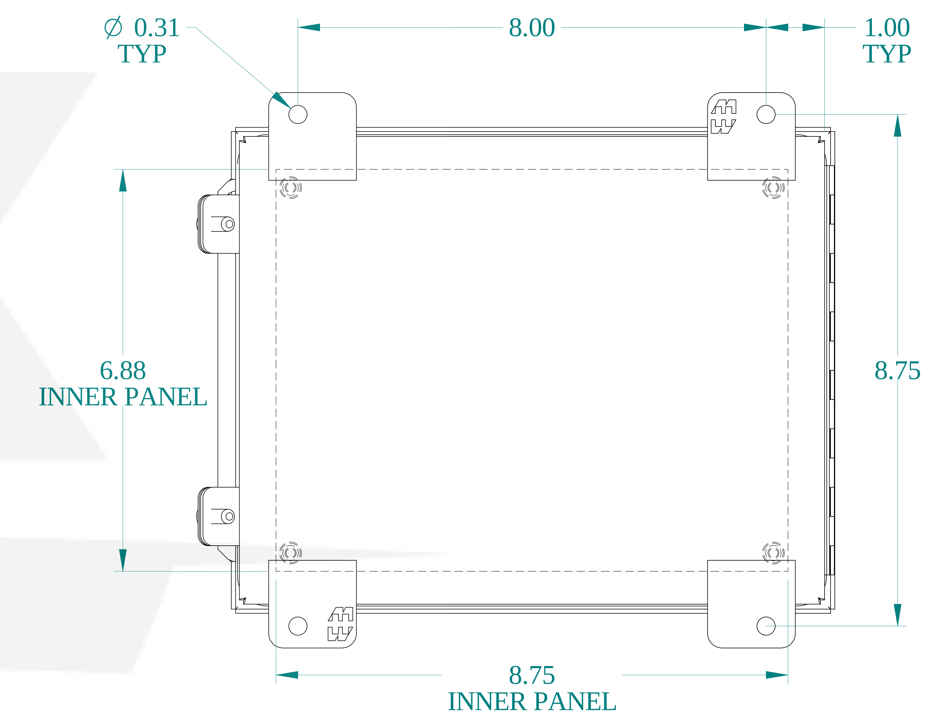
BACK VIEW
