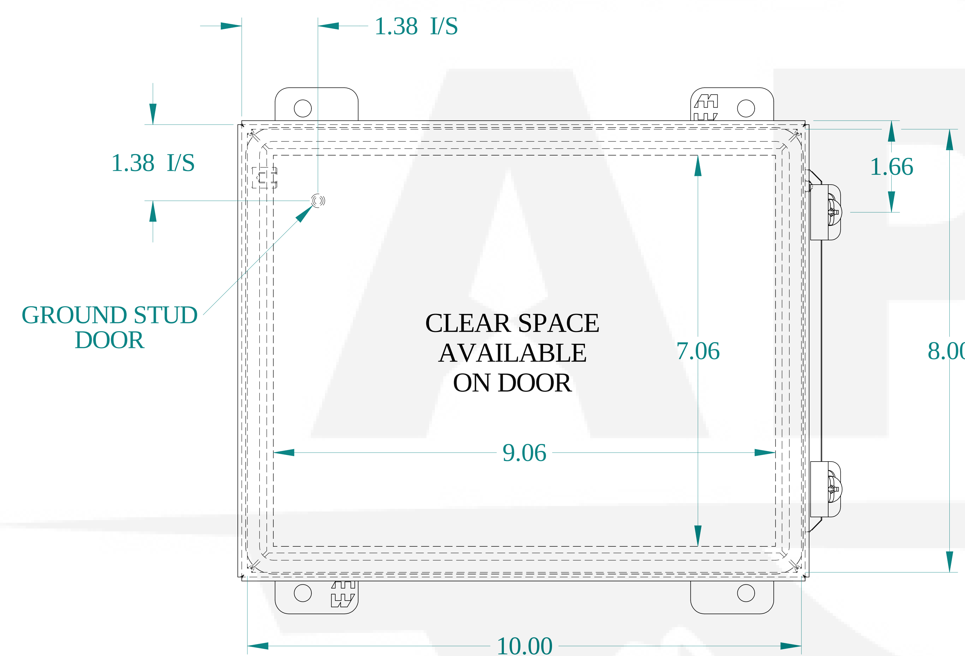
FRONT VIEW
