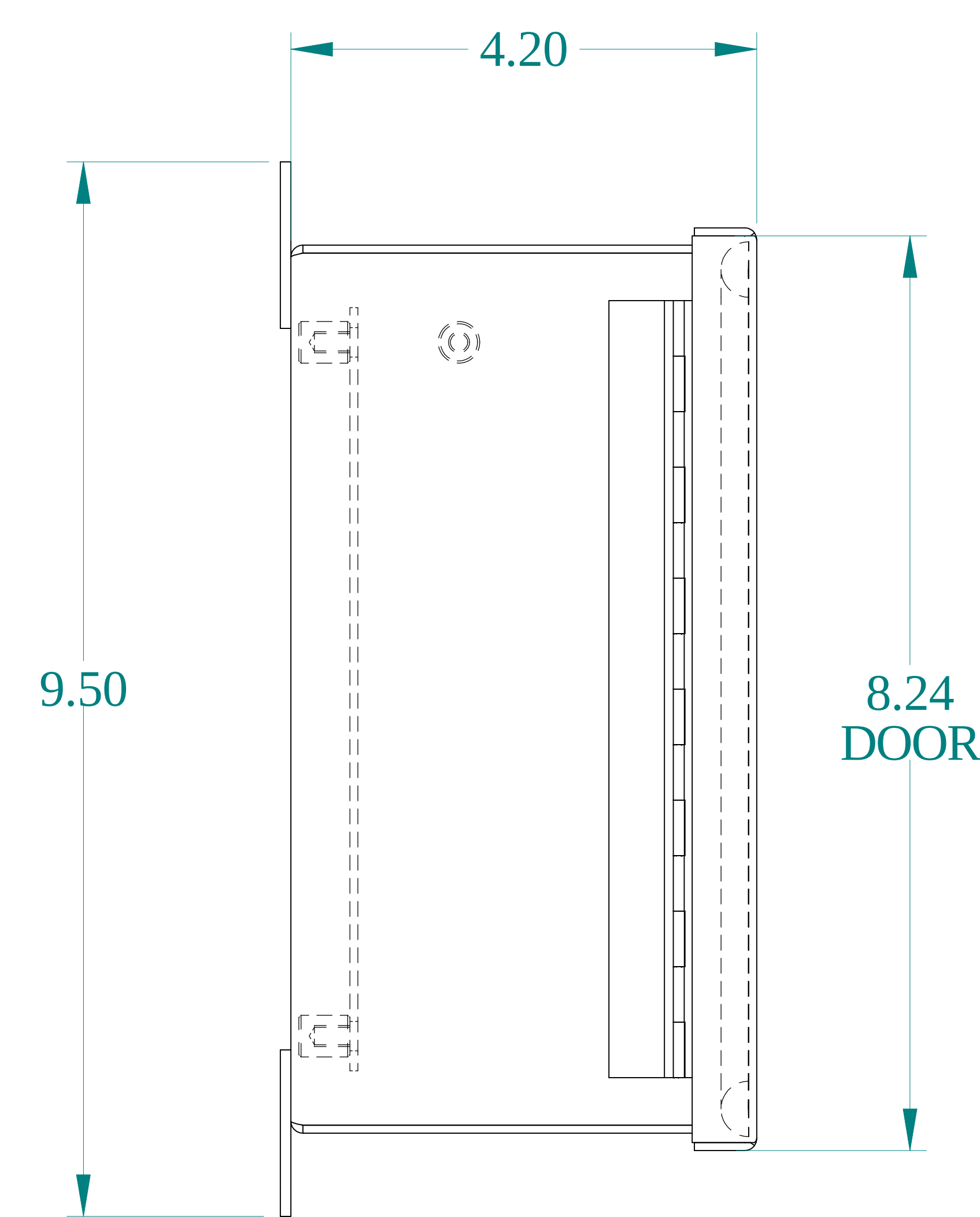
SIDE VIEW
