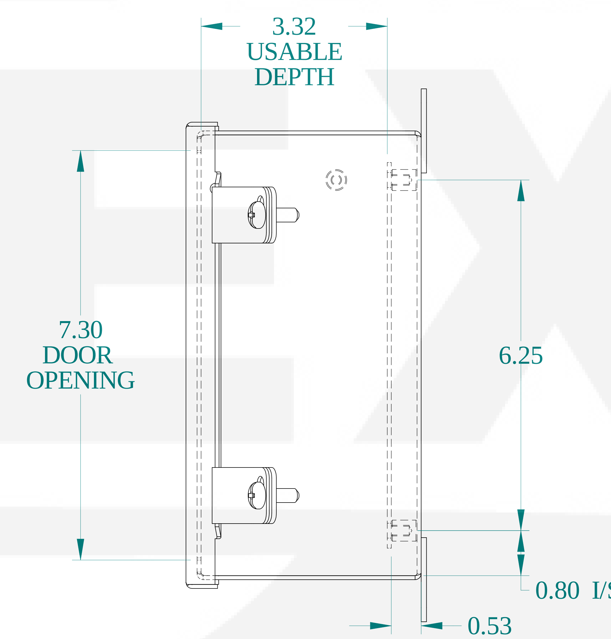
SIDE VIEW
