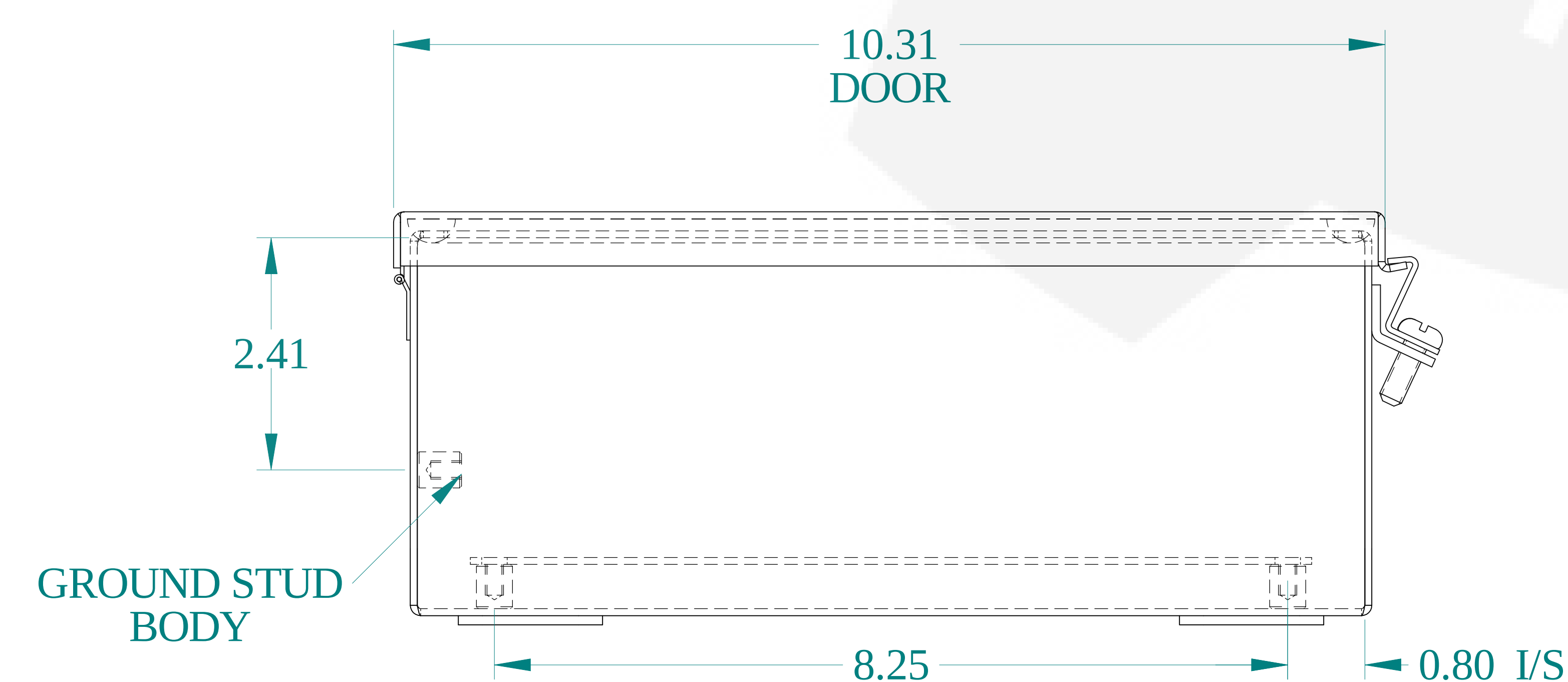
BOTTOM VIEW
